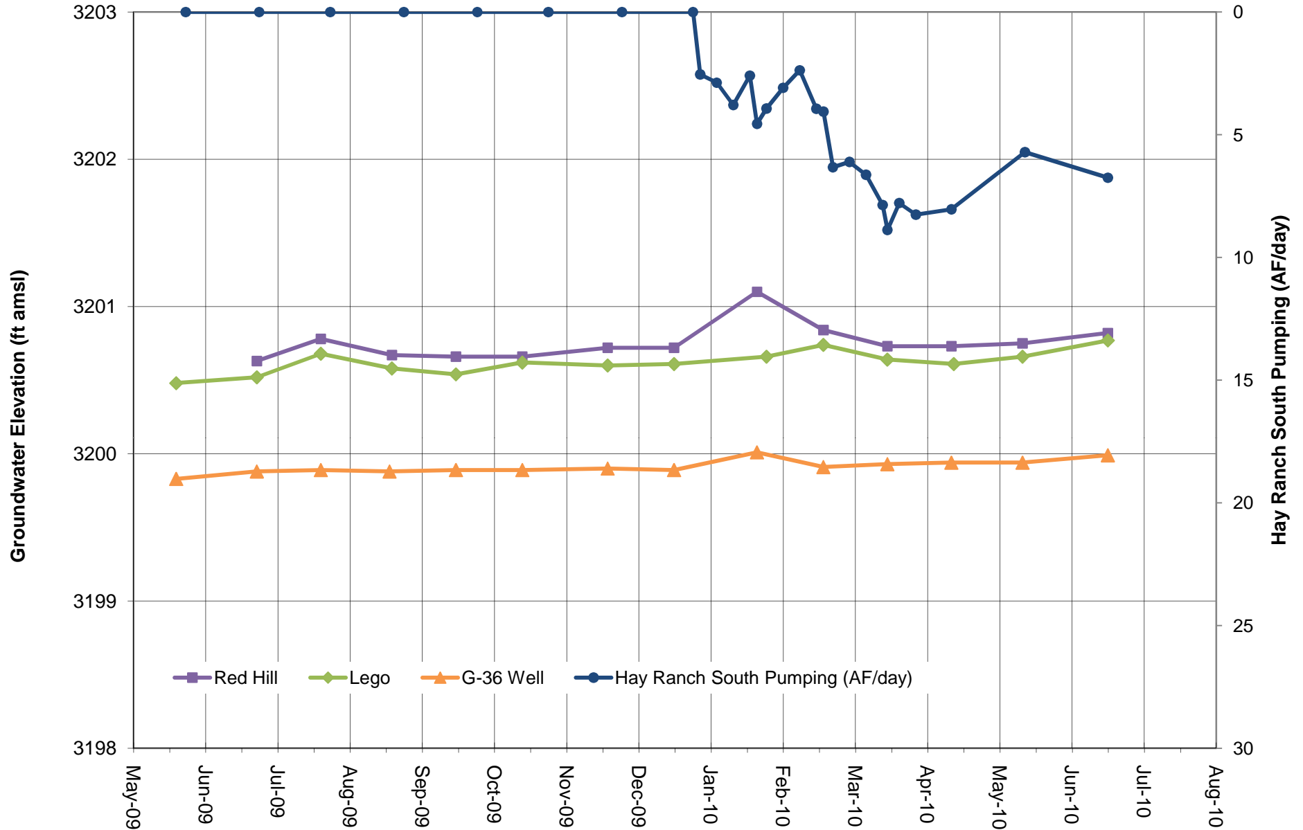
FIGURE 8 GROUNDWATER ELEVATION and HR SOUTH PUMPING: Red Hill, Lego and G-36
