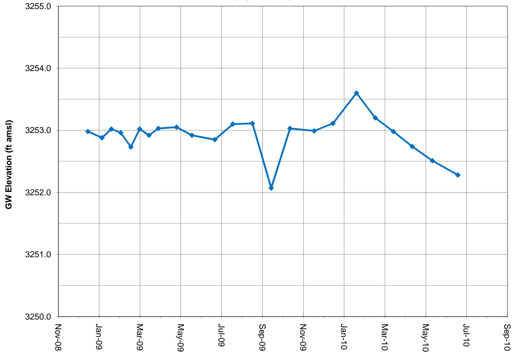
FIGURE 1 GROUNDWATER ELEVATION DATA - Long-Term (Manual) RV040 - Dunmovin Well
