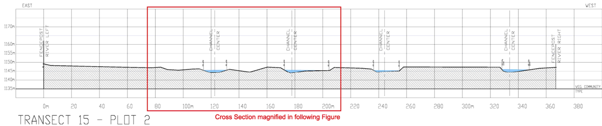
Channel Cross Section at Plot 2 Transect 15 Baseflow 45 cfs
