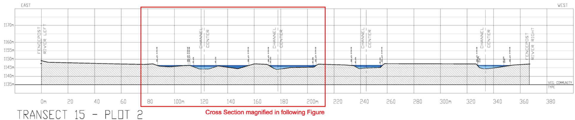
Channel Cross Section at Plot 2 Transect 15 High flow 200 cfs
