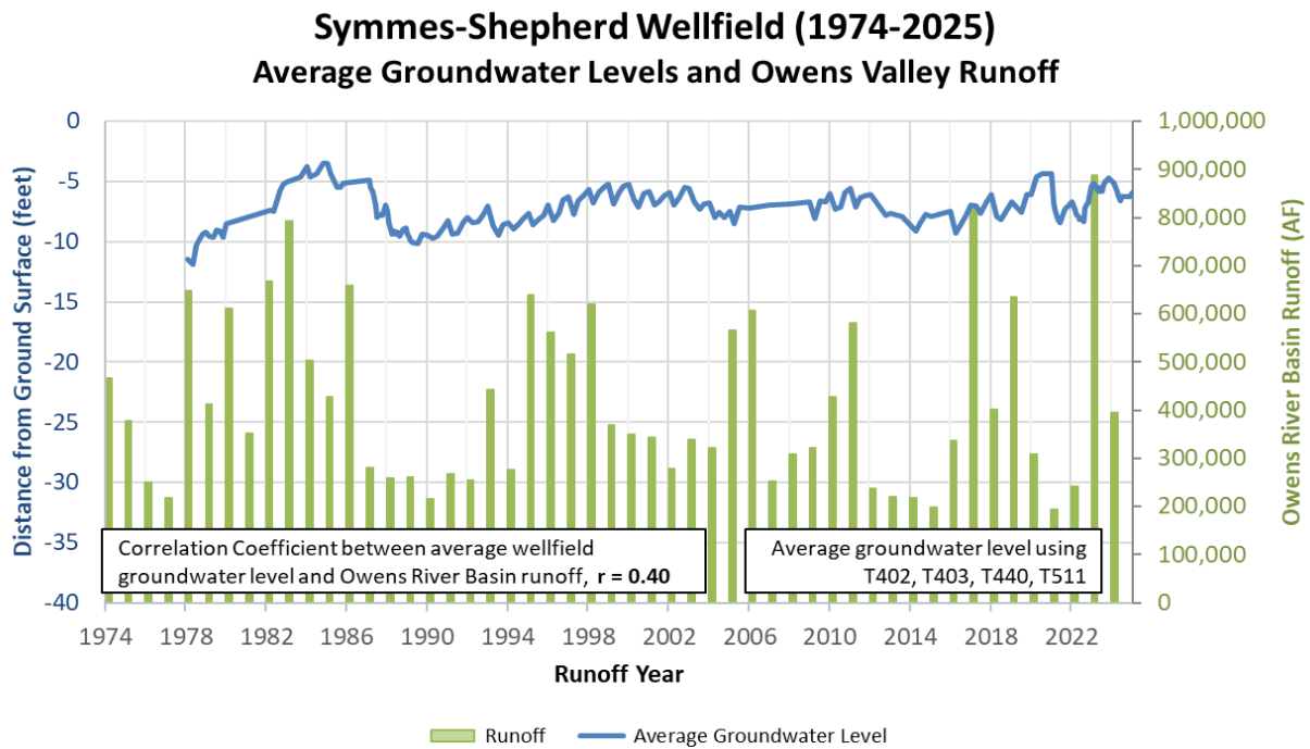
Figure 2.14. Average Symmes-Shepherd Wellfield Groundwater Level and Owens River Basin Runoff
