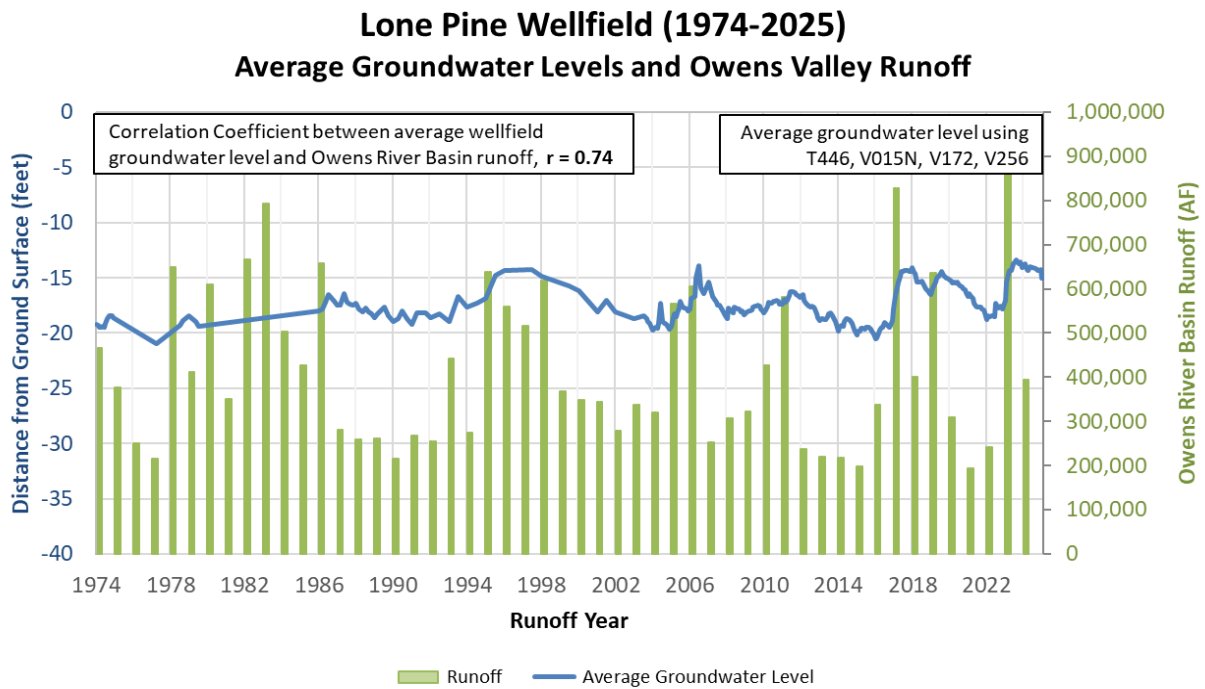
Figure 2.18. Average Lone Pine Wellfield Groundwater Level and Owens River Basin Runoff
