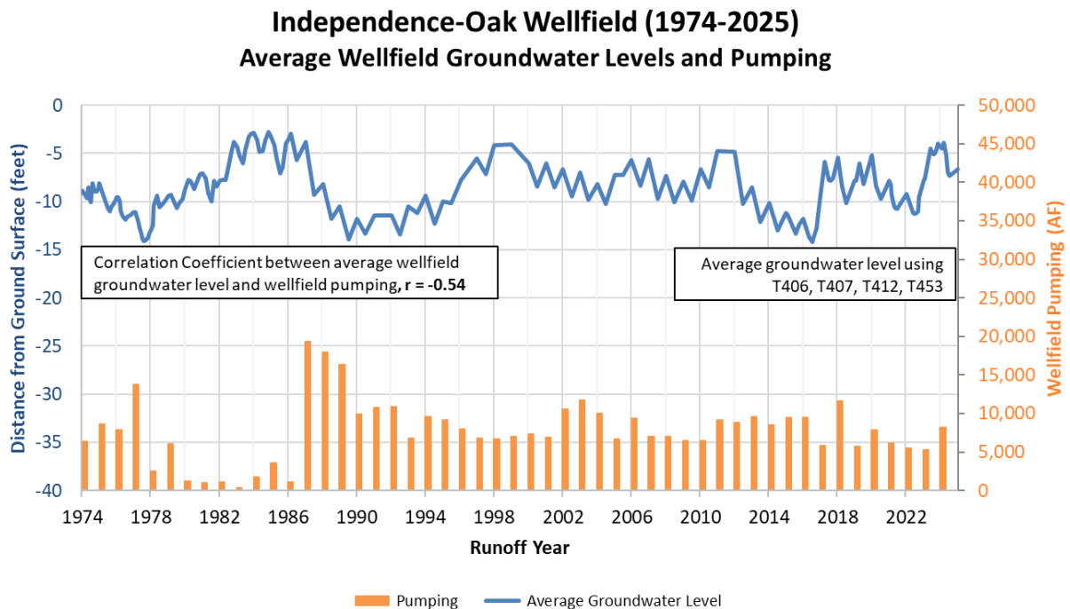
Figure 2.13. Average Independence-Oak Wellfield Groundwater Levels and Pumping
