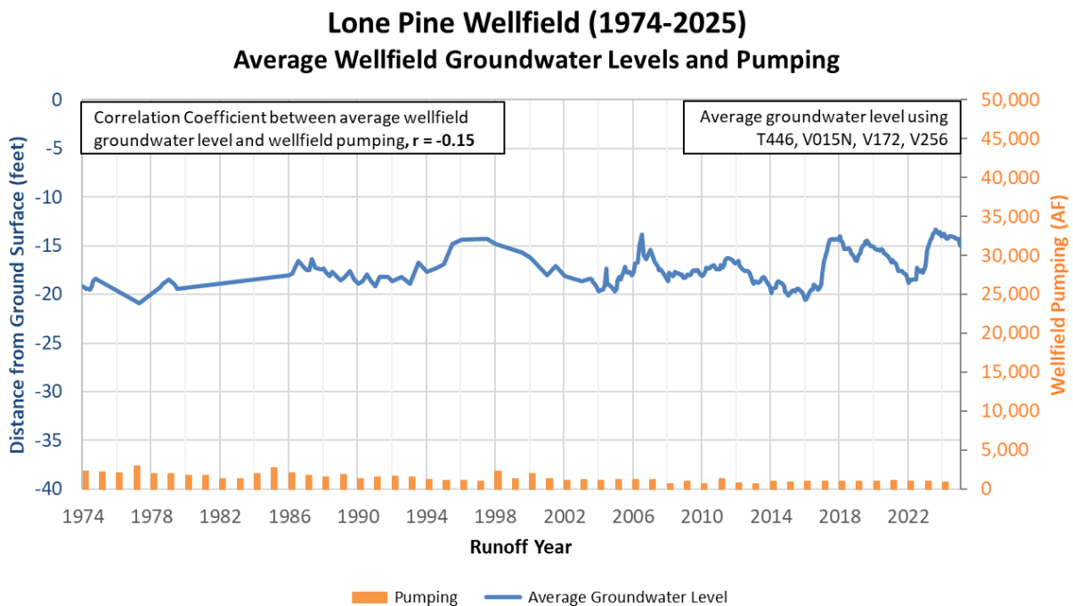
Figure 2.19. Average Lone Pine Wellfield Groundwater Levels and Pumping
