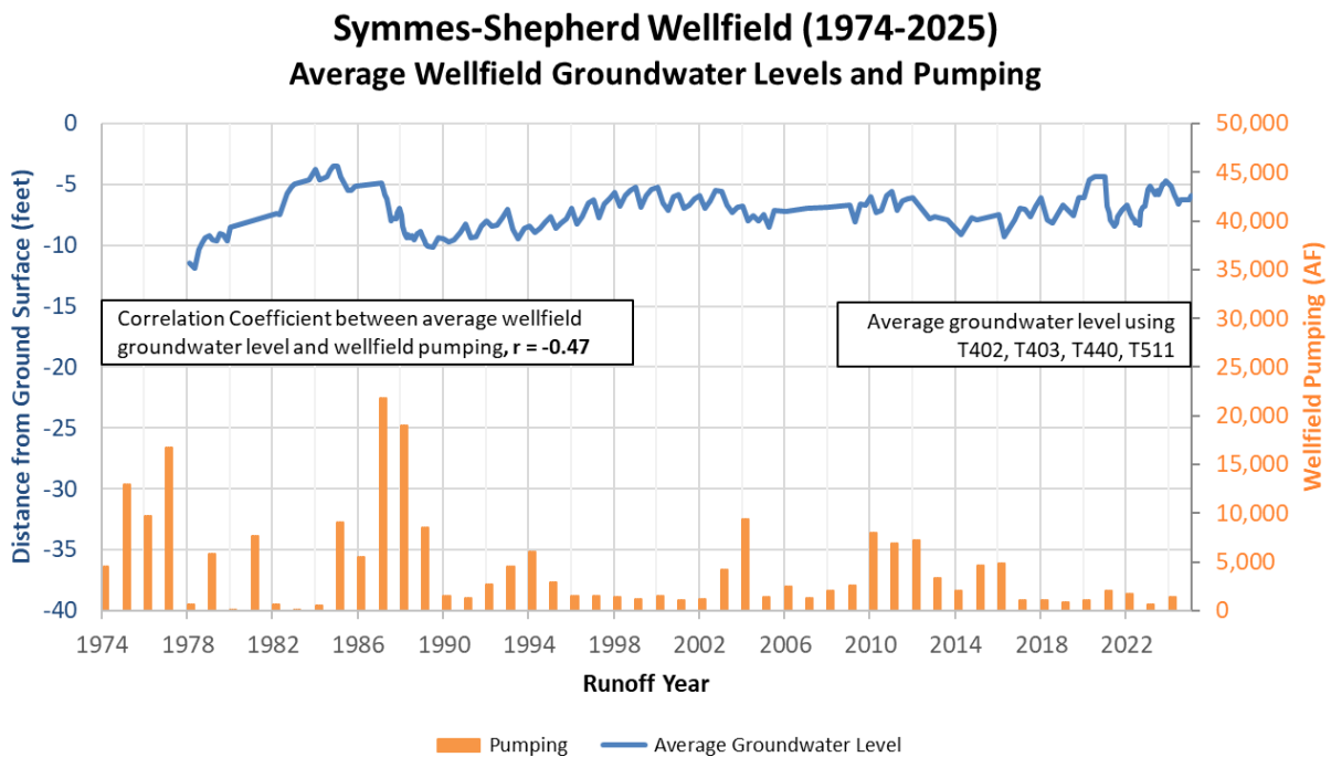
Figure 2.15. Average Symmes-Shepherd Wellfield Groundwater Levels and Pumping
