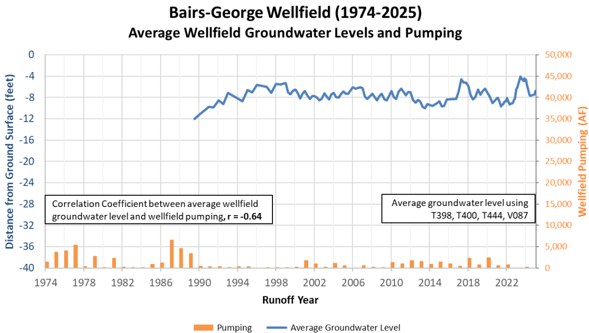
Figure 2.17. Average Bairs-George Wellfield Groundwater Levels and Pumping
