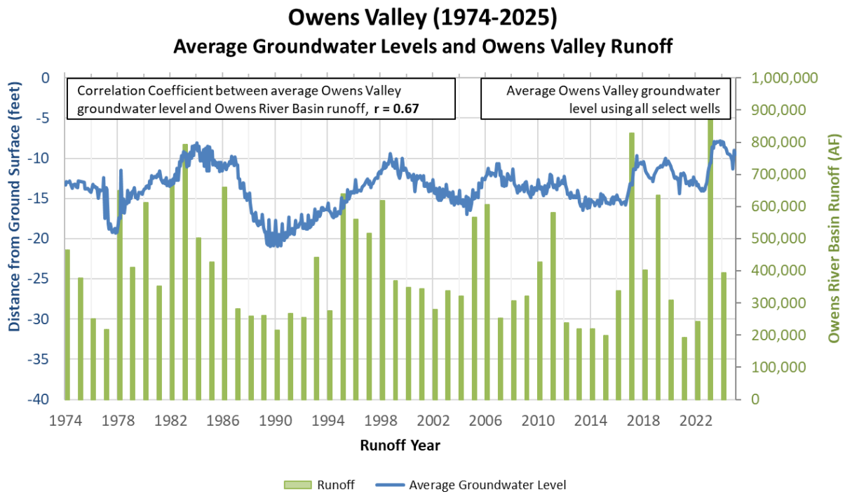
Figure 2.20. Average Owens Valley Groundwater Level and Owens River Basin Runoff
