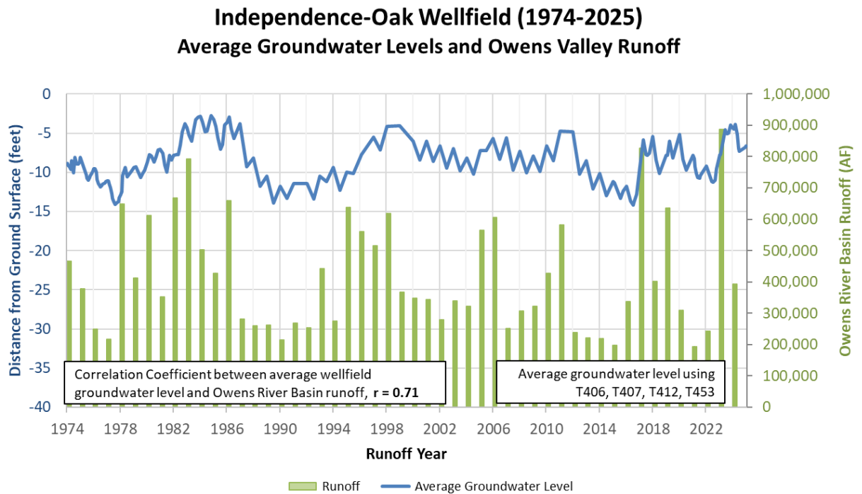
Figure 2.12. Average Independence-Oak Wellfield Groundwater Level and Owens River Basin Runoff
