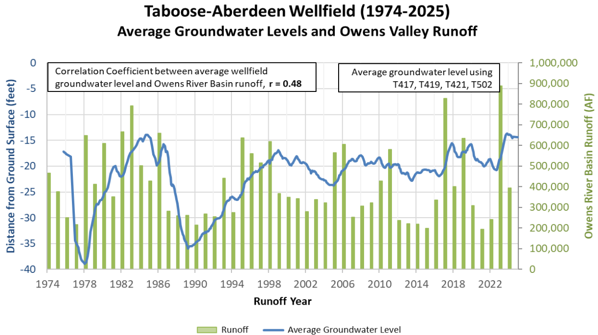
Figure 2.8. Average Taboose-Aberdeen Wellfield Groundwater Level and Owens River Basin Runoff
