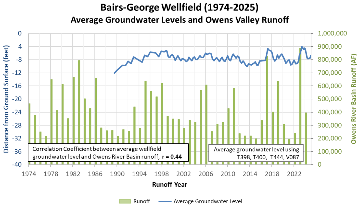
Figure 2.16. Average Bairs-George Wellfield Groundwater Level and Owens River Basin Runoff
