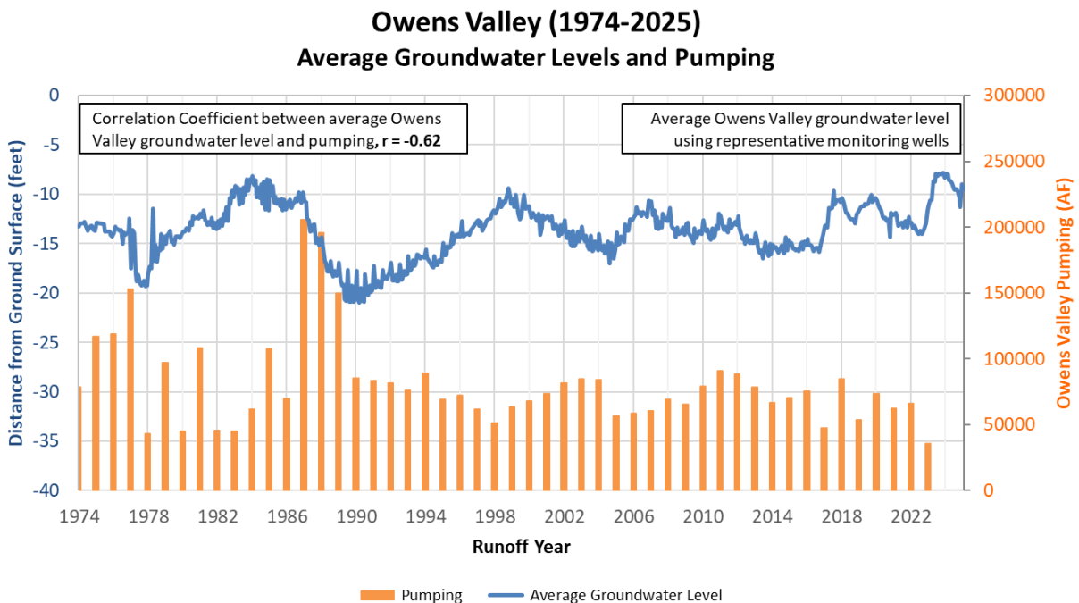
Figure 2.21. Average Owens Valley Groundwater Levels and Pumping
