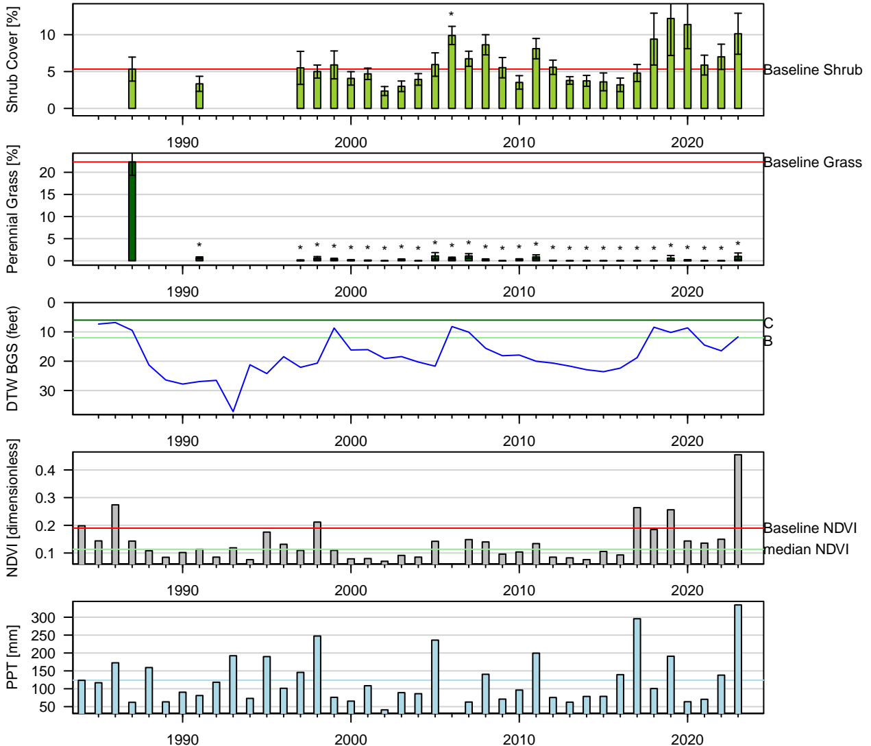
Figure 79: Two-Sample t-Test: Baseline (lpt) vs. reinventory (* p < 0.05 ). Baseline sample size ( n = 6 ). Current year sample size ( n = 8 ). Error bars = 95% CI.
