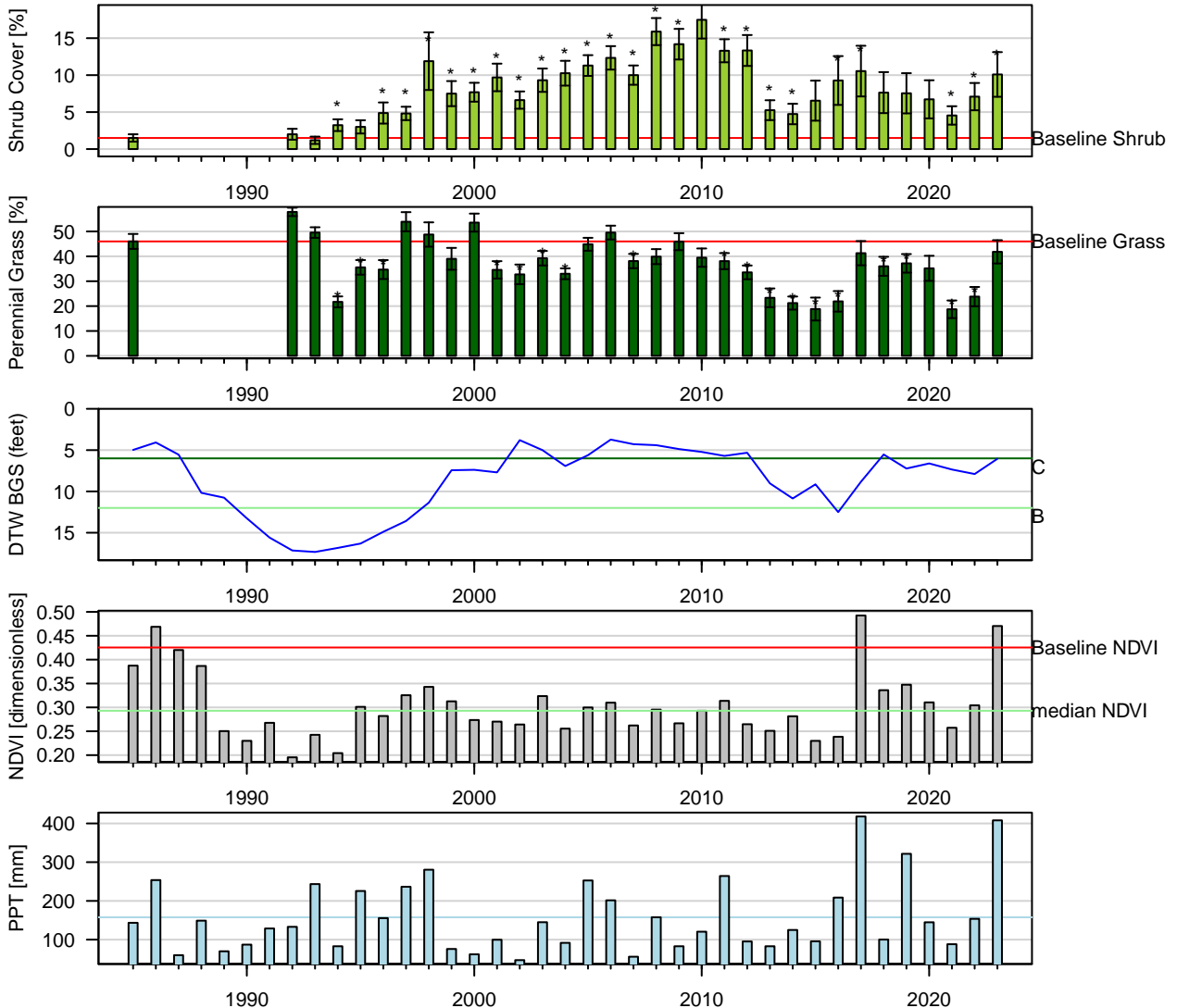
Figure 61: One-Sample t-Test: Baseline (1pt) vs. reinventory (* p < 0.05 ). Baseline sample size (n = 2). Current year sample size (n = 11). Error bars = 95% CI.
