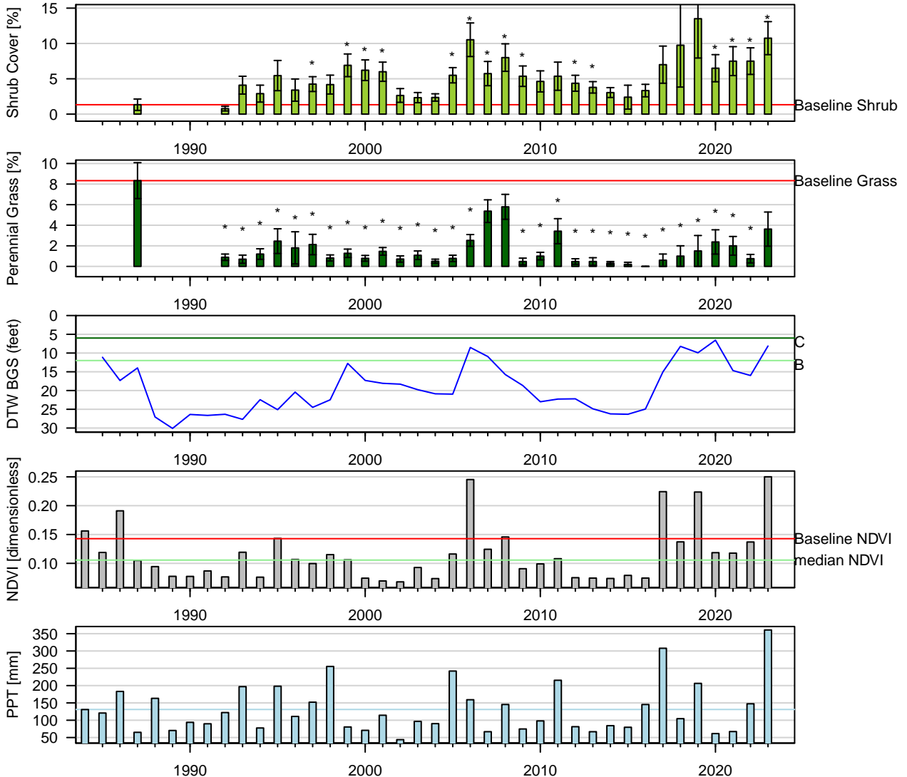
Figure 82: Two-Sample t-Test: Baseline (lpt) vs. reinventory (* p < 0.05 ). Baseline sample size ( n = 6 ). Current year sample size ( n = 8 ). Error bars = 95% CI.
