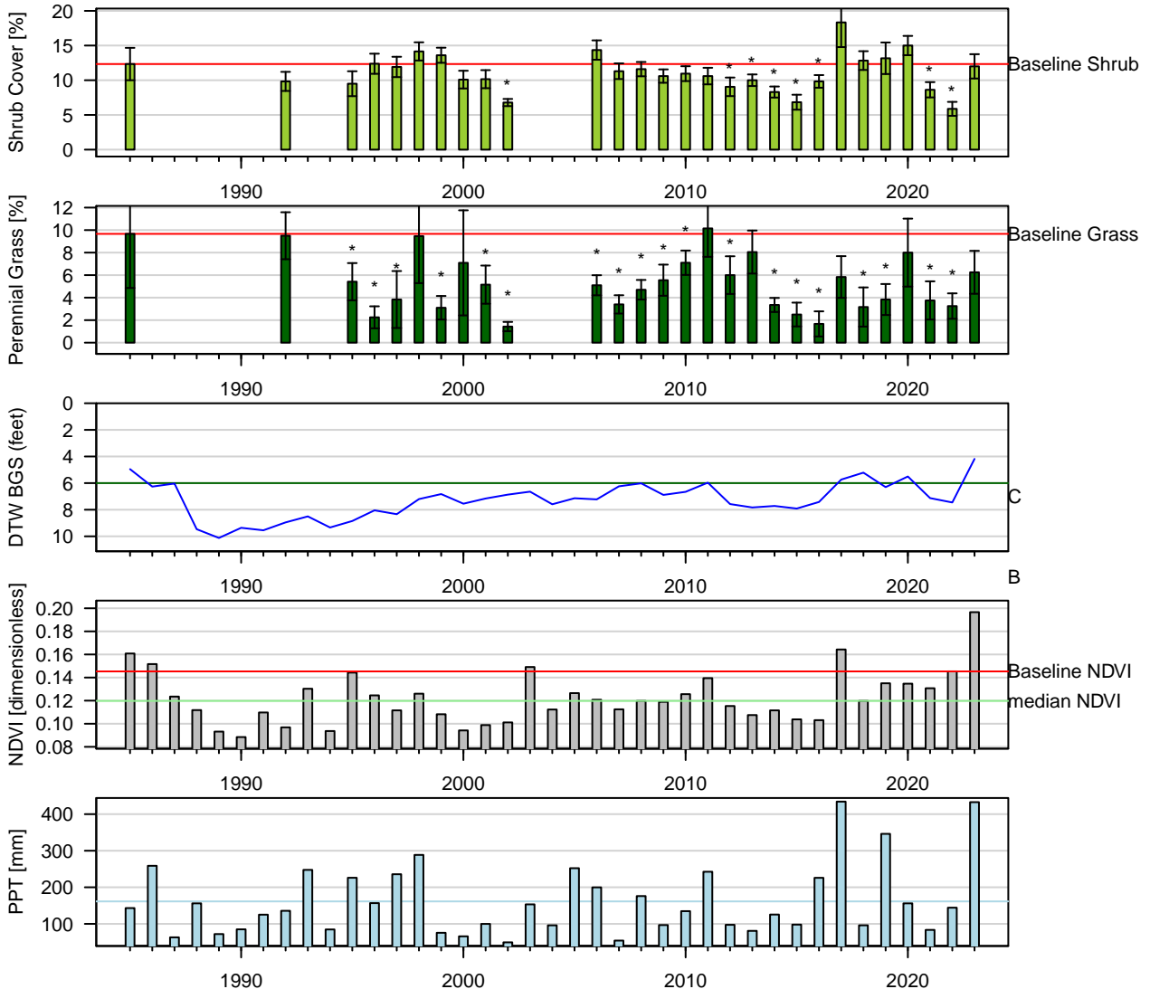
Figure 101: One-Sample t-Test: Baseline (1pt) vs. reinventory (* p < 0.05). Baseline sample size (n = 3). Current year sample size (n = 8). Error bars = 95% CI.
