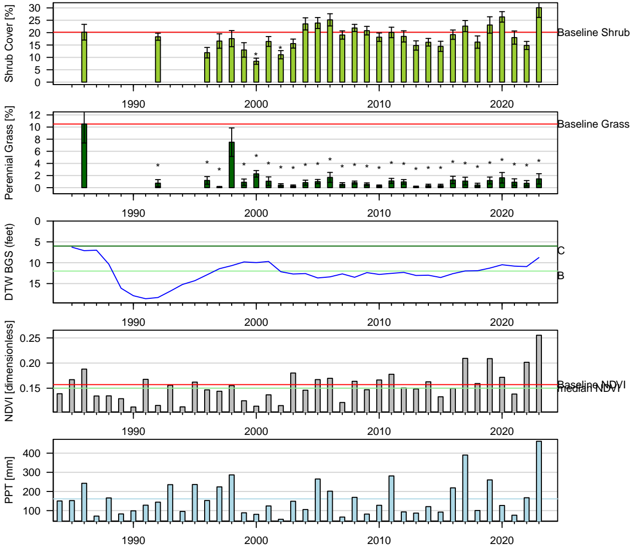
Figure 15: Two-Sample t-Test: Baseline (lpt) vs. reinventory (* p < 0.05 ).
