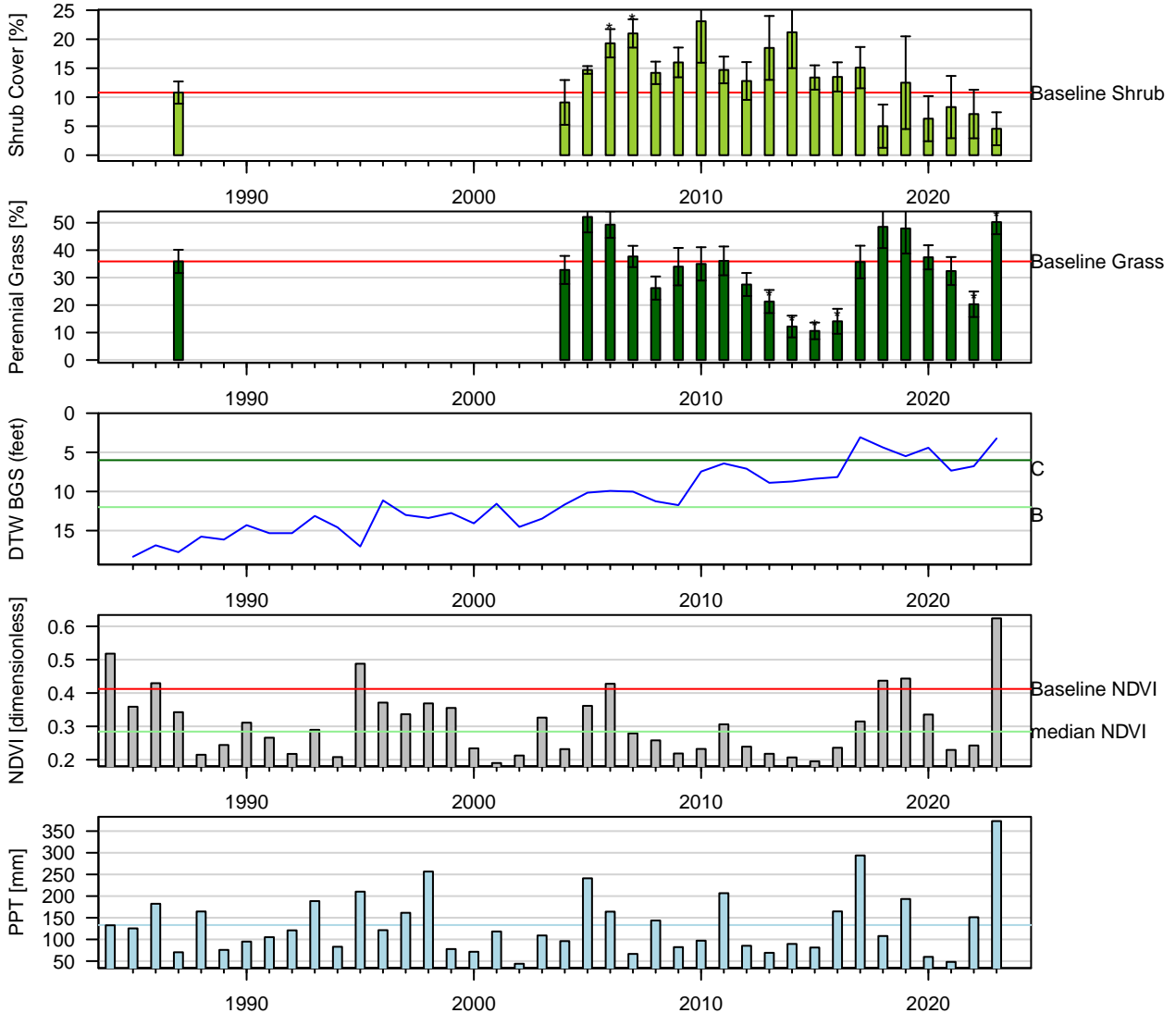
Figure 45: Two-Sample t-Test: Baseline (lpt) vs. reinventory (* p < 0.05 ).
