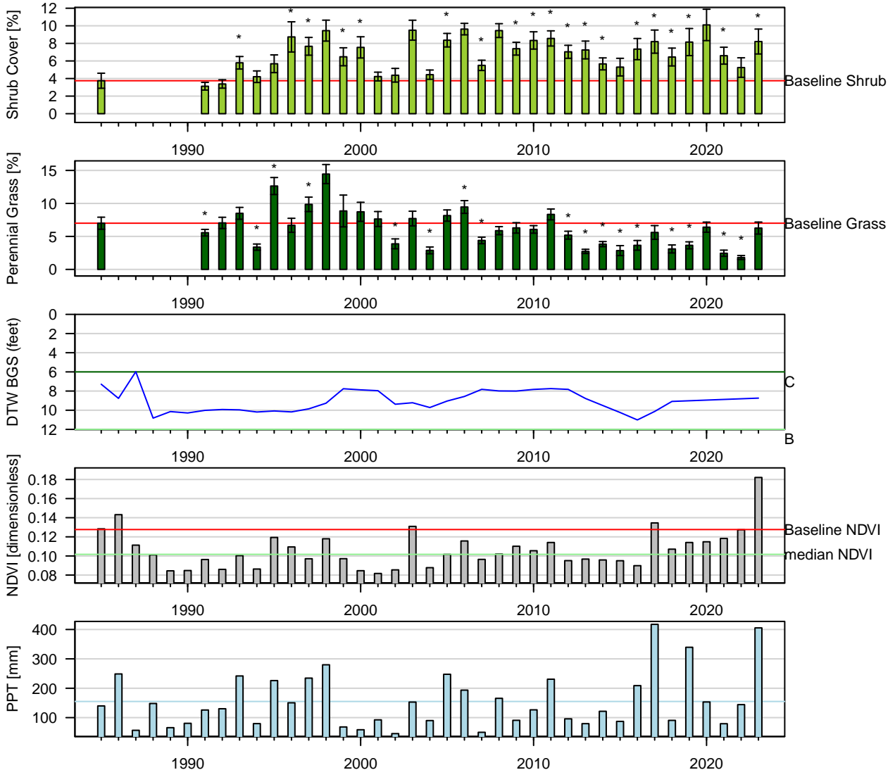
Figure 73: One-Sample t-Test: Baseline (lpt) vs. reinventory (* p < 0.05 ).
