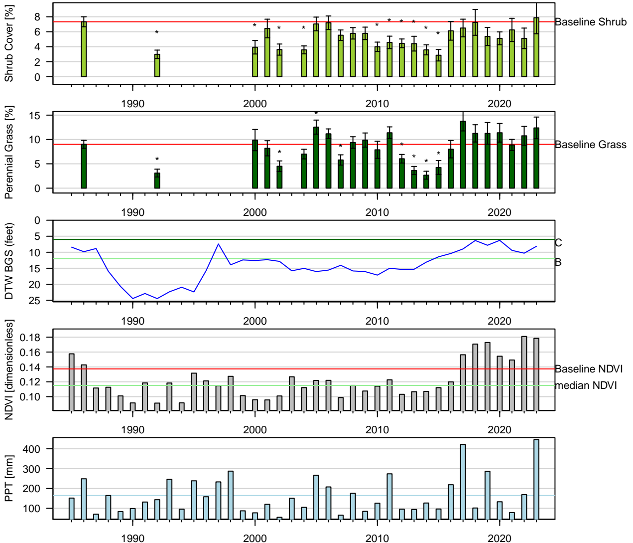
Figure 23: Two-Sample t-Test: Baseline (lpt) vs. reinventory (* p < 0.05 ). Baseline sample size ( n = 6 ). Current year sample size ( n = 8 ). Error bars = 95% CI.
