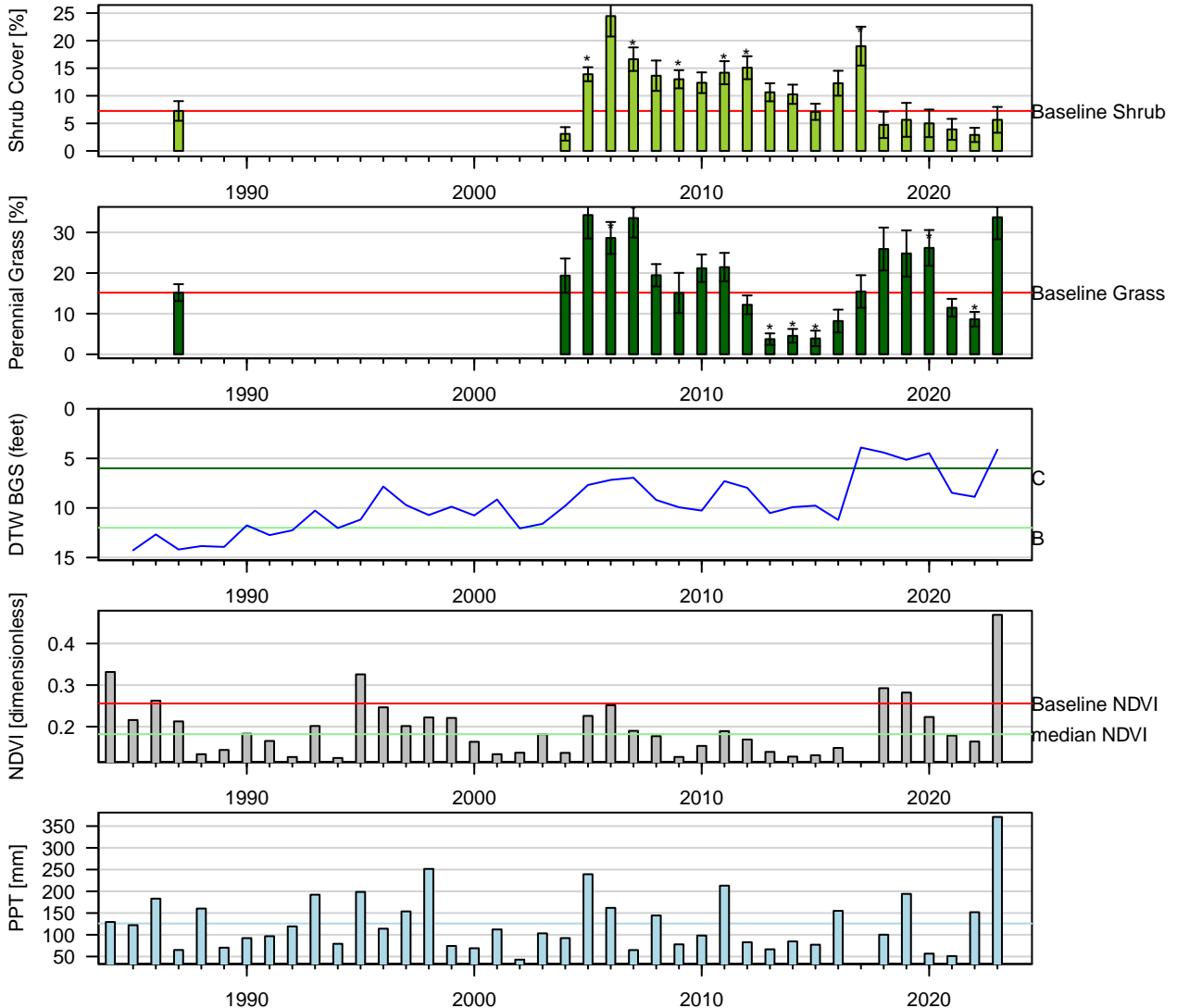
Figure 46: Two-Sample t-Test: Baseline (1pt) vs. reinventory (* p < 0.05 ). Baseline sample size ( n = 12 ). Current year sample size ( n = 11 ). Error bars = 95% CI.
