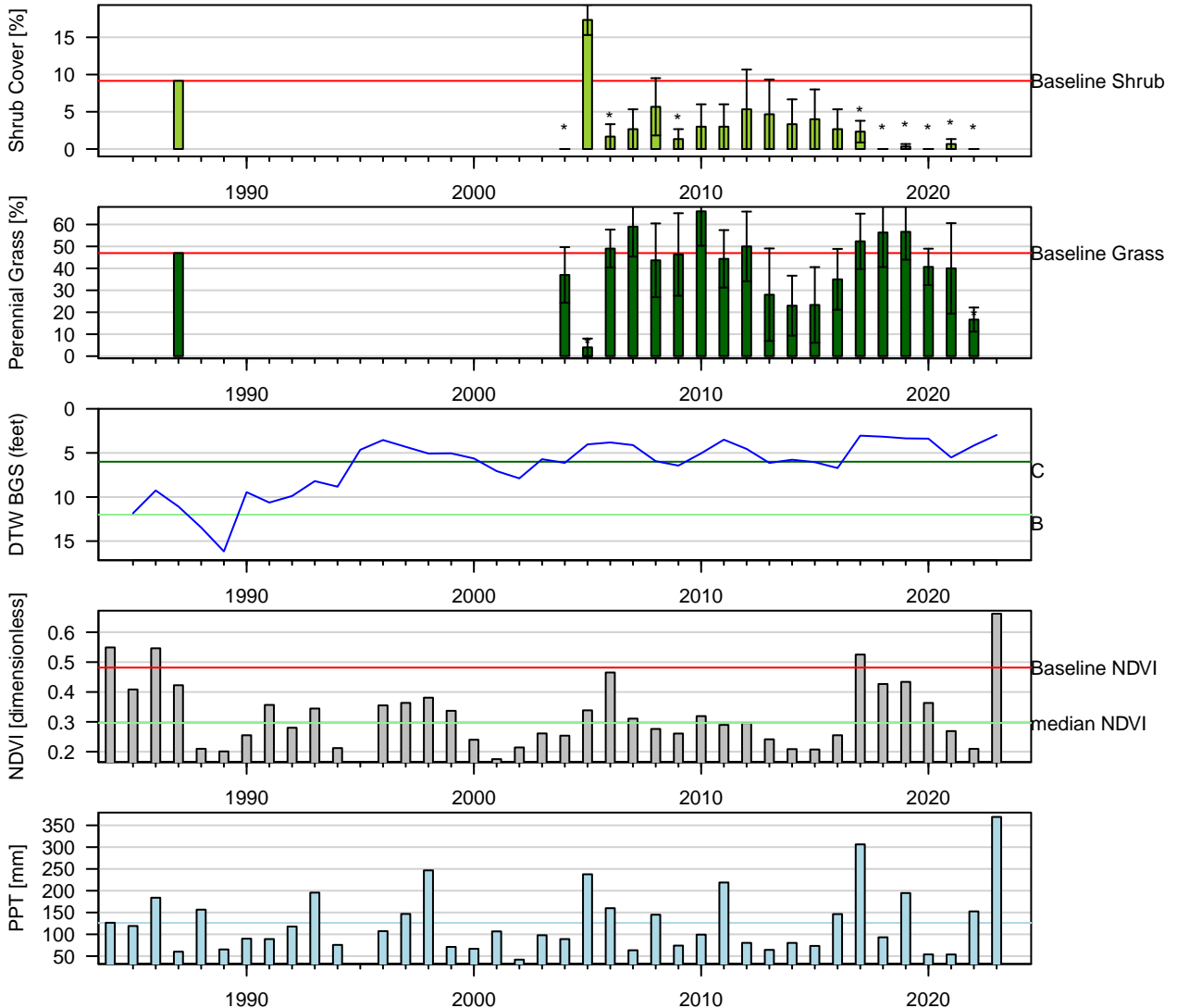
Figure 42: One-Sample t-Test: Baseline (wvcom) vs. reinventory (* p < 0.05 ). Baseline sample size ( n = 1 ). Current year sample size ( n = ). Error bars = 95% CI.
