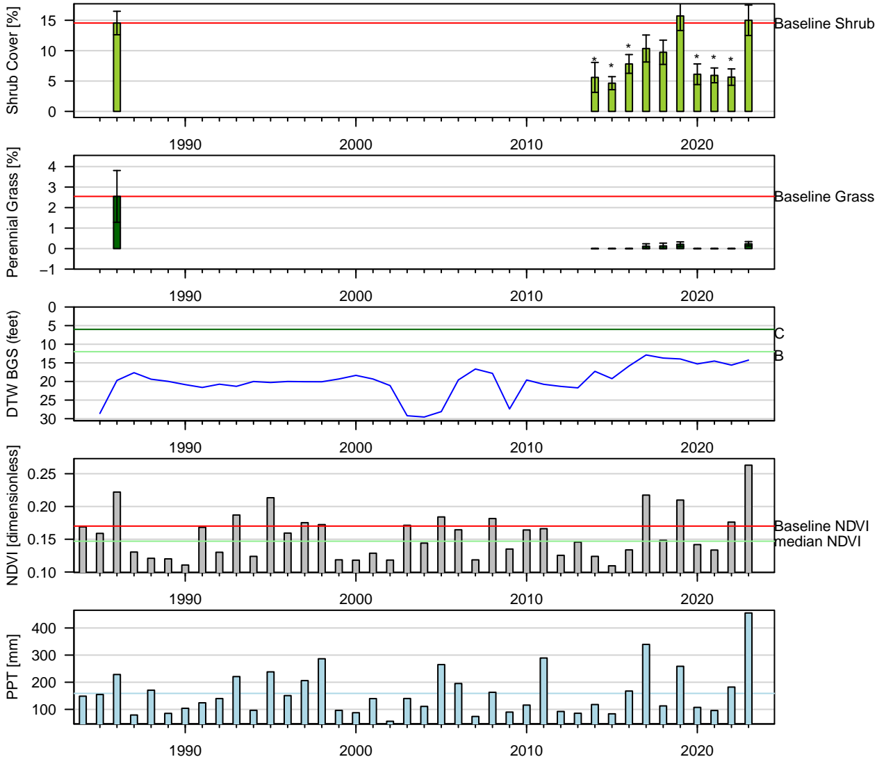
Figure 54: Two-Sample t-Test: Baseline (1pt) vs. reinventory (* p < 0.05 ). Baseline sample size (n = 11). Current year sample size (n = 17). Error bars = 95% CI.
