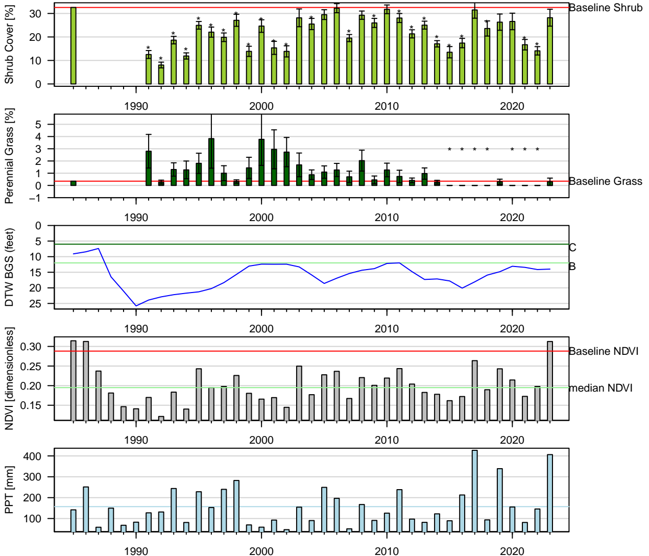
Figure 70: One-Sample t-Test: Baseline (wvcom) vs. reinventory (* p < 0.05 ). Baseline sample size ( n = 1 ). Current year sample size ( n = 10 ). Error bars = 95% CI.
