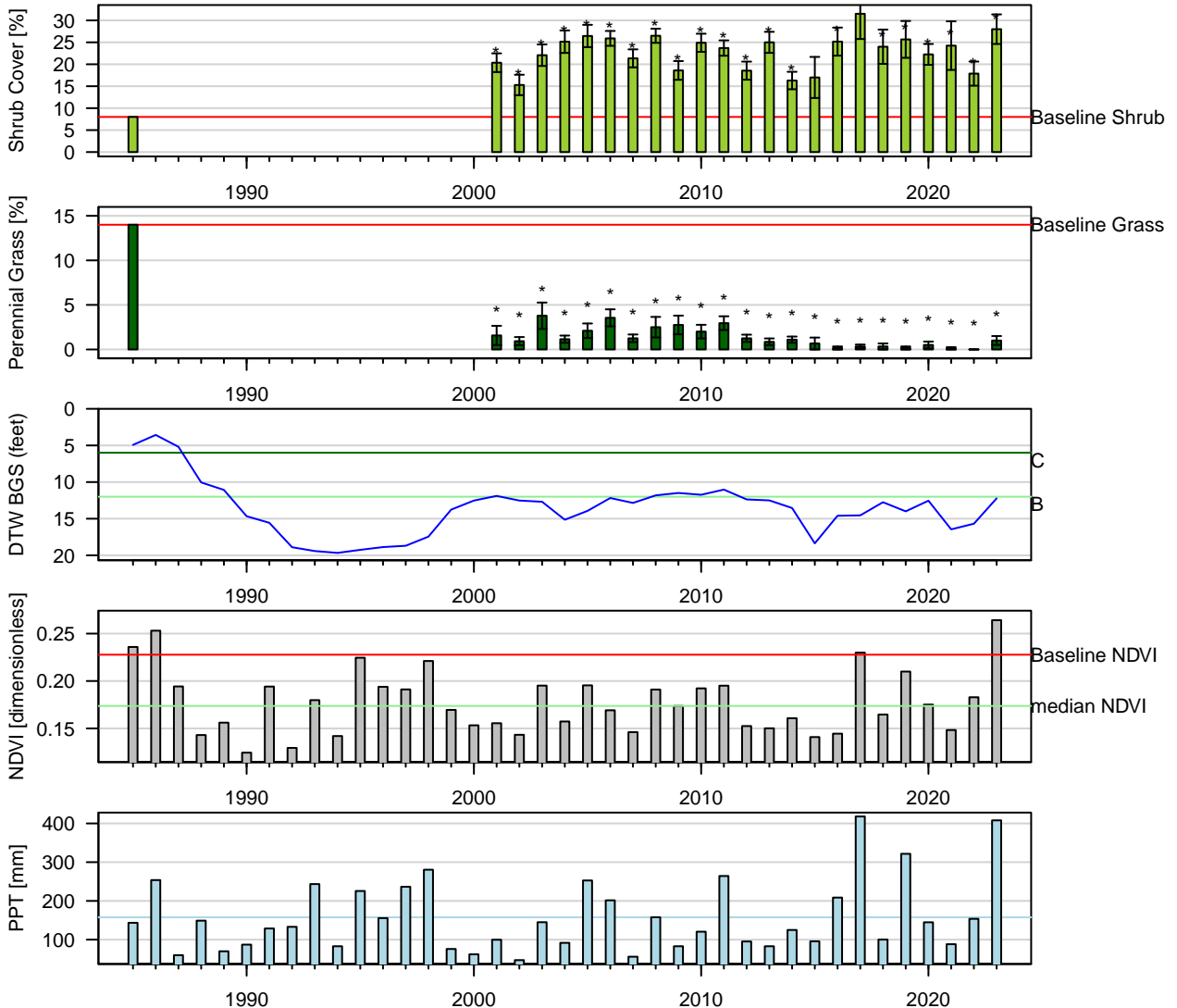
Figure 60: One-Sample t-Test: Baseline (1pt) vs. reinventory (* p < 0.05). Baseline sample size (n = 1). Current year sample size (n = 8). Error bars = 95% CI.
