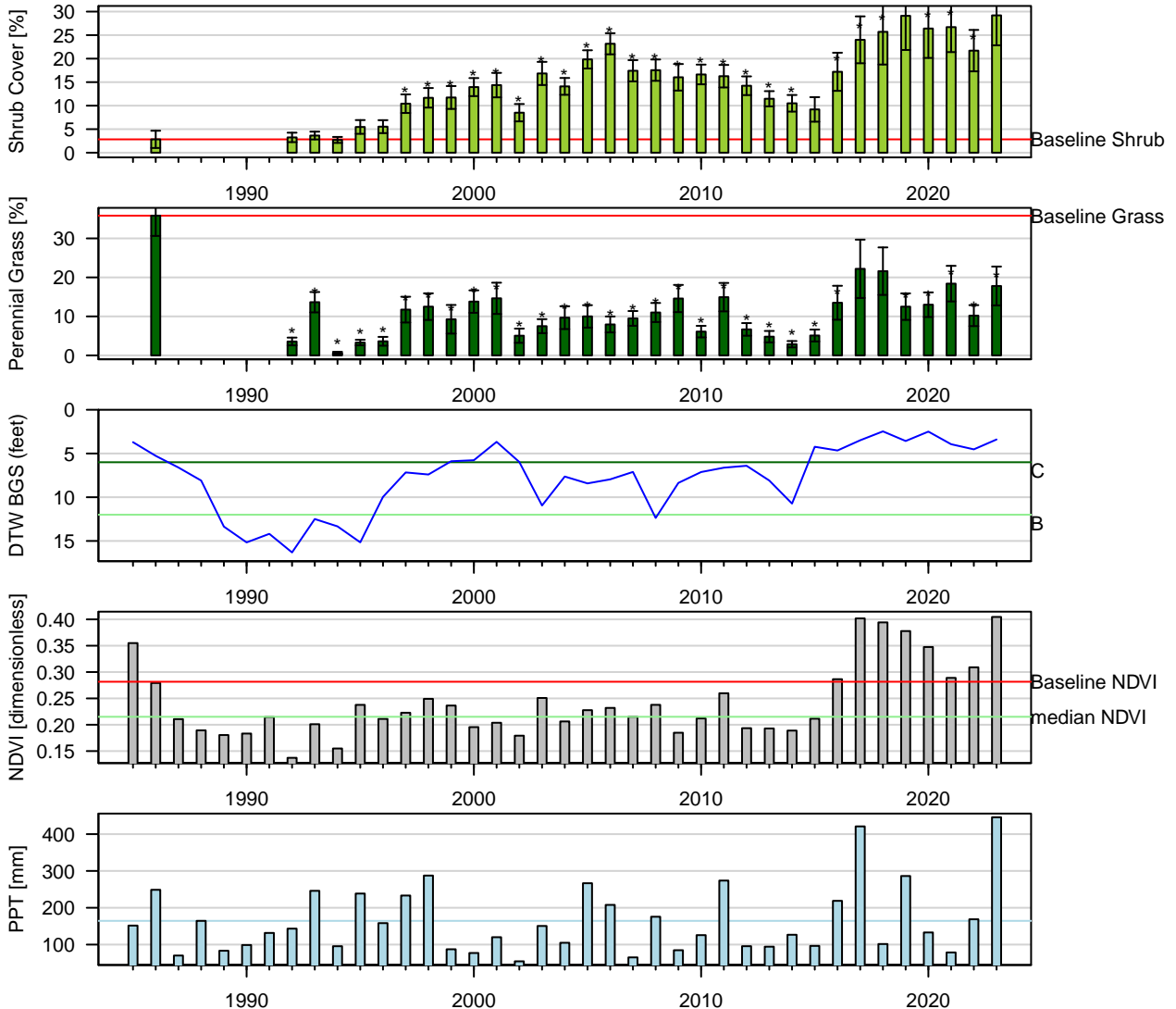
Figure 22: Two-Sample t-Test: Baseline (lpt) vs. reinventory (* p < 0.05 ).
