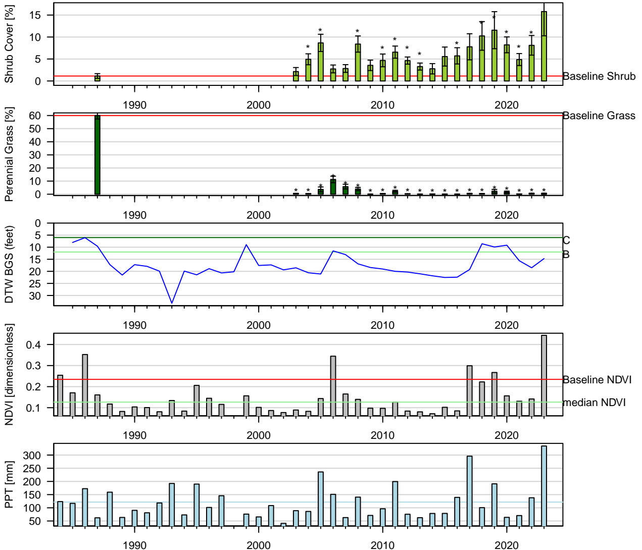
Figure 78: Two-Sample t-Test: Baseline (1pt) vs. reinventory (* p < 0.05 ). Baseline sample size ( n = 8 ). Current year sample size ( n = 5 ). Error bars = 95% CI.
