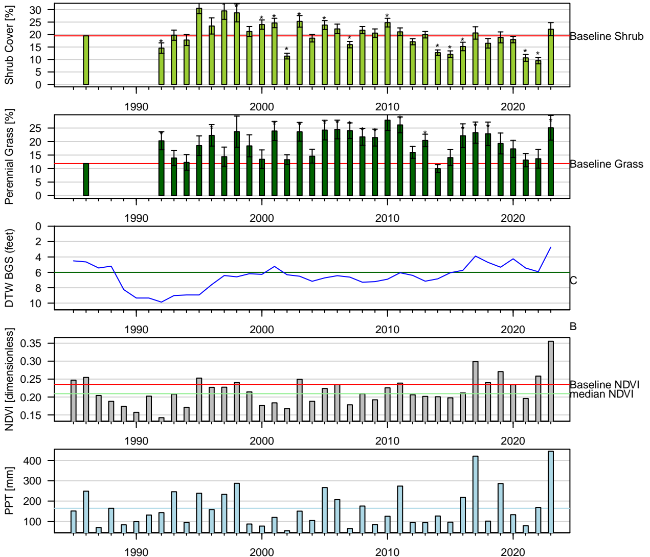
Figure 21: One-Sample t-Test: Baseline (wvcom) vs. reinventory (* p < 0.05 ). Baseline sample size ( n = 1 ). Current year sample size ( n = 14 ). Error bars = 95% CI.
