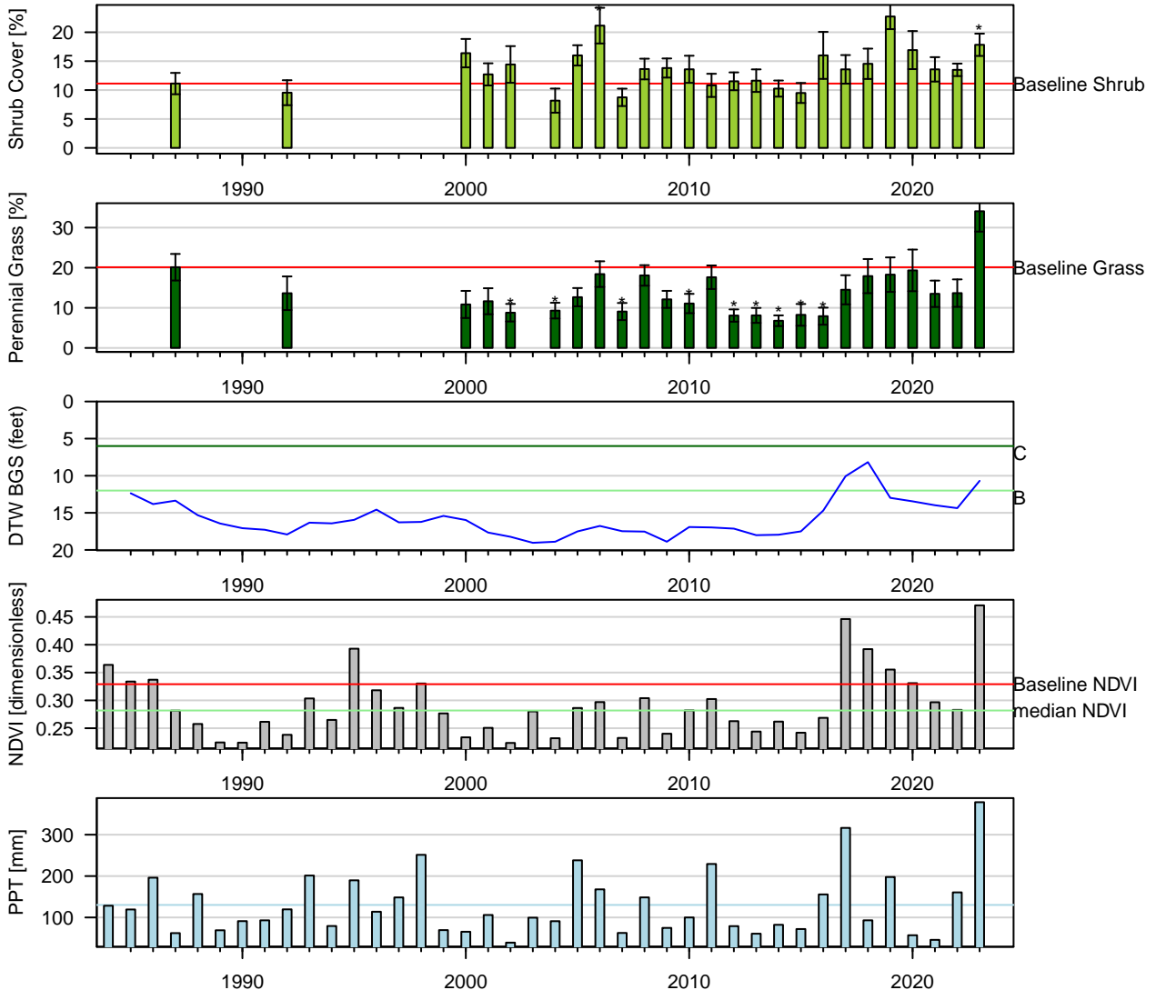
Figure 10: Two-Sample t-Test: Baseline (lpt) vs. reinventory (* p < 0.05 ).
