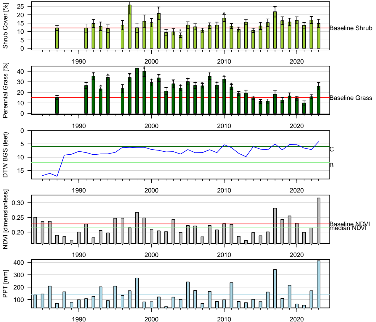
Figure 114: Two-Sample t-Test: Baseline (1pt) vs. reinventory (* p < 0.05 ). Baseline sample size ( n = 10 ). Current year sample size ( n = 16 ). Error bars = 95% CI.
