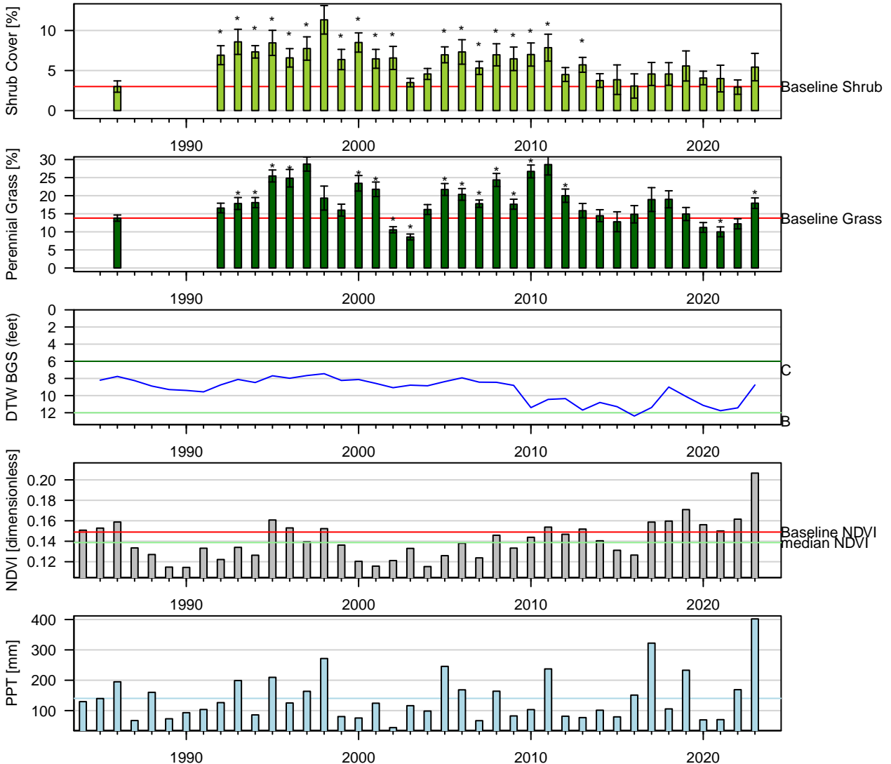
Figure 1: Two-Sample t-Test: Baseline (1pt) vs. reinventory (* p < 0.05 ). Baseline sample size ( n = 5 ). Current year sample size ( n = 14 ). Error bars = 95% CI.
