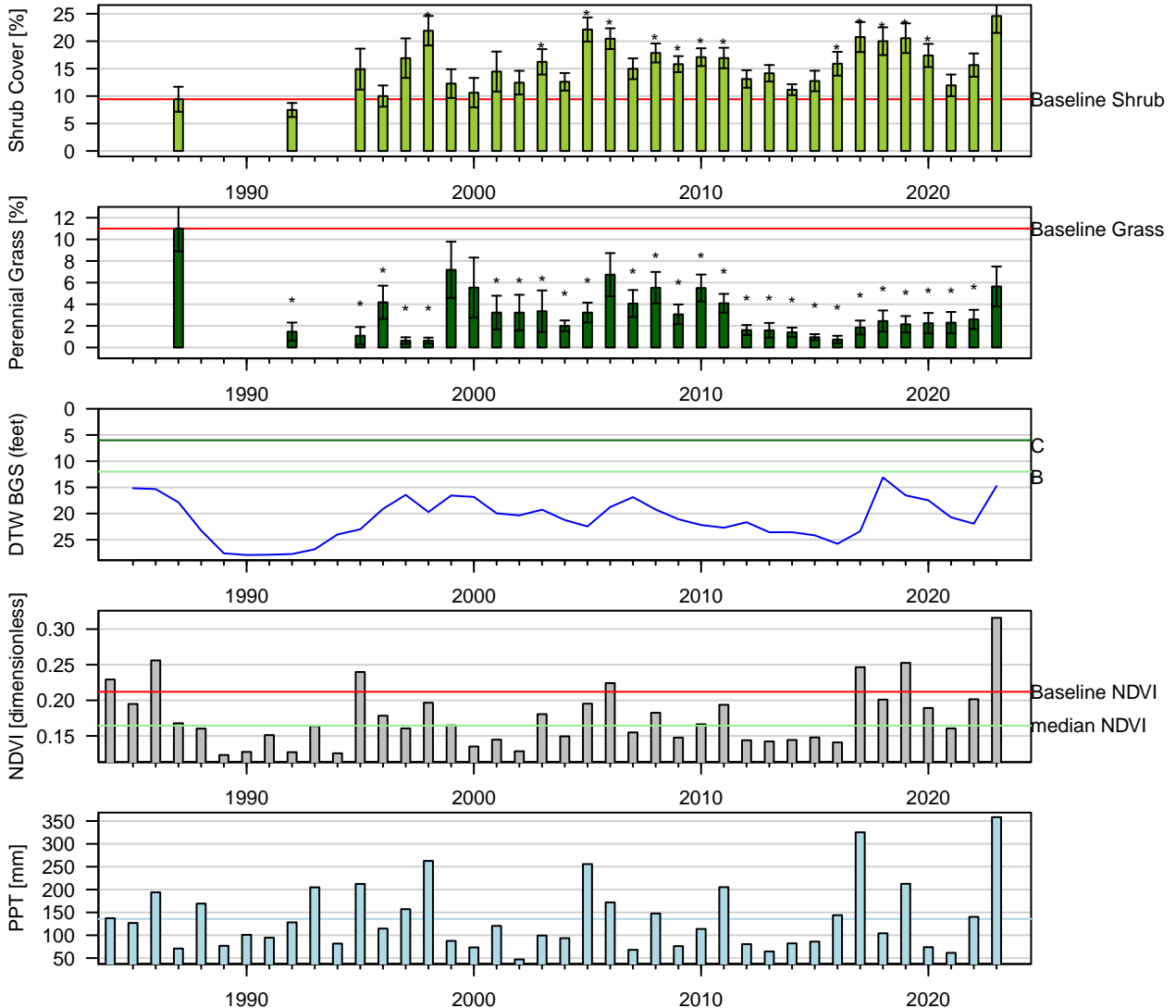
Figure 94: Two-Sample t-Test: Baseline (lpt) vs. reinventory (* p < 0.05 ). Baseline sample size ( n = 12 ). Current year sample size ( n = 17 ). Error bars = 95% CI.
