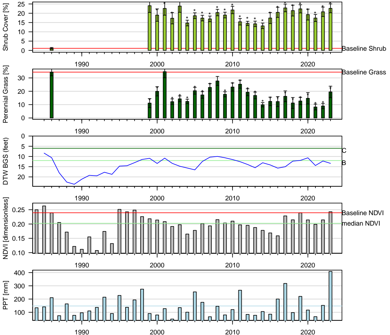
Figure 119: Two-Sample t-Test: Baseline (1pt) vs. reinventory (* p < 0.05 ). Baseline sample size ( n = 9 ). Current year sample size ( n = 14 ). Error bars = 95% CI.
