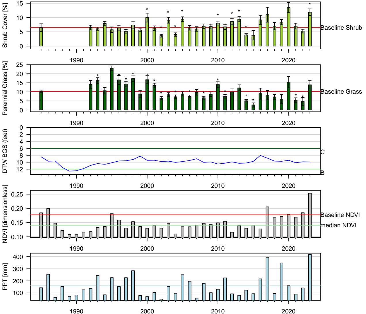
Figure 123: One-Sample t-Test: Baseline (1pt) vs. reinventory (* p < 0.05 ). Baseline sample size ( n = 4 ). Current year sample size ( n = 8 ). Error bars = 95% CI.
