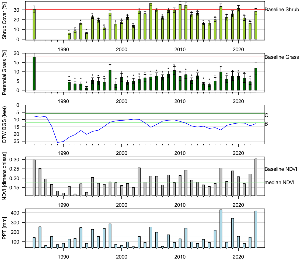
Figure 72: One-Sample t-Test: Baseline (1pt) vs. reinventory (* p < 0.05 ). Baseline sample size ( n = 2 ). Current year sample size ( n = 21 ). Error bars = 95% CI.
