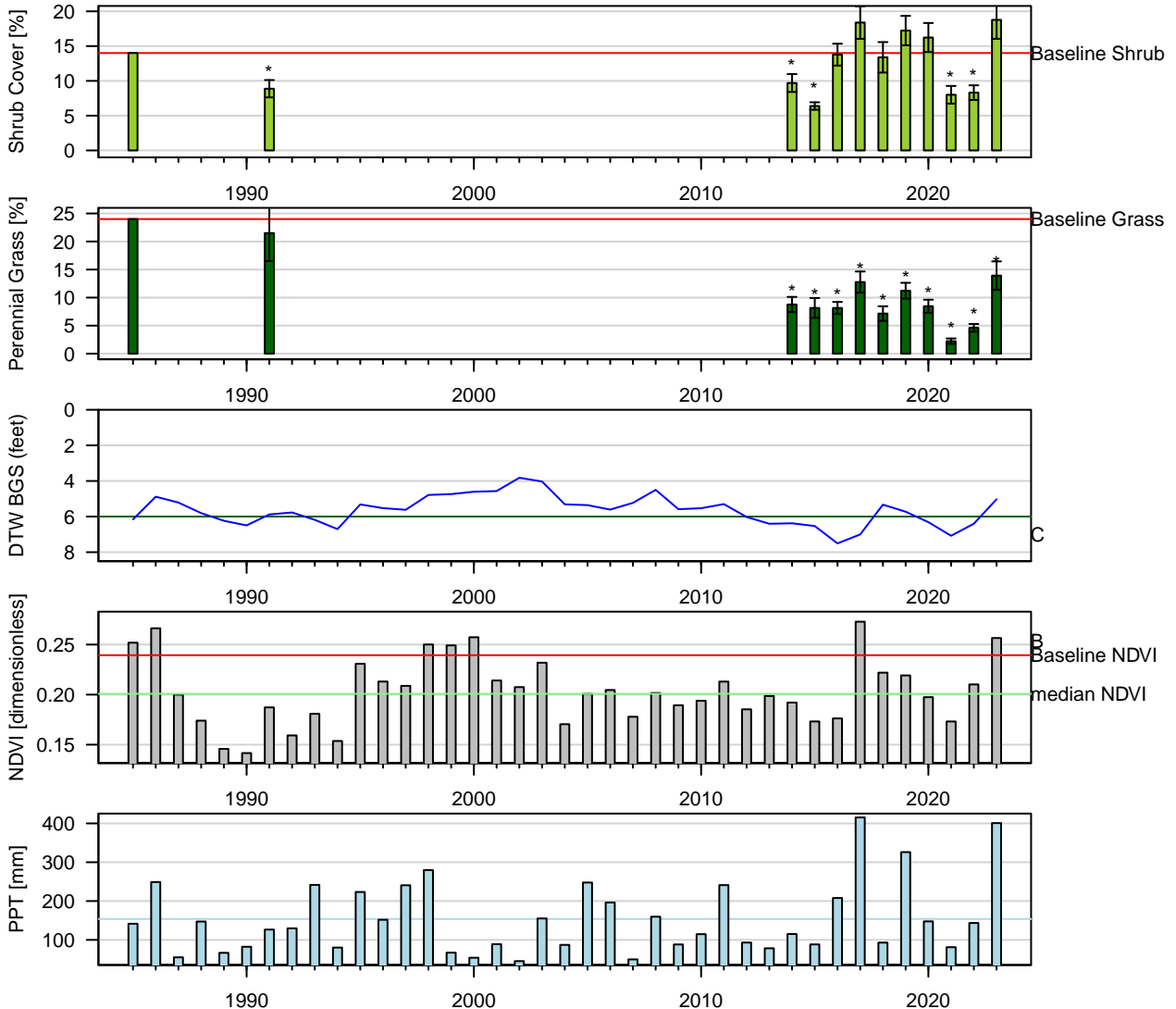
Figure 64: One-Sample t-Test: Baseline (1pt) vs. reinventory (* p < 0.05 ).
