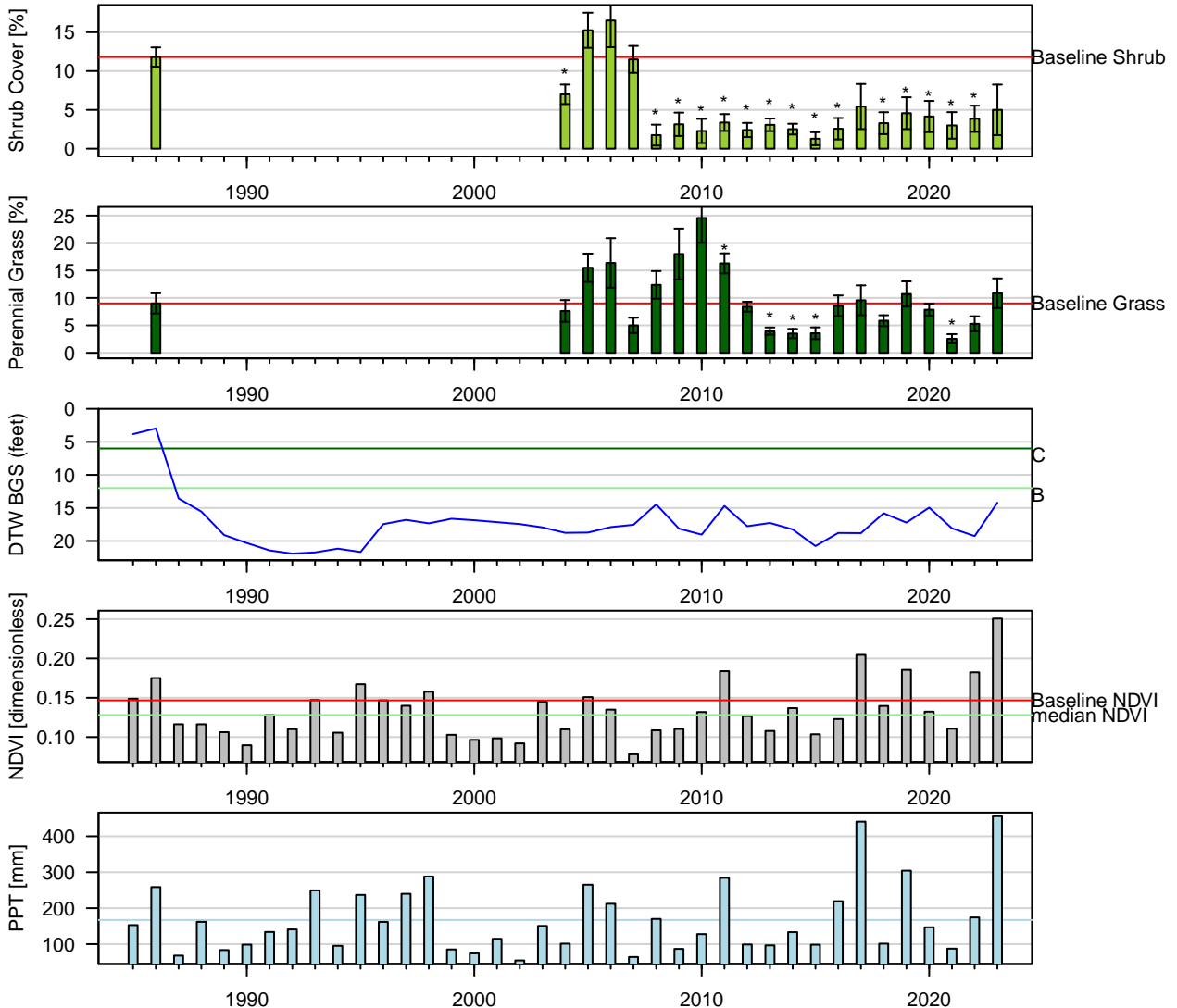
Figure 26: Two-Sample t-Test: Baseline (1pt) vs. reinventory (* p < 0.05 ). Baseline sample size ( n = 5 ). Current year sample size ( n = 7 ). Error bars = 95% CI.
