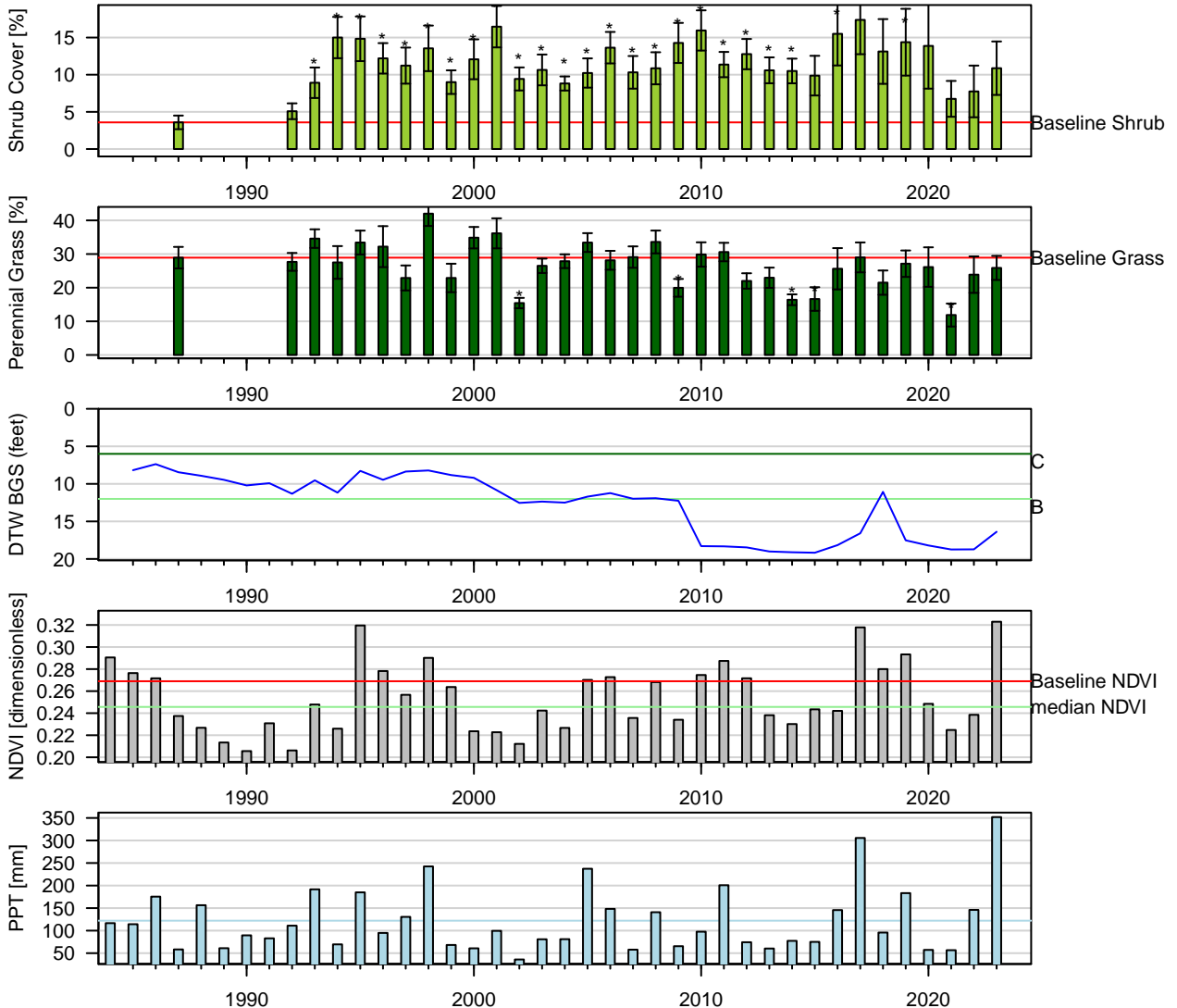
Figure 107: Two-Sample t-Test: Baseline (1pt) vs. reinventory (* p < 0.05 ). Baseline sample size ( n = 12 ). Current year sample size ( n = 8 ). Error bars = 95% CI.
