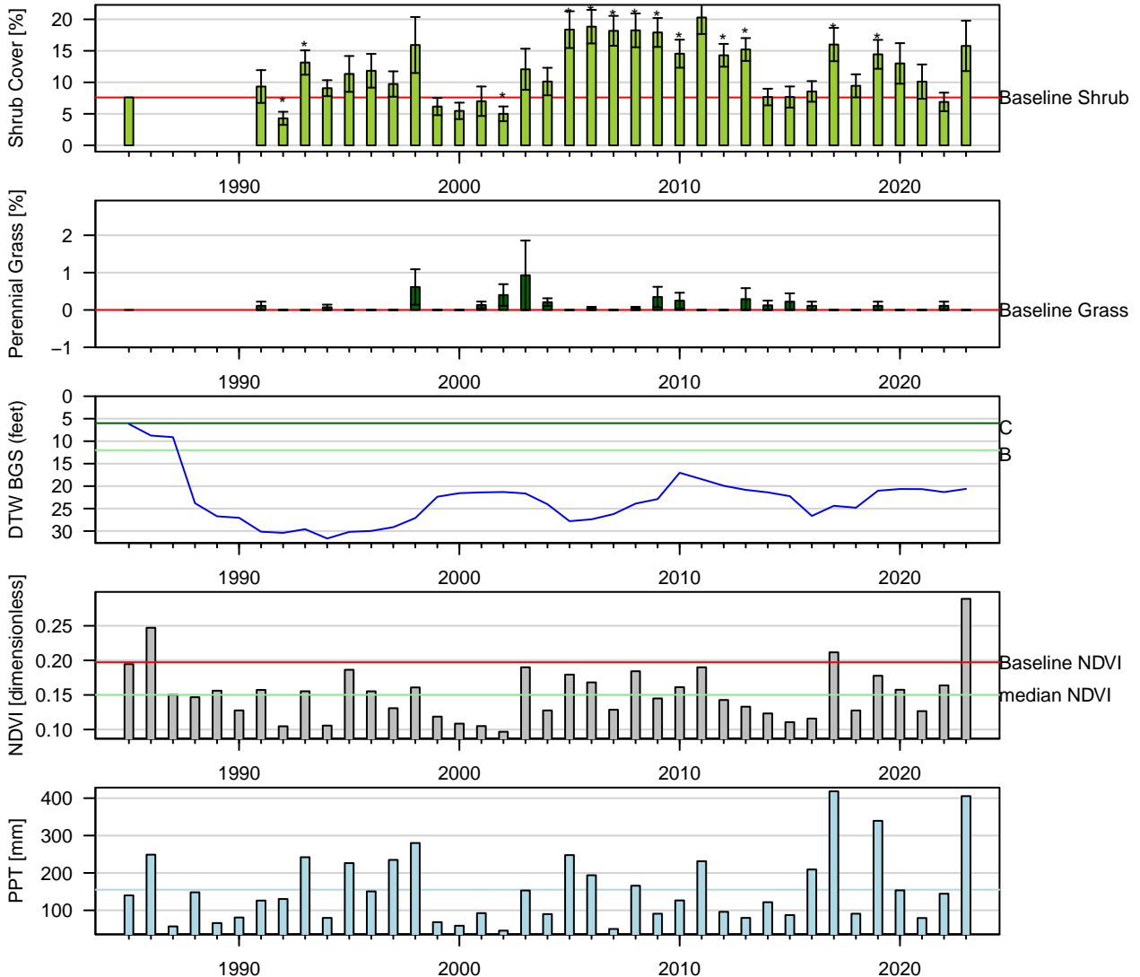
Figure 75: One-Sample t-Test: Baseline (wvcom) vs. reinventory (* p < 0.05 ). Baseline sample size ( n = 1 ). Current year sample size ( n = 9 ). Error bars = 95% CI.
