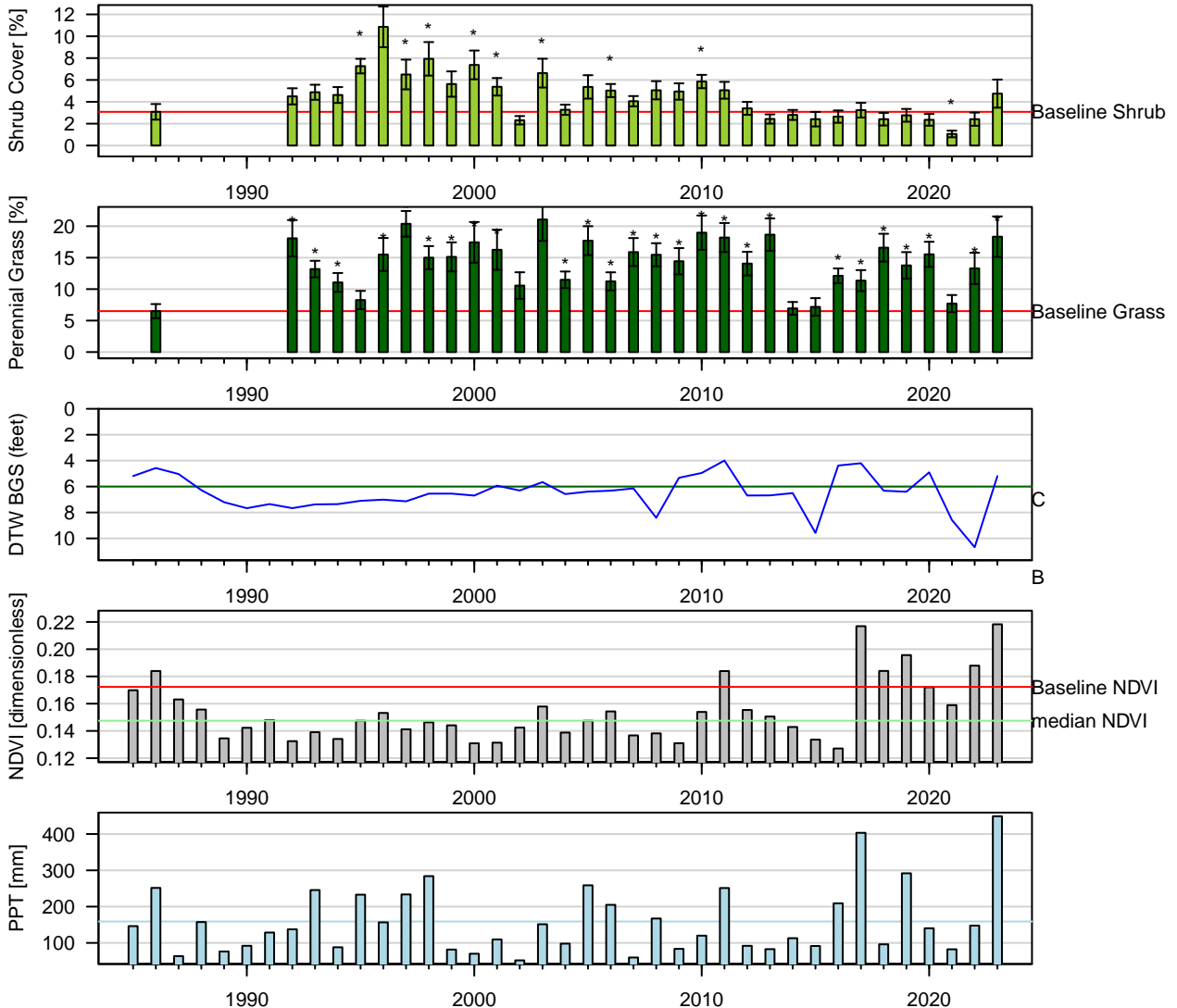
Figure 28: Two-Sample t-Test: Baseline (lpt) vs. reinventory (* p < 0.05 ). Baseline sample size ( n = 12 ). Current year sample size ( n = 12 ). Error bars = 95% CI.
