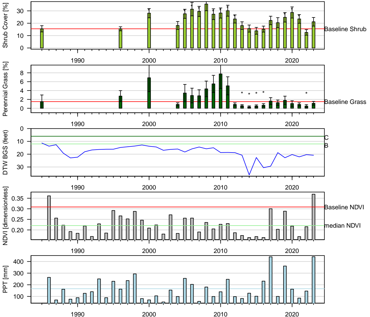
Figure 104: One-Sample t-Test: Baseline (1pt) vs. reinventory (* p < 0.05 ). Baseline sample size ( n = 2 ). Current year sample size ( n = 17 ). Error bars = 95% CI.
