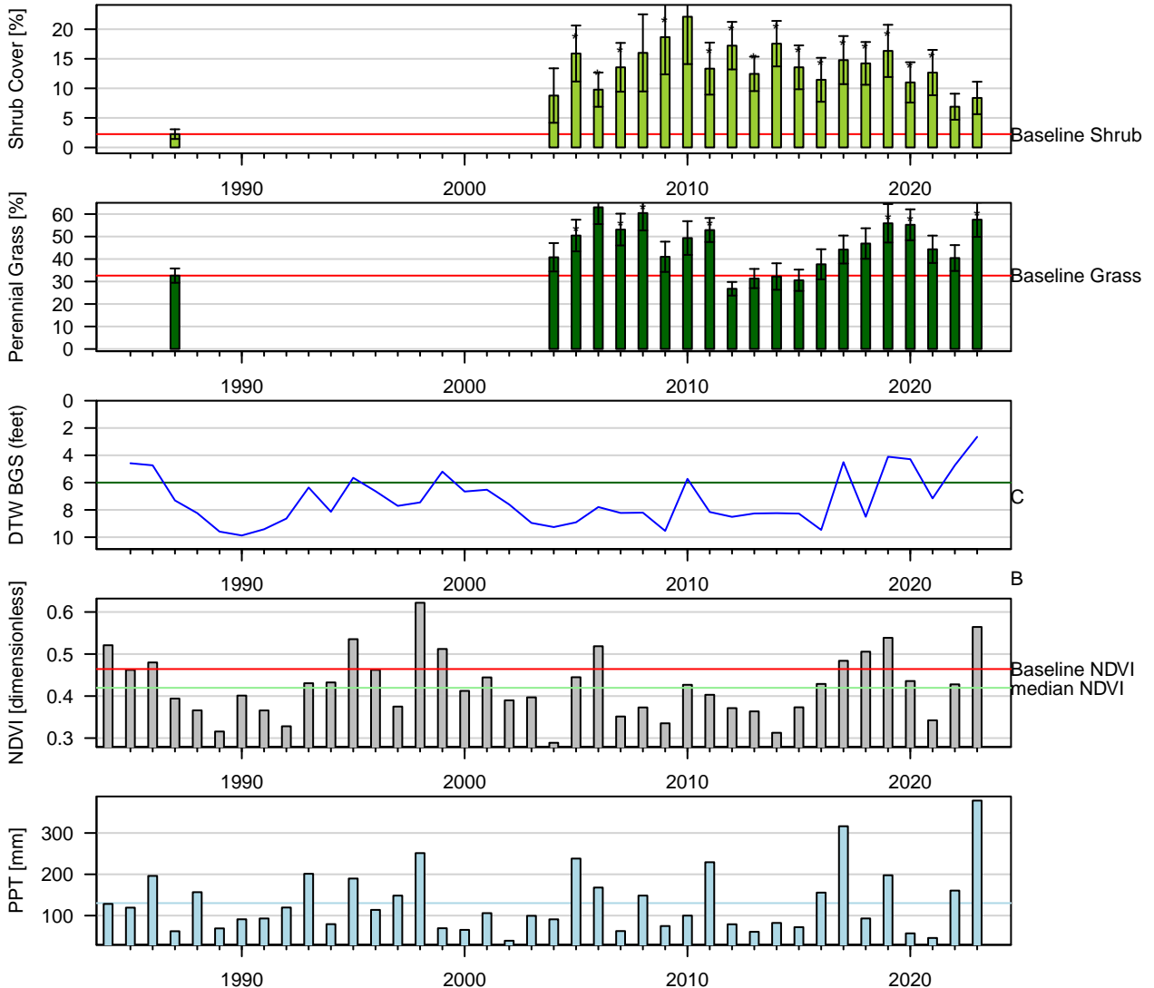
Figure 9: Two-Sample t-Test: Baseline (1pt) vs. reinventory (* p < 0.05). Baseline sample size (n = 8). Current year sample size (n = 8). Error bars = 95% CI.
