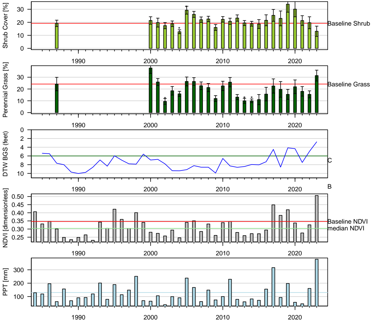
Figure 8: Two-Sample t-Test: Baseline (lpt) vs. reinventory (* p < 0.05 ). Baseline sample size ( n = 10 ). Current year sample size ( n = 8 ). Error bars = 95% CI.
