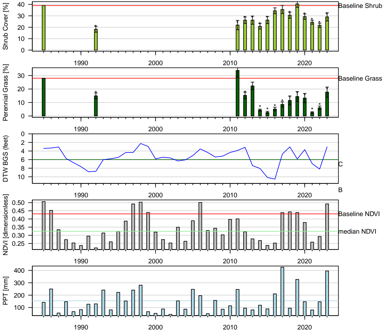
Figure 57: One-Sample t-Test: Baseline (1pt) vs. reinventory (* p < 0.05 ). Baseline sample size ( n = 1 ). Current year sample size ( n = 14 ). Error bars = 95% CI.
