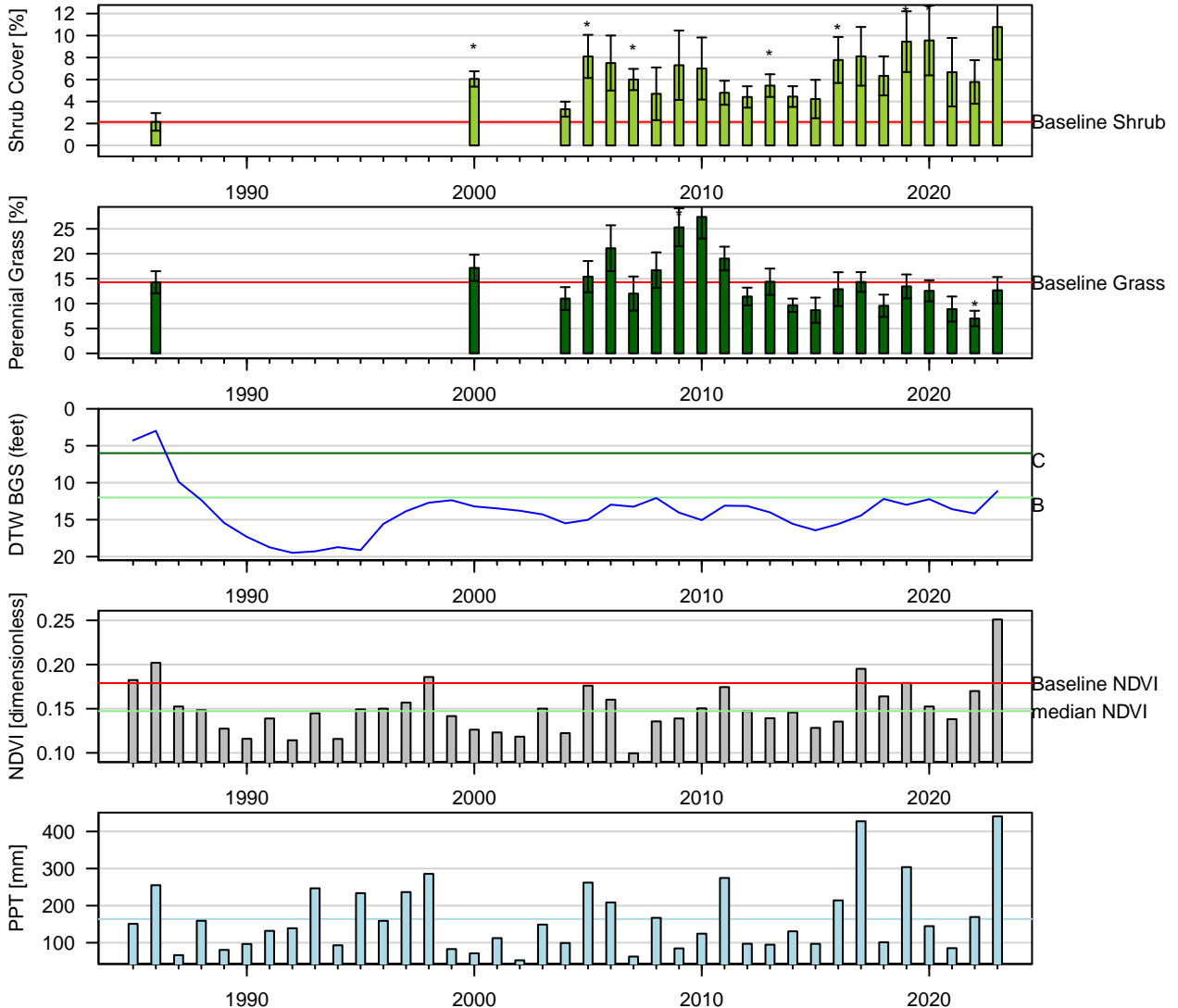
Figure 25: Two-Sample t-Test: Baseline (lpt) vs. reinventory (* p < 0.05 ). Baseline sample size ( n = 7 ). Current year sample size ( n = 9 ). Error bars = 95% CI.
