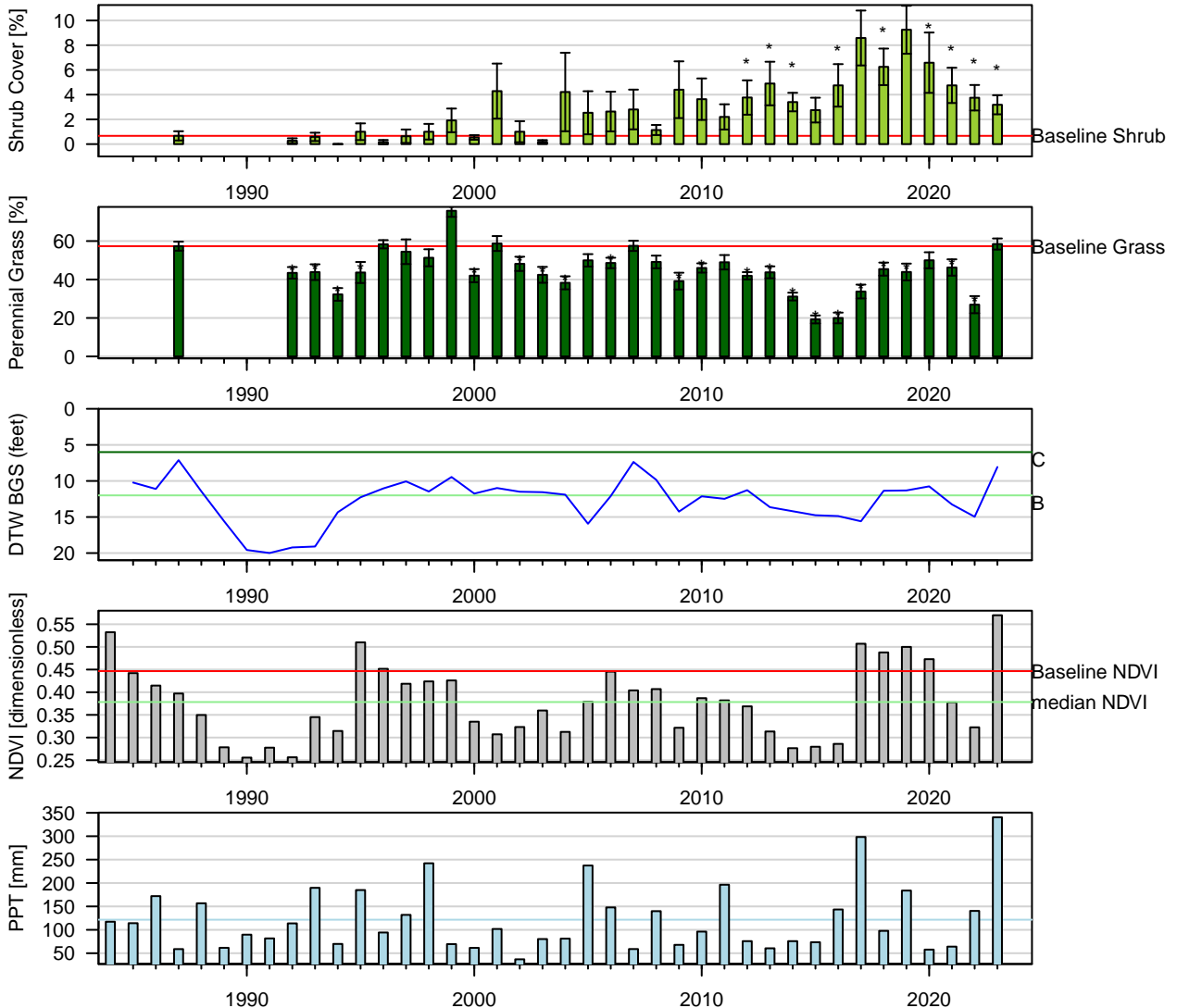
Figure 93: Two-Sample t-Test: Baseline (lpt) vs. reinventory (* p < 0.05 ).
