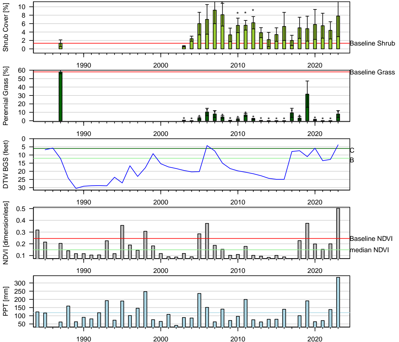
Figure 83: Two-Sample t-Test: Baseline (lpt) vs. reinventory (* p < 0.05 ). Baseline sample size ( n = 6 ). Current year sample size ( n = 5 ). Error bars = 95% CI.
