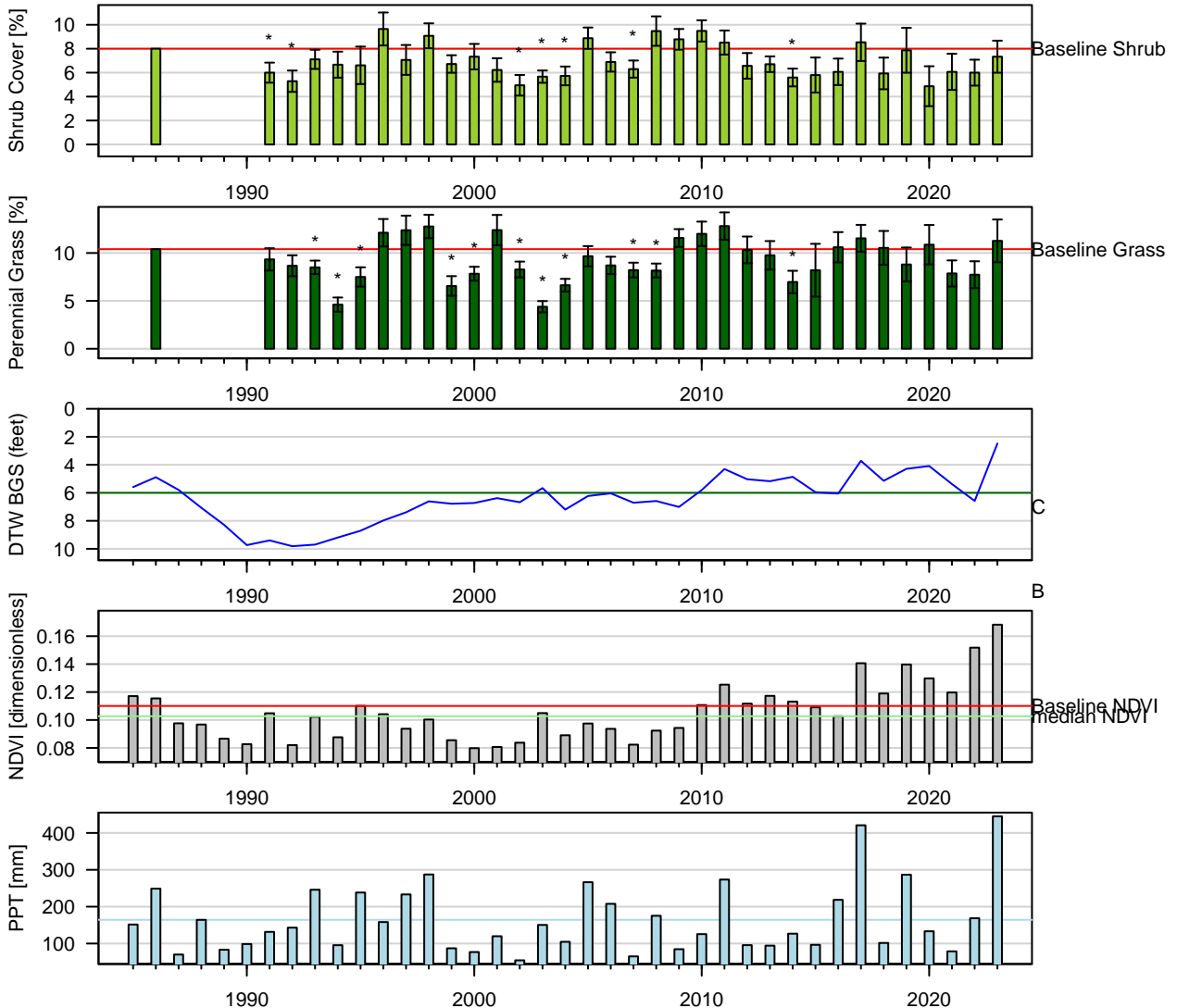
Figure 20: One-Sample t-Test: Baseline (wvcom) vs. reinventory (* p < 0.05 ). Baseline sample size ( n = 1 ). Current year sample size ( n = 15 ). Error bars = 95% CI.
