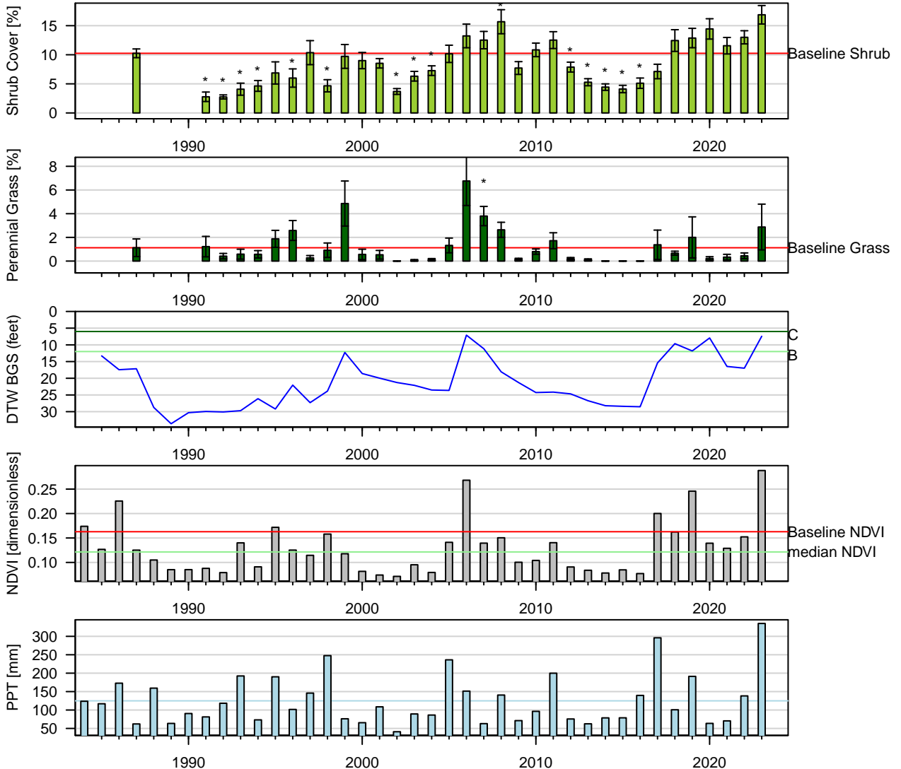
Figure 81: Two-Sample t-Test: Baseline (1pt) vs. reinventory (* p < 0.05 ). Baseline sample size ( n = 8 ). Current year sample size ( n = 8 ). Error bars = 95% CI.
