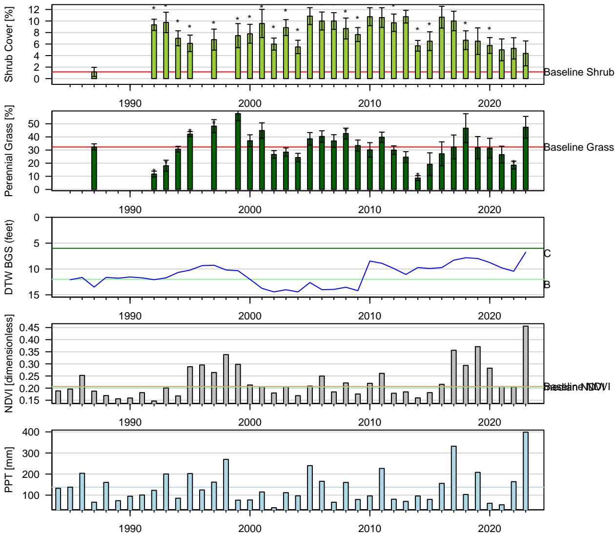
Figure 110: Two-Sample t-Test: Baseline (1pt) vs. reinventory (* p < 0.05 ). Baseline sample size ( n = 6 ). Current year sample size ( n = 8 ). Error bars = 95% CI.
