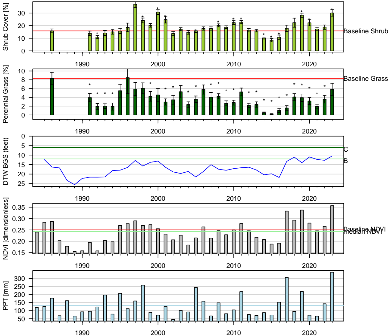
Figure 5: Two-Sample t-Test: Baseline (1pt) vs. reinventory (* p < 0.05 ). Baseline sample size ( n = 6 ). Current year sample size ( n = 12 ). Error bars = 95% CI.
