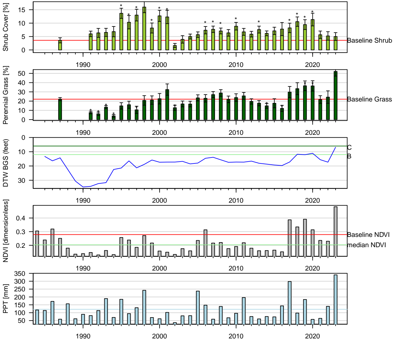
Figure 92: Two-Sample t-Test: Baseline (lpt) vs. reinventory (* p < 0.05 ).
