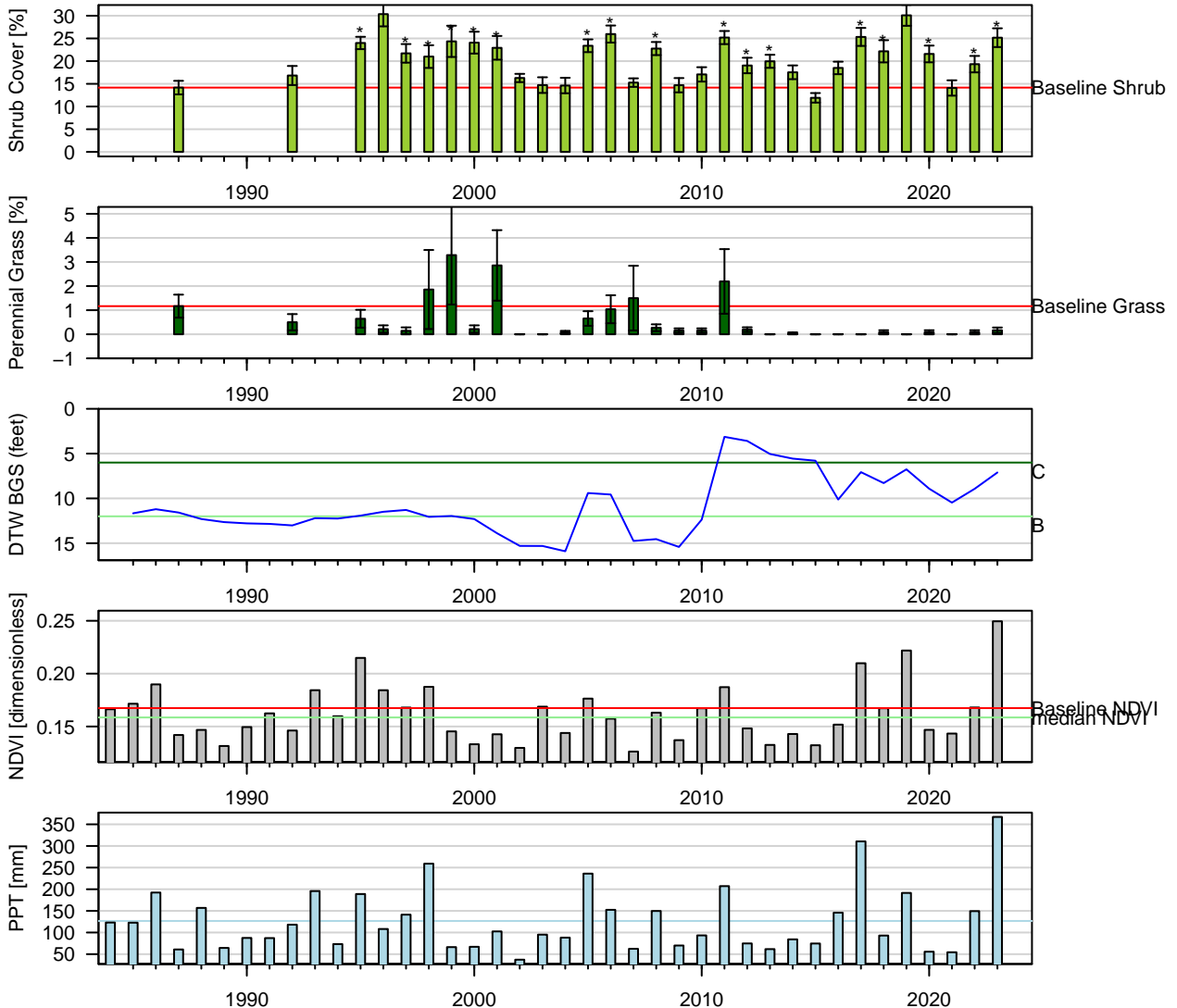
Figure 109: Two-Sample t-Test: Baseline (1pt) vs. reinventory (* p < 0.05 ). Baseline sample size ( n = 6 ). Current year sample size ( n = 12 ). Error bars = 95% CI.
