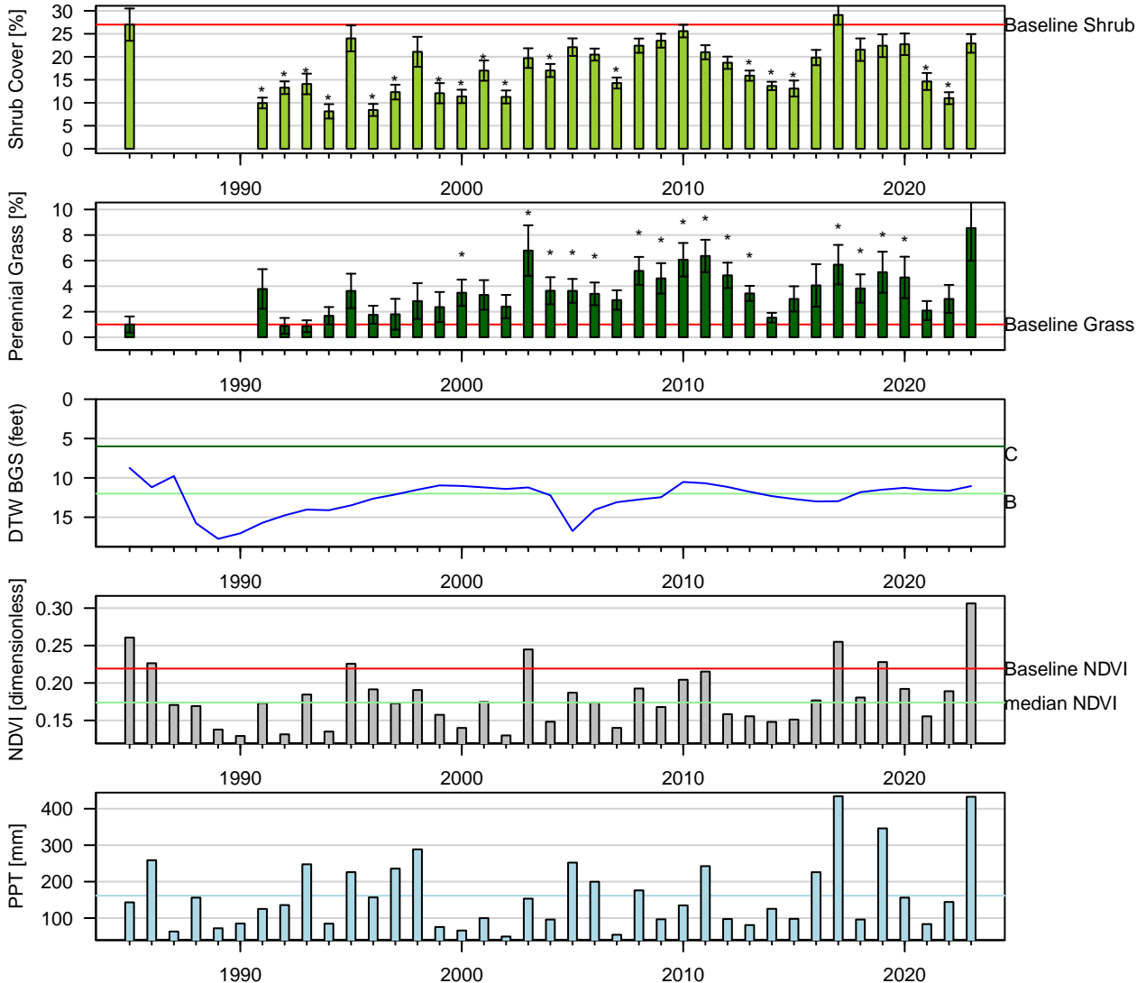
Figure 100: Two-Sample t-Test: Baseline (1pt) vs. reinventory (* p < 0.05 ). Baseline sample size ( n = 8 ). Current year sample size ( n = 22 ). Error bars = 95% CI.
