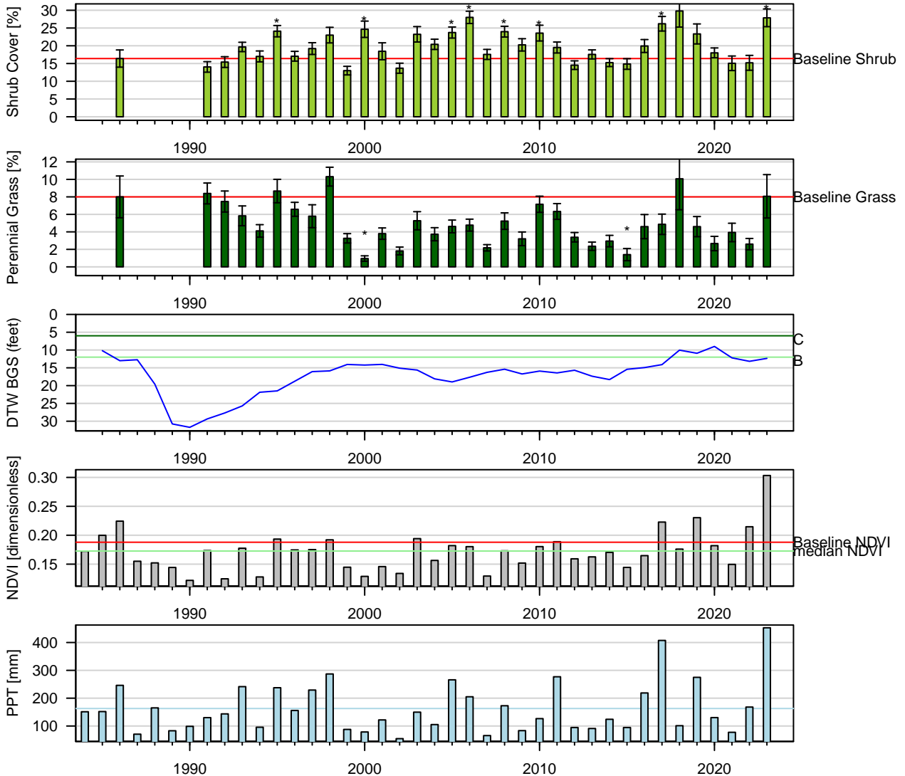
Figure 16: Two-Sample t-Test: Baseline (1pt) vs. reinventory (* p < 0.05 ). Baseline sample size ( n = 5 ). Current year sample size ( n = 15 ). Error bars = 95% CI.
