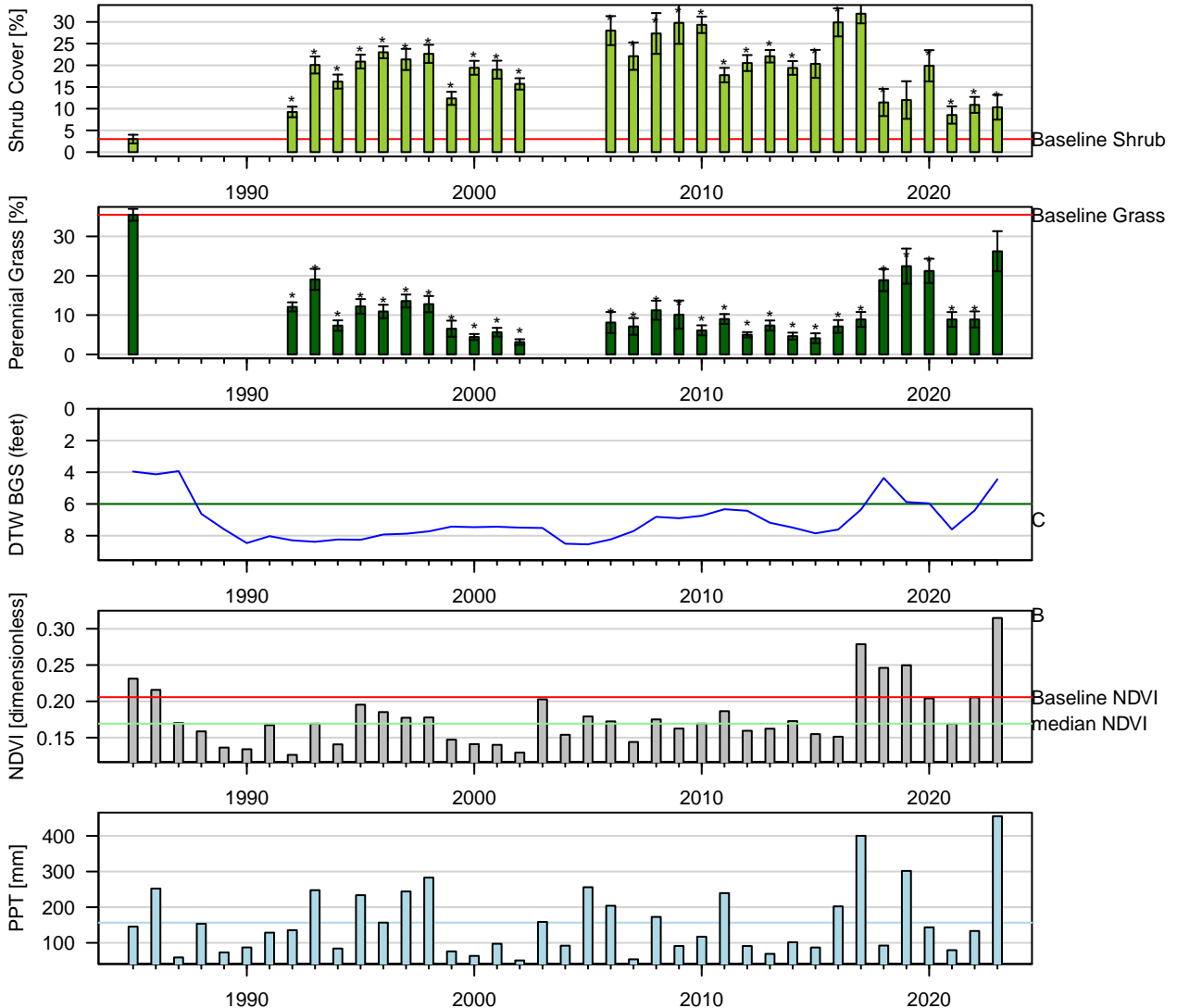
Figure 62: One-Sample t-Test: Baseline (1pt) vs. reinventory (* p < 0.05). Baseline sample size (n = 2). Current year sample size (n = 9). Error bars = 95% CI.
