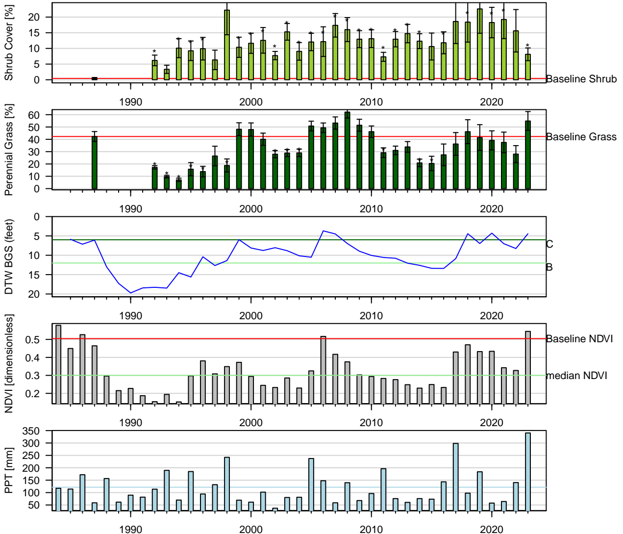
Figure 89: Two-Sample t-Test: Baseline (1pt) vs. reinventory (* p < 0.05 ). Baseline sample size ( n = 7 ). Current year sample size ( n = 8 ). Error bars = 95% CI.
