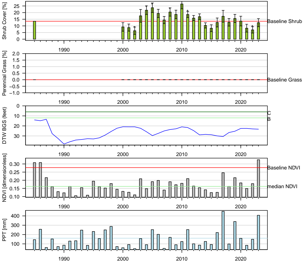
Figure 71: One-Sample t-Test: Baseline (wvcom) vs. reinventory (* p < 0.05 ). Baseline sample size ( n = 1 ). Current year sample size ( n = 7 ). Error bars = 95% CI.
