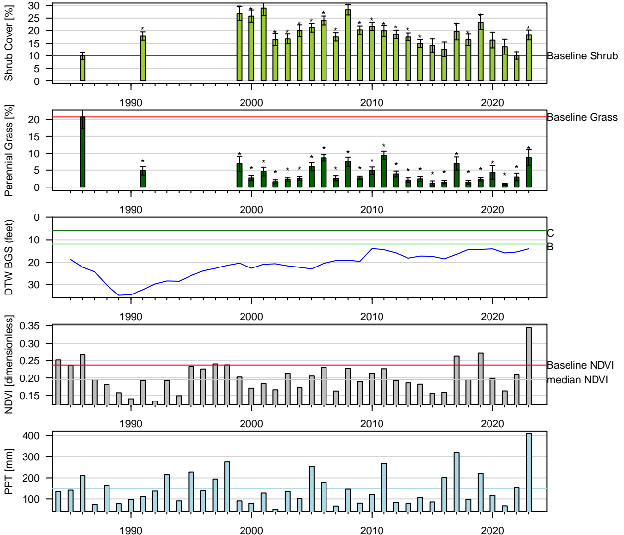
Figure 121: One-Sample t-Test: Baseline (1pt) vs. reinventory (* p < 0.05). Baseline sample size (n = 4). Current year sample size (n = 8). Error bars = 95% CI.
