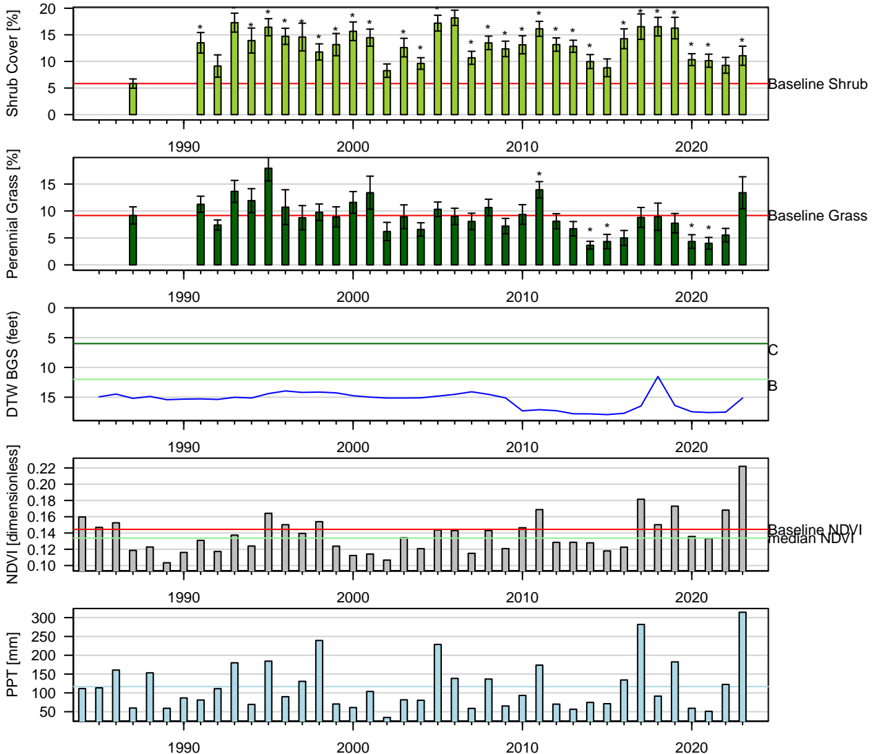
Figure 116: Two-Sample t-Test: Baseline (1pt) vs. reinventory (* p < 0.05 ). Baseline sample size ( n = 6 ). Current year sample size ( n = 15 ). Error bars = 95% CI.
