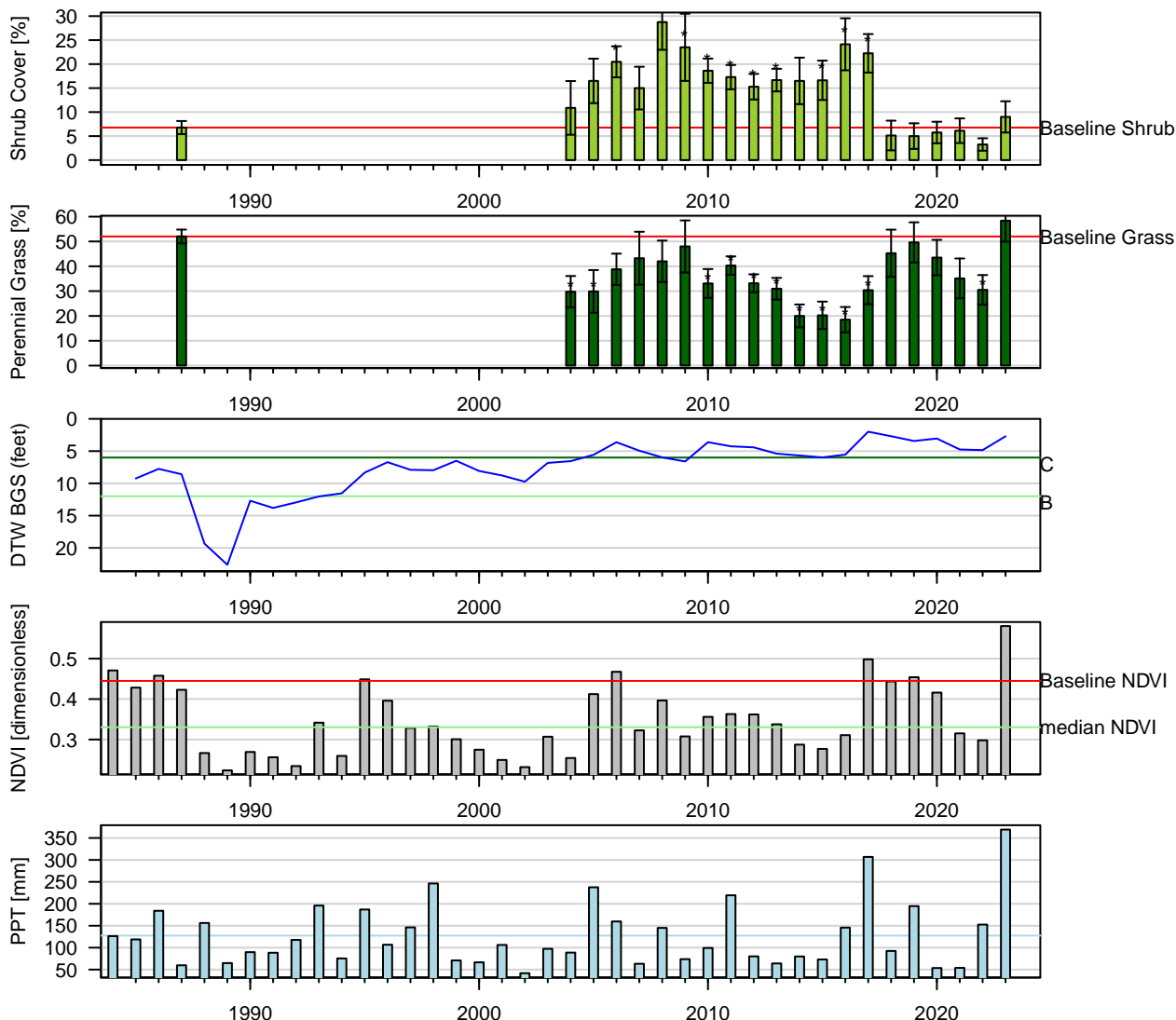
Figure 33: Two-Sample t-Test: Baseline (lpt) vs. reinventory (* p < 0.05 ). Baseline sample size ( n = 9 ). Current year sample size ( n = 8 ). Error bars = 95% CI.
