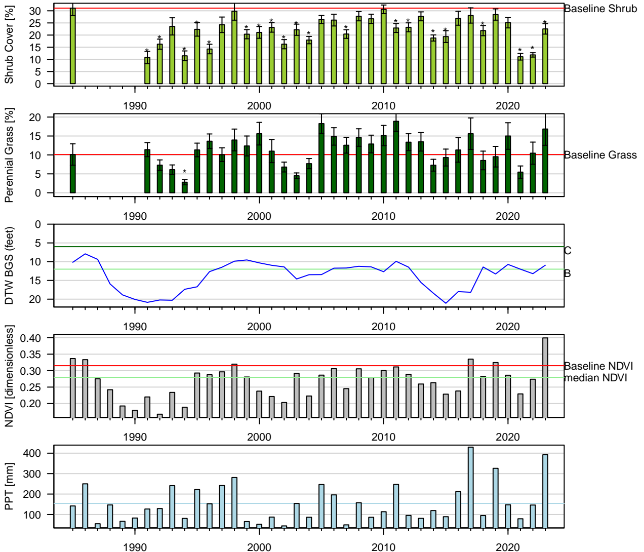
Figure 67: Two-Sample t-Test: Baseline (lpt) vs. reinventory (* p < 0.05 ). Baseline sample size (n = 10). Current year sample size (n = 13). Error bars = 95% CI.
