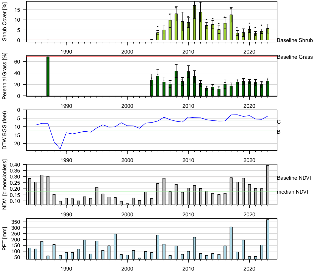
Figure 31: Two-Sample t-Test: Baseline (1pt) vs. reinventory (* p < 0.05 ). Baseline sample size ( n = 6 ). Current year sample size ( n = 6 ). Error bars = 95% CI.
