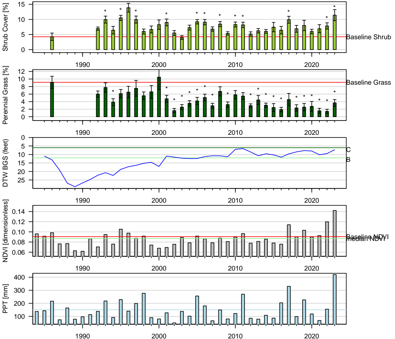
Figure 122: Two-Sample t-Test: Baseline (1pt) vs. reinventory (* p < 0.05 ). Baseline sample size ( n = 8 ). Current year sample size ( n = 12 ). Error bars = 95% CI.
