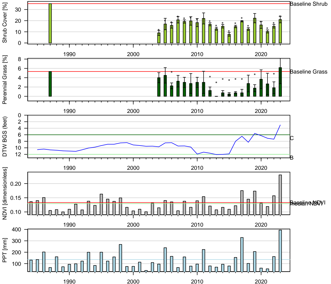
Figure 112: One-Sample t-Test: Baseline (wvcom) vs. reinventory (* p < 0.05). Baseline sample size (n = 1). Current year sample size (n = 6). Error bars = 95% CI.
