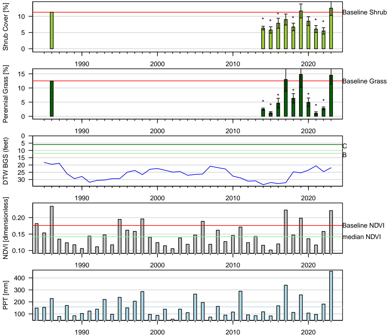
Figure 53: One-Sample t-Test: Baseline (wvcom) vs. reinventory (* p < 0.05 ). Baseline sample size ( n = 1 ). Current year sample size ( n = 14 ). Error bars = 95% CI.
