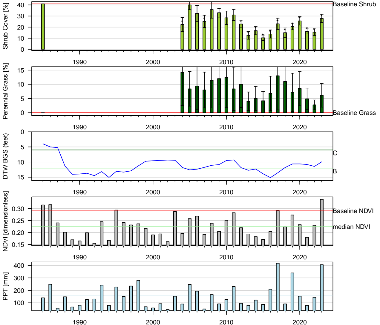
Figure 69: One-Sample t-Test: Baseline (1pt) vs. reinventory (* p < 0.05 ). Baseline sample size ( n = 1 ). Current year sample size ( n = 8 ). Error bars = 95% CI.
