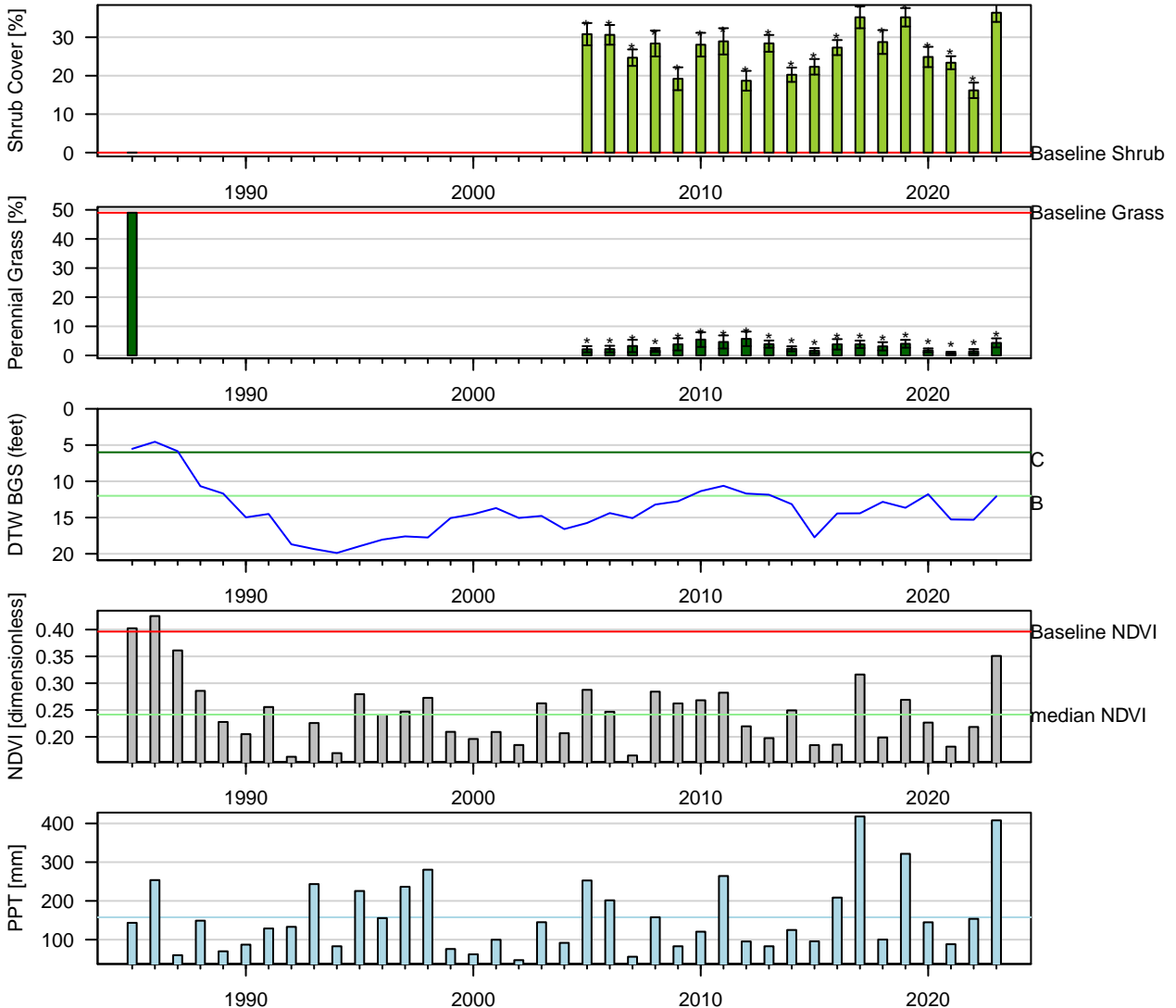
Figure 59: One-Sample t-Test: Baseline (1pt) vs. reinventoried (* p < 0.05 ). Baseline sample size ( n = 1 ). Current year sample size ( n = 16 ). Error bars = 95% CI.
