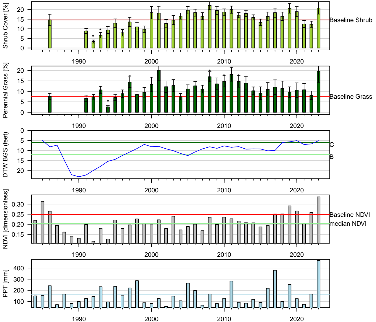
Figure 14: Two-Sample t-Test: Baseline (lpt) vs. reinventory (* p < 0.05 ). Baseline sample size ( n = 10 ). Current year sample size ( n = 16 ). Error bars = 95% CI.
