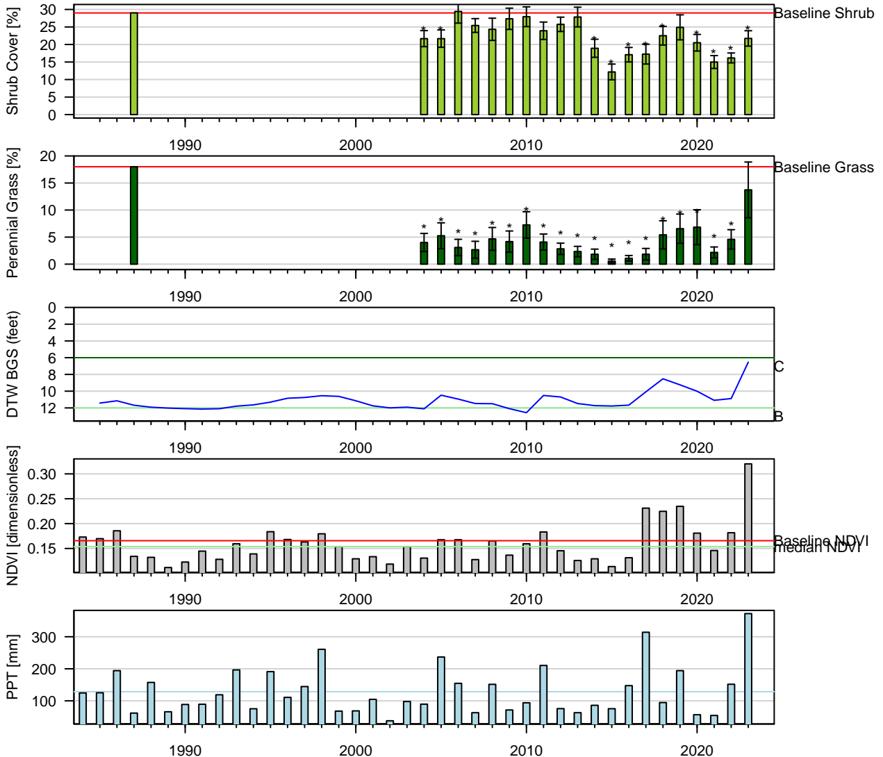
Figure 108: One-Sample t-Test: Baseline (wvcom) vs. reinventory (* p < 0.05). Baseline sample size (n = 1). Current year sample size (n = 11). Error bars = 95% CI.
