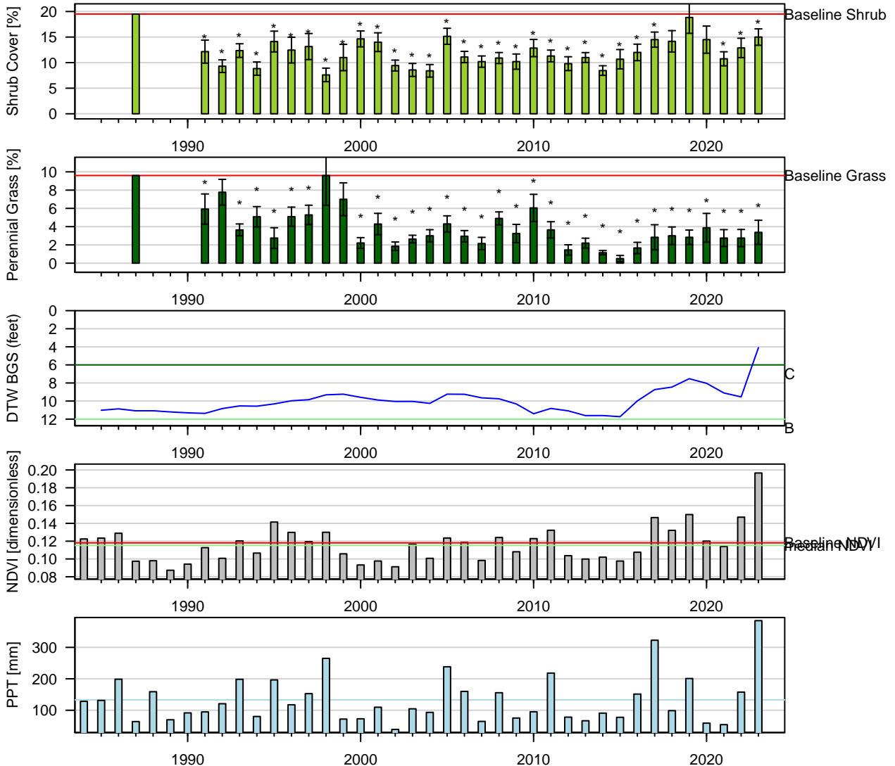
Figure 111: One-Sample t-Test: Baseline (wvcom) vs. reinventory (* p < 0.05 ). Baseline sample size ( n = 1 ). Current year sample size ( n = 8 ). Error bars = 95% CI.
