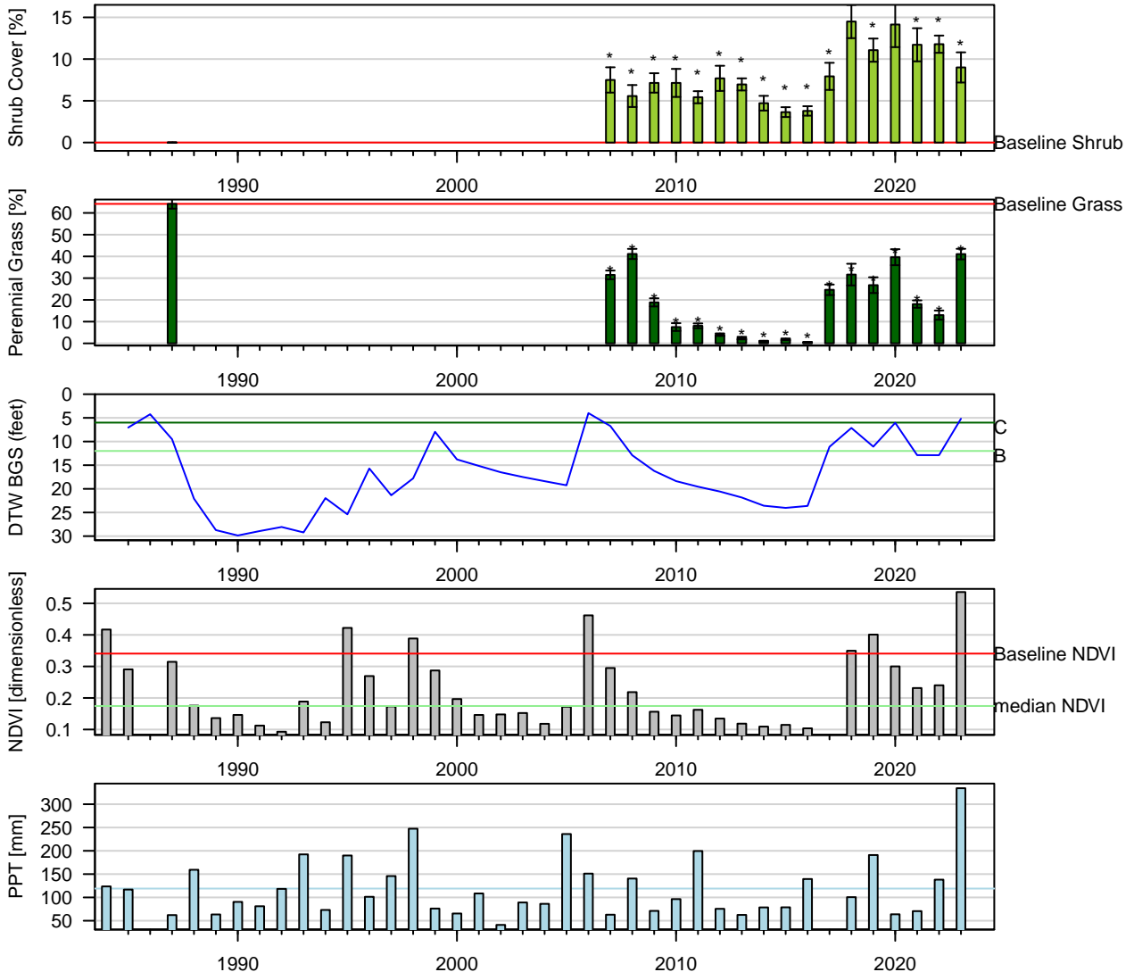
Figure 84: Two-Sample t-Test: Baseline (lpt) vs. reinventory (* p < 0.05 ).
