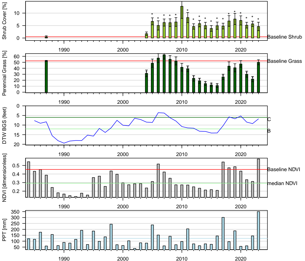
Figure 90: Two-Sample t-Test: Baseline (1pt) vs. reinventory (* p < 0.05 ).
