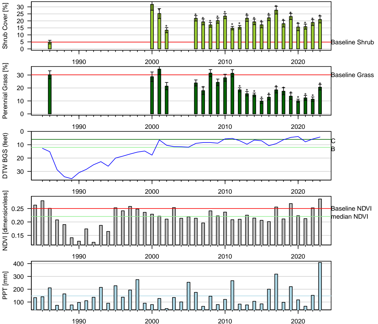
Figure 120: Two-Sample t-Test: Baseline (1pt) vs. reinventory (* p < 0.05 ). Baseline sample size ( n = 6 ). Current year sample size ( n = 16 ). Error bars = 95% CI.
