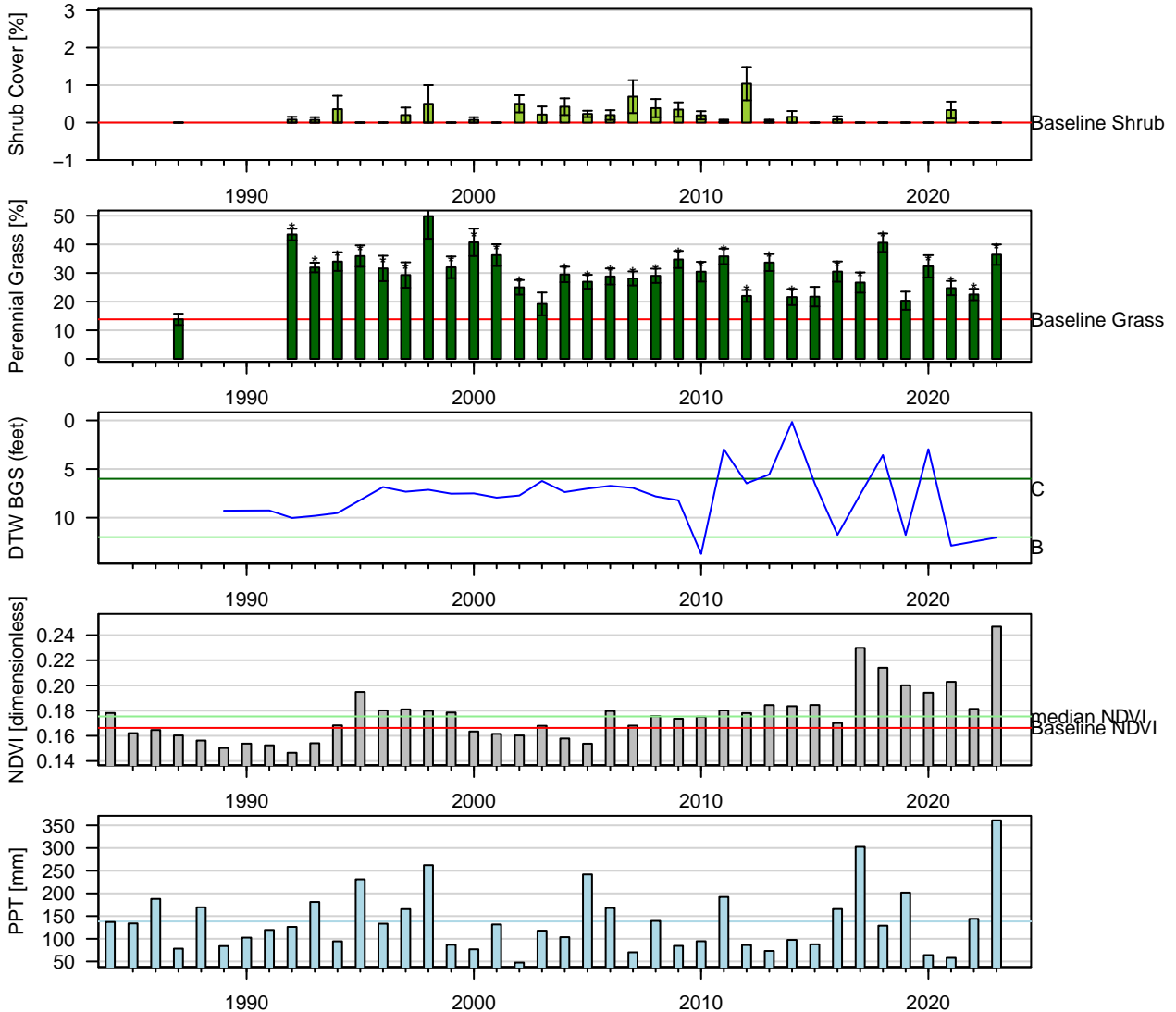
Figure 50: Two-Sample t-Test: Baseline (lpt) vs. reinventory (* p < 0.05 ). Baseline sample size ( n = 12 ). Current year sample size ( n = 12 ). Error bars = 95% CI.
