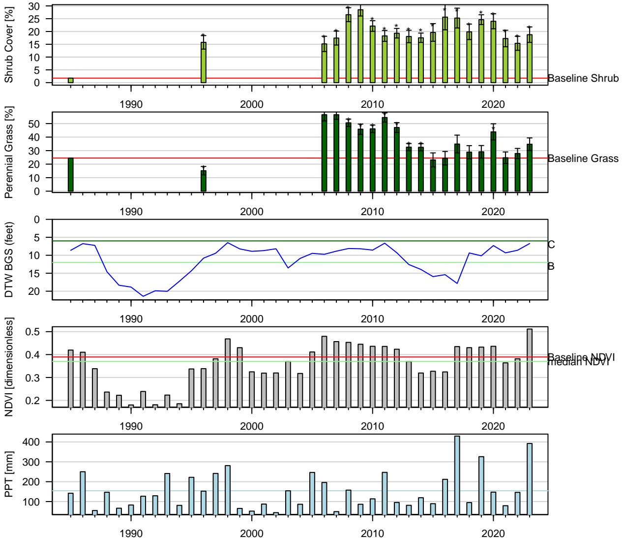
Figure 74: One-Sample t-Test: Baseline (wvcom) vs. reinventory (* p < 0.05). Baseline sample size (n = 1). Current year sample size (n = 8). Error bars = 95% CI.
