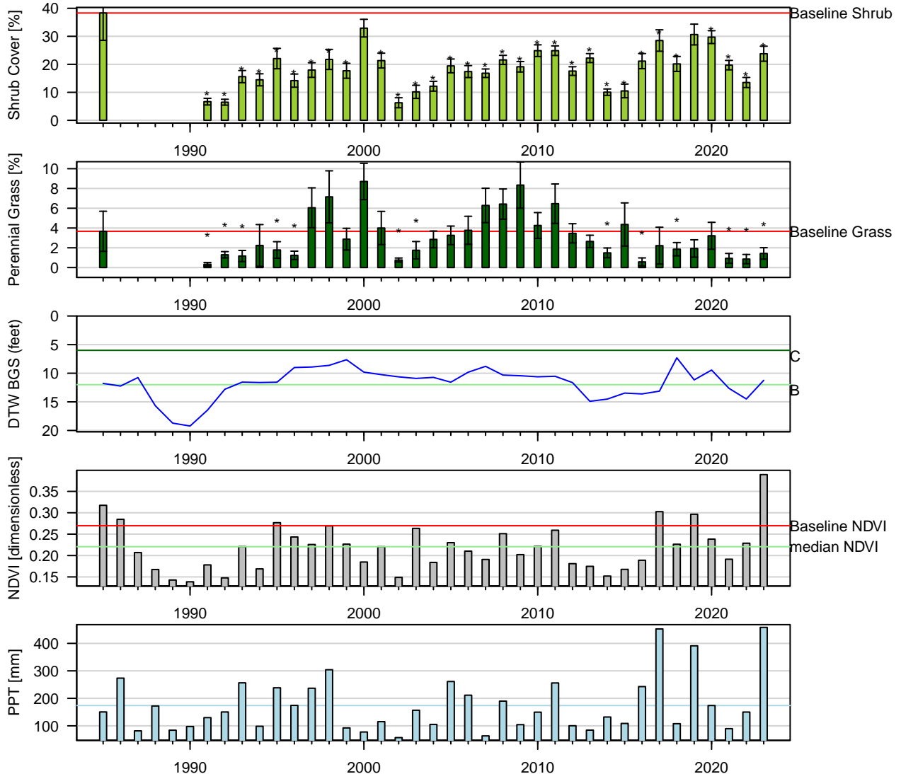
Figure 103: One-Sample t-Test: Baseline (1pt) vs. reinventory (* p < 0.05 ). Baseline sample size ( n = 3 ). Current year sample size ( n = 14 ). Error bars = 95% CI.
