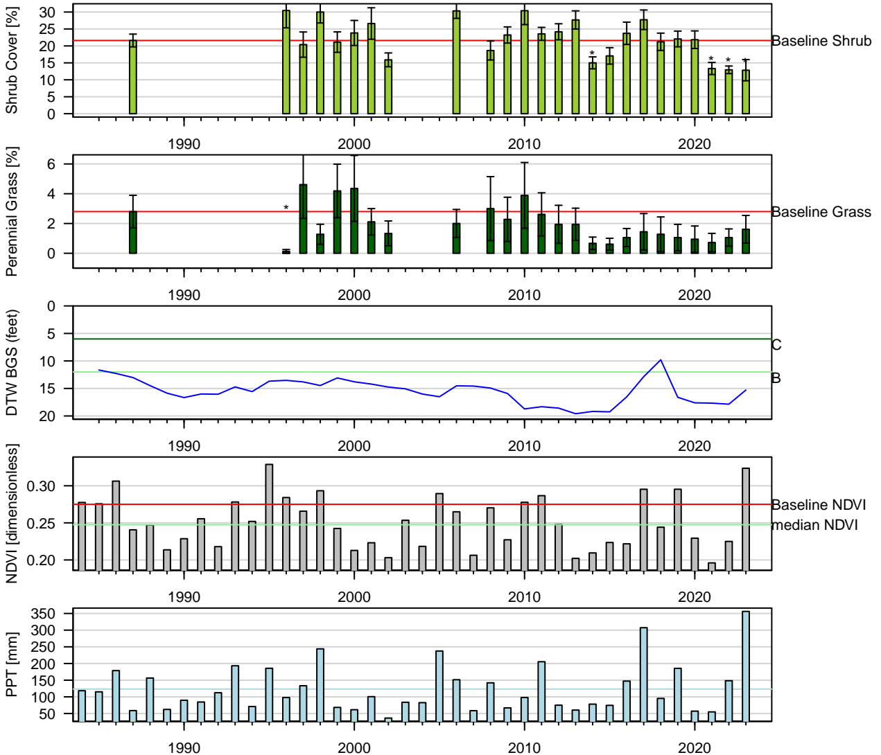
Figure 106: Two-Sample t-Test: Baseline (1pt) vs. reinventory (* p < 0.05 ).
