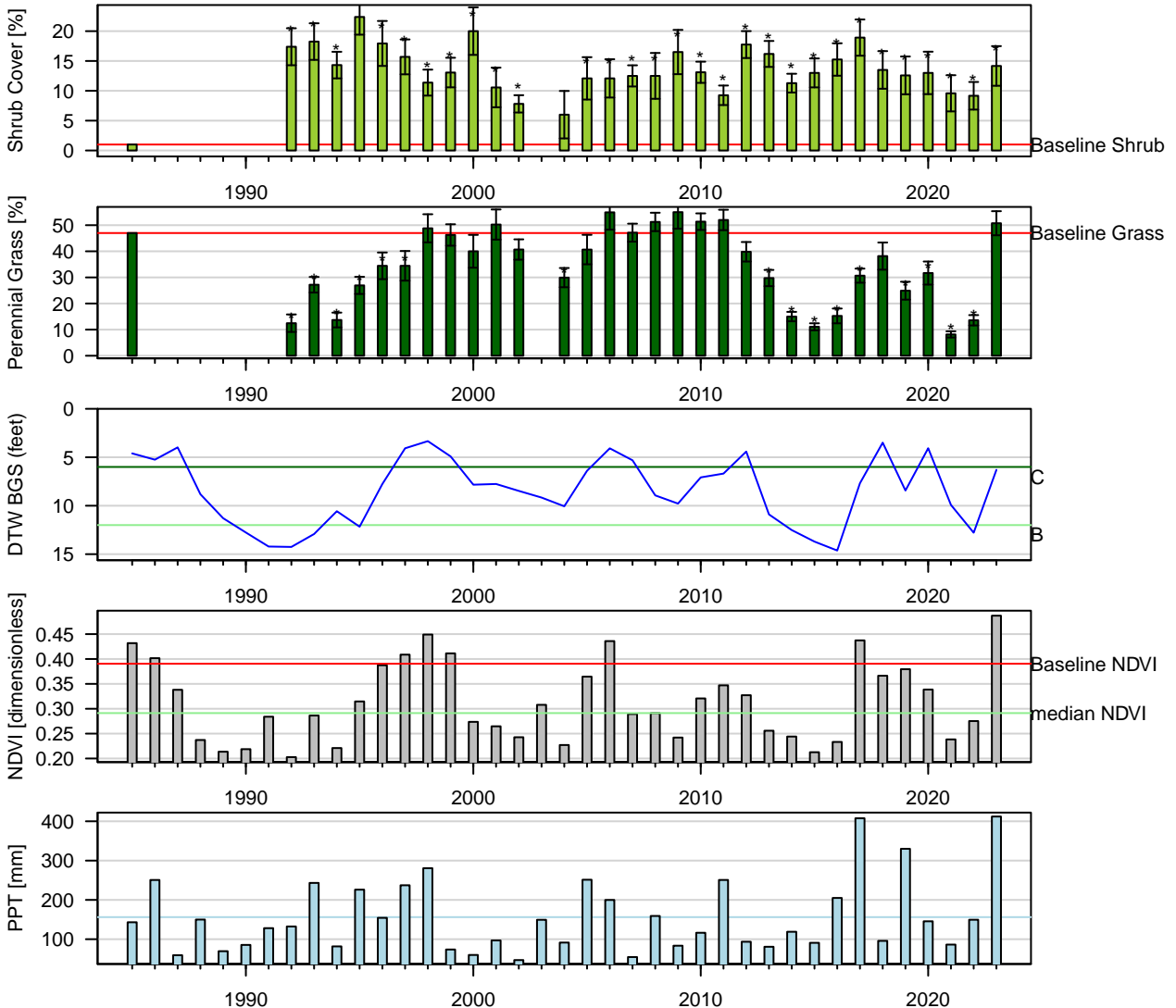
Figure 56: One-Sample t-Test: Baseline (1pt) vs. reinventory (* p < 0.05 ).
