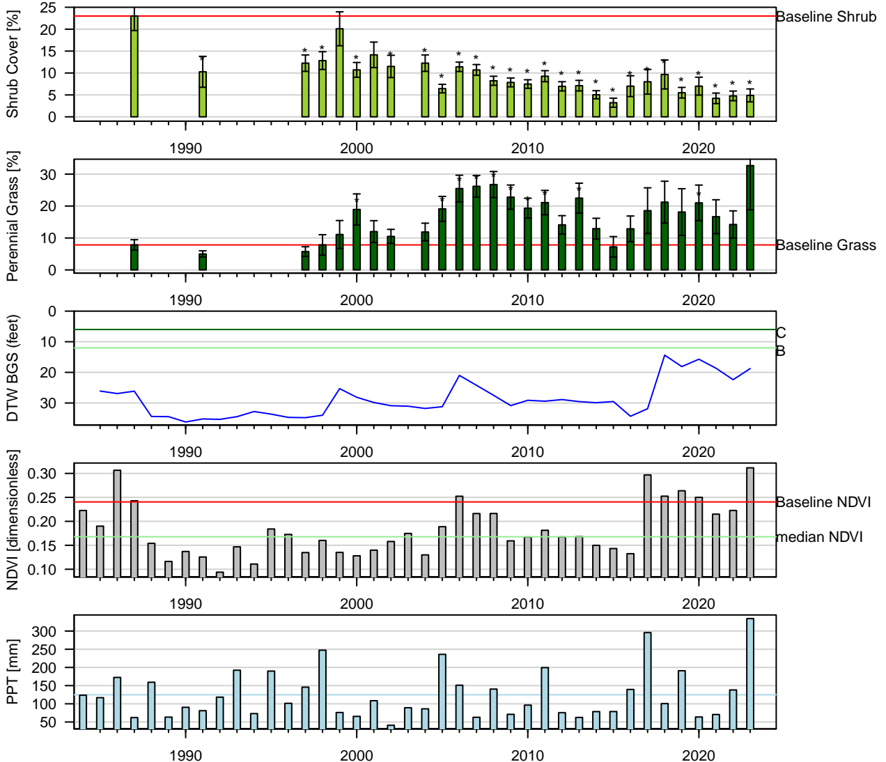
Figure 76: Two-Sample t-Test: Baseline (lpt) vs. reinventory (* p < 0.05 ).
