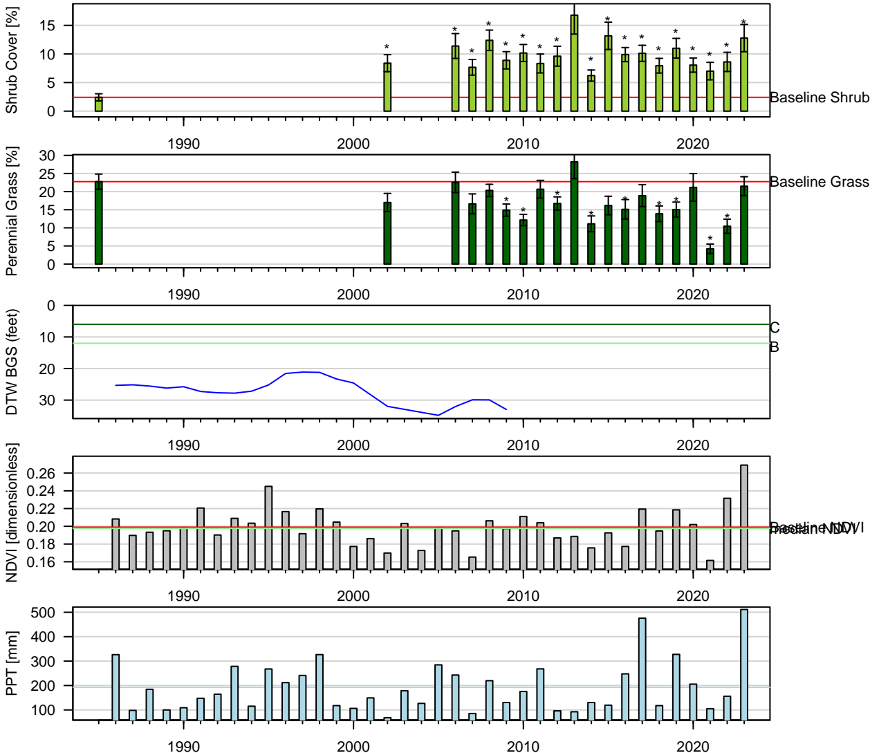
Figure 98: Two-Sample t-Test: Baseline (lpt) vs. reinventory (* p < 0.05 ). Baseline sample size ( n = 12 ). Current year sample size ( n = 18 ). Error bars = 95% CI.
