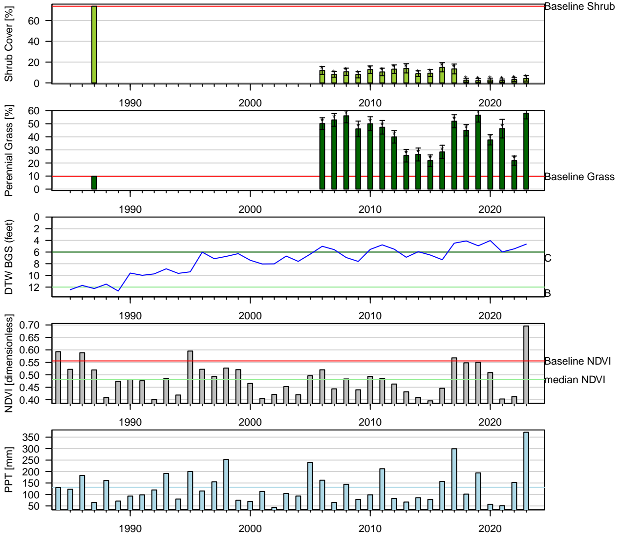
Figure 34: One-Sample t-Test: Baseline (wvcom) vs. reinventory (* p < 0.05 ). Baseline sample size ( n = 1 ). Current year sample size ( n = 12 ). Error bars = 95% CI.
