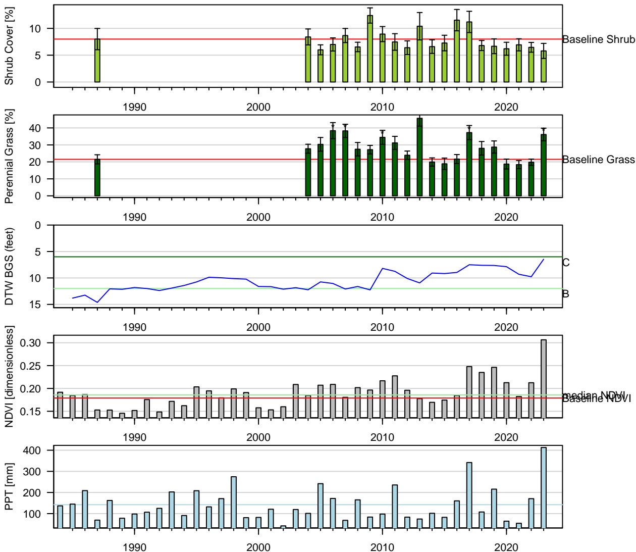
Figure 115: Two-Sample t-Test: Baseline (1pt) vs. reinventory (* p < 0.05 ). Baseline sample size (n = 6). Current year sample size (n = 15). Error bars = 95% CI.
