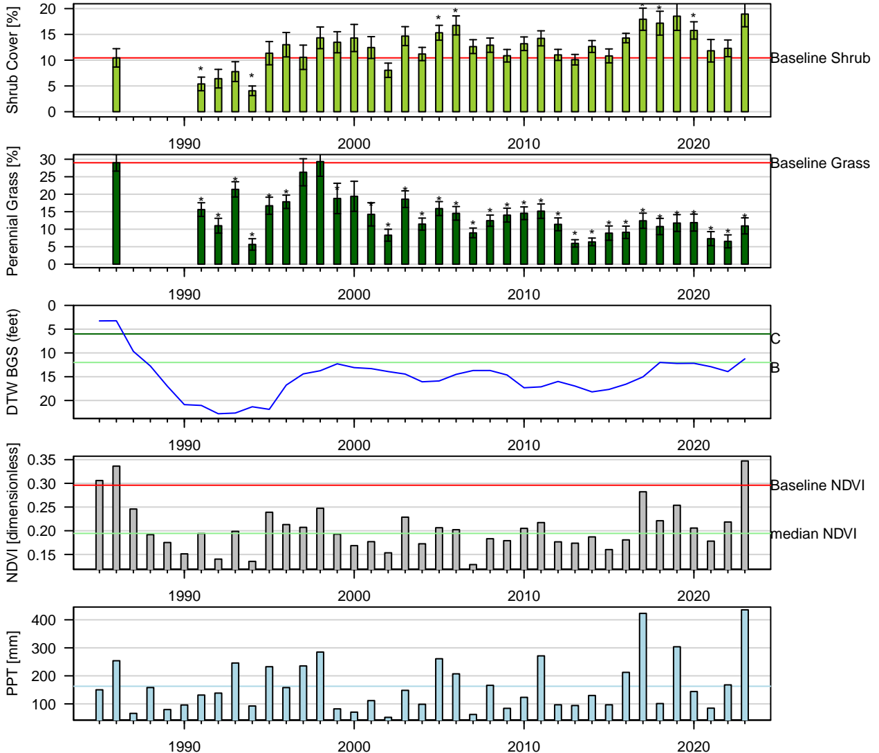
Figure 24: Two-Sample t-Test: Baseline (lpt) vs. reinventory (* p < 0.05 ).
