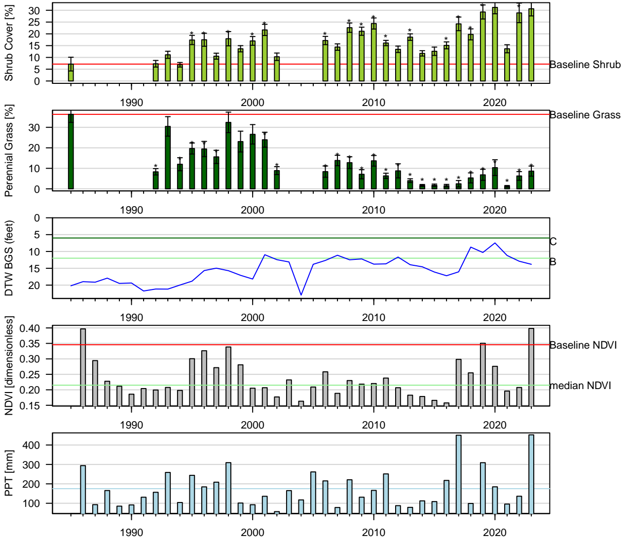
Figure 97: Two-Sample t-Test: Baseline (1pt) vs. reinventory (* p < 0.05 ).
