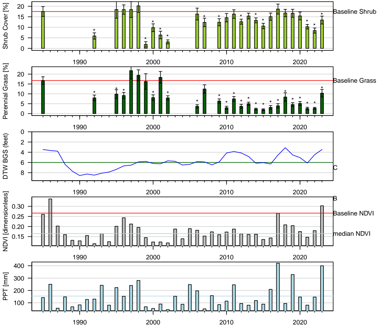
Figure 63: One-Sample t-Test: Baseline (1pt) vs. reinventory (* p < 0.05 ). Baseline sample size (n = 4). Current year sample size (n = 18). Error bars = 95% CI.
