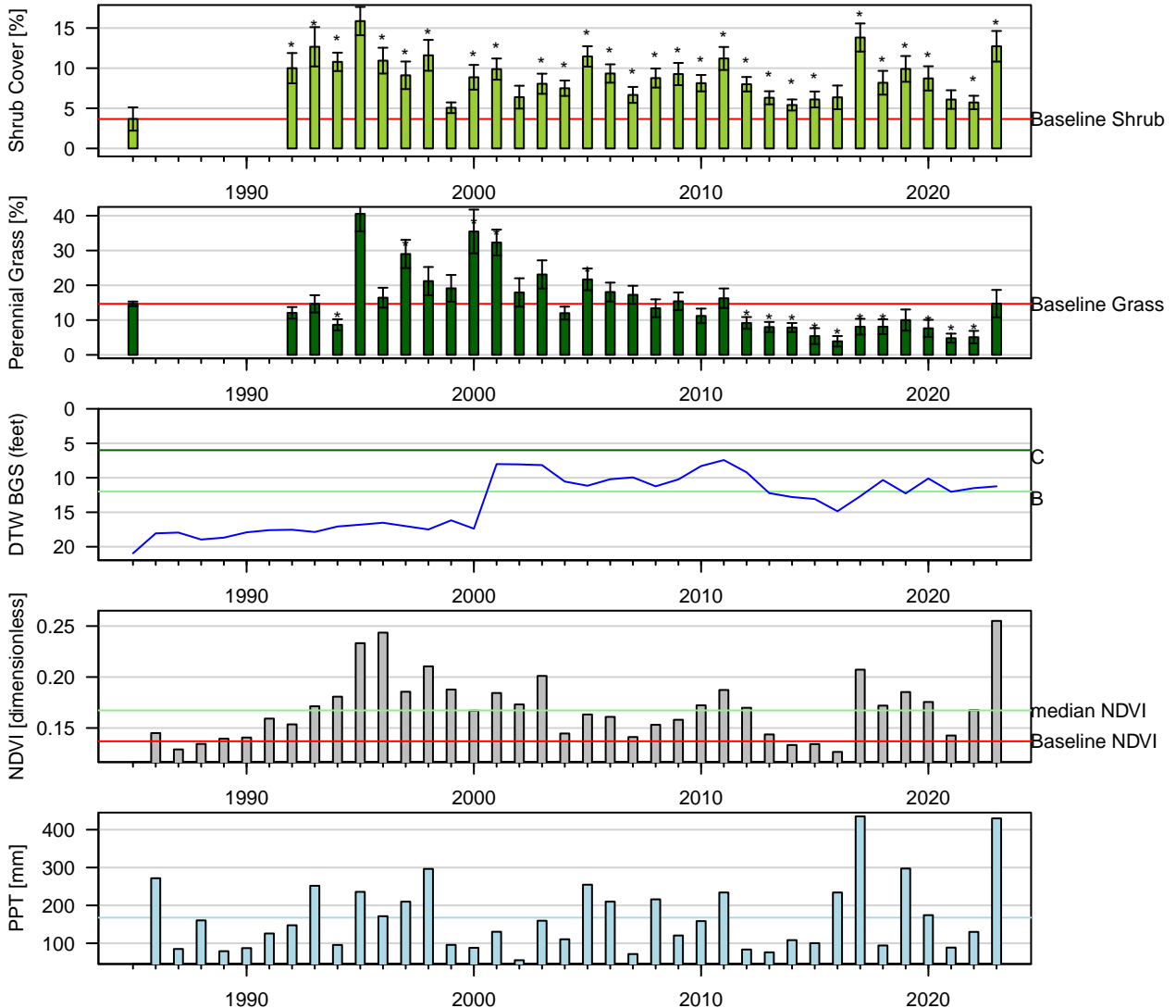
Figure 95: One-Sample t-Test: Baseline (1pt) vs. reinventory (* p < 0.05 ). Baseline sample size ( n = 3 ). Current year sample size ( n = 11 ). Error bars = 95% CI.
