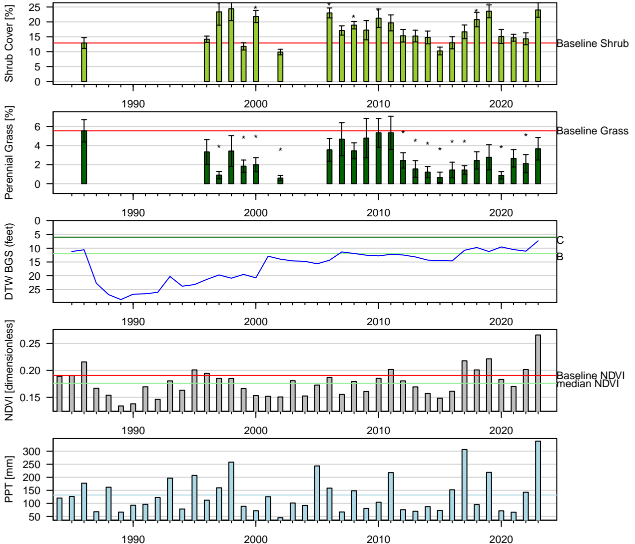
Figure 3: Two-Sample t-Test: Baseline (1pt) vs. reinventory (* p < 0.05 ).
