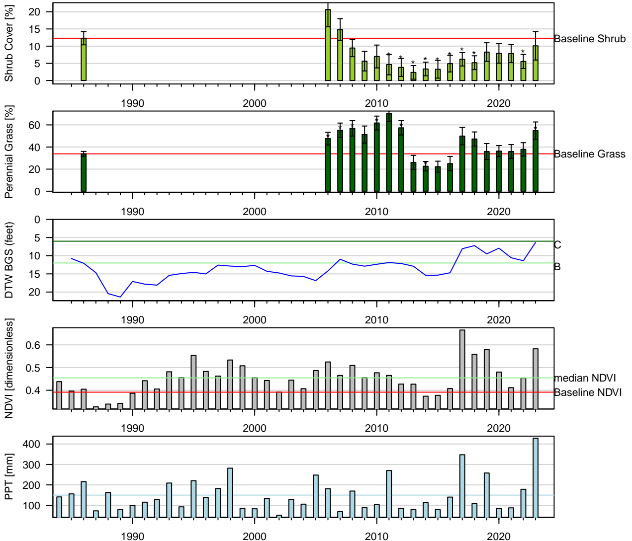
Figure 4: Two-Sample t-Test: Baseline (1pt) vs. reinventory (* p < 0.05 ). Baseline sample size ( n = 13 ). Current year sample size ( n = 11 ). Error bars = 95% CI.
