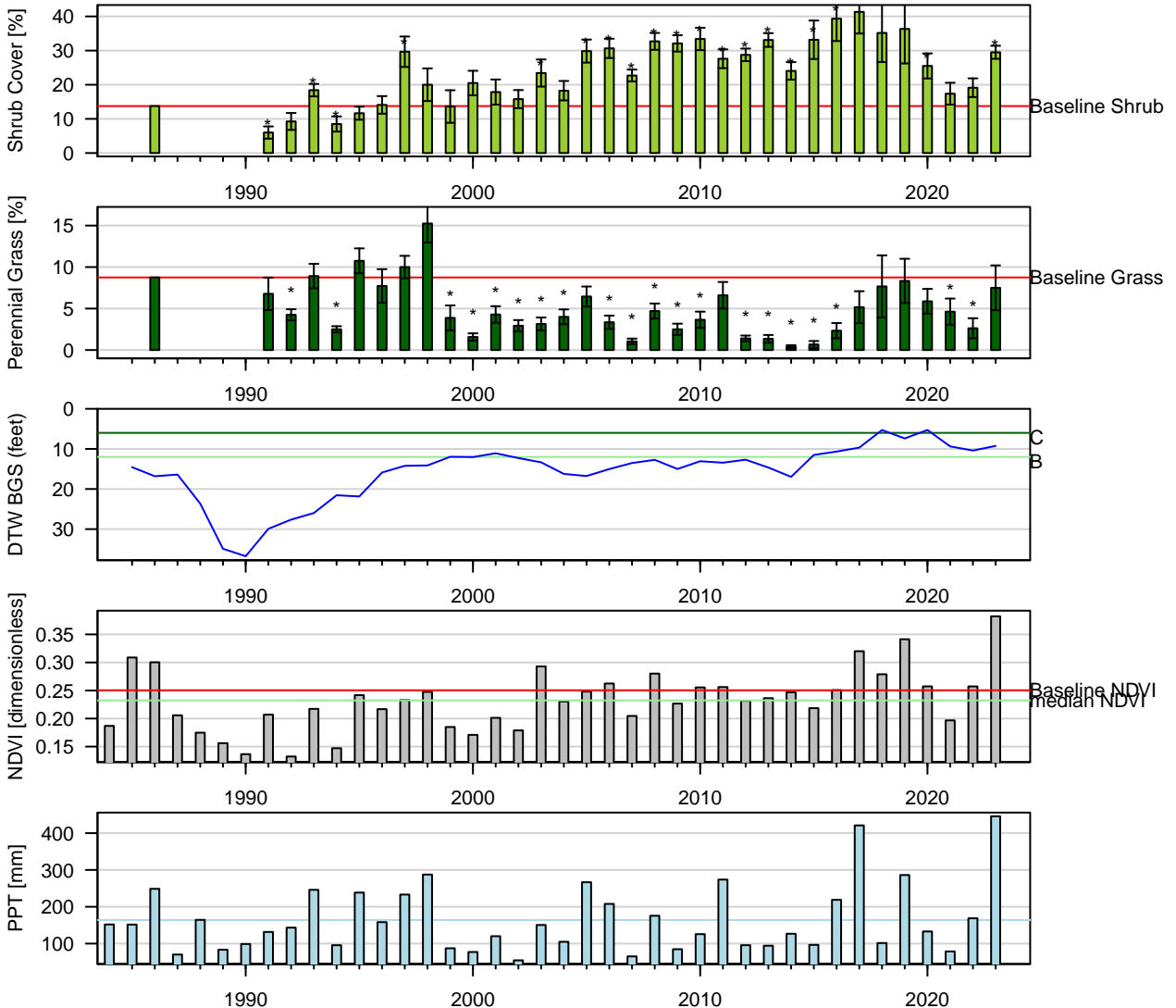
Figure 19: One-Sample t-Test: Baseline (wvcom) vs. reinventory (* p < 0.05 ). Baseline sample size ( n = 1 ). Current year sample size ( n = 8 ). Error bars = 95% CI.
