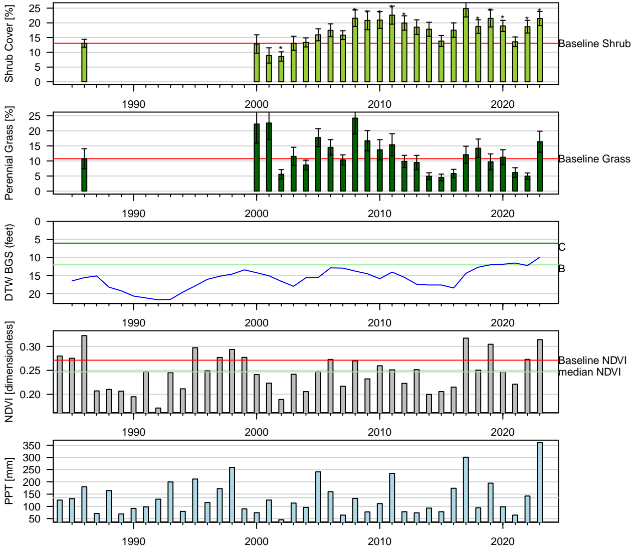
Figure 118: Two-Sample t-Test: Baseline (1pt) vs. reinventory (* p < 0.05 ). Baseline sample size ( n = 12 ). Current year sample size ( n = 24 ). Error bars = 95% CI.
