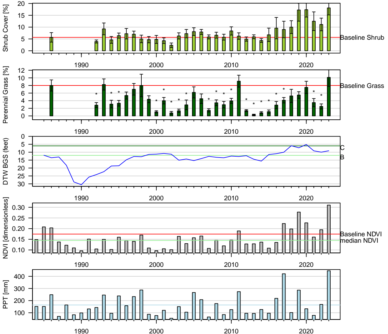
Figure 17: Two-Sample t-Test: Baseline (lpt) vs. reinventory (* p < 0.05 ).
