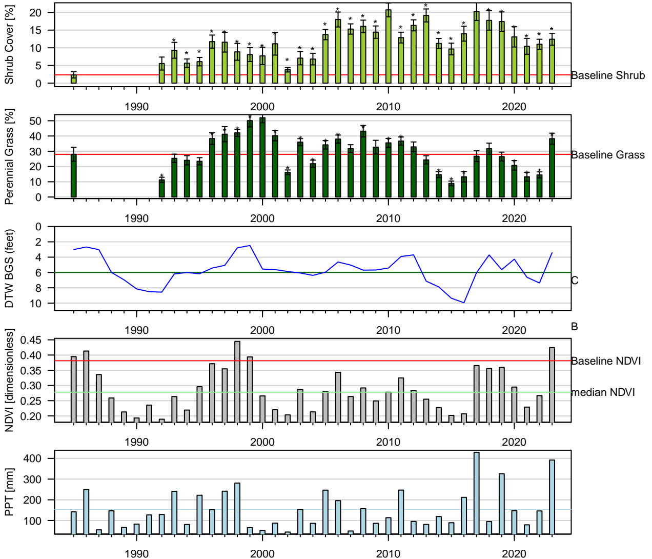
Figure 55: One-Sample t-Test: Baseline (lpt) vs. reinventory (* p < 0.05 ). Baseline sample size ( n = 3 ). Current year sample size ( n = 12 ). Error bars = 95% CI.
