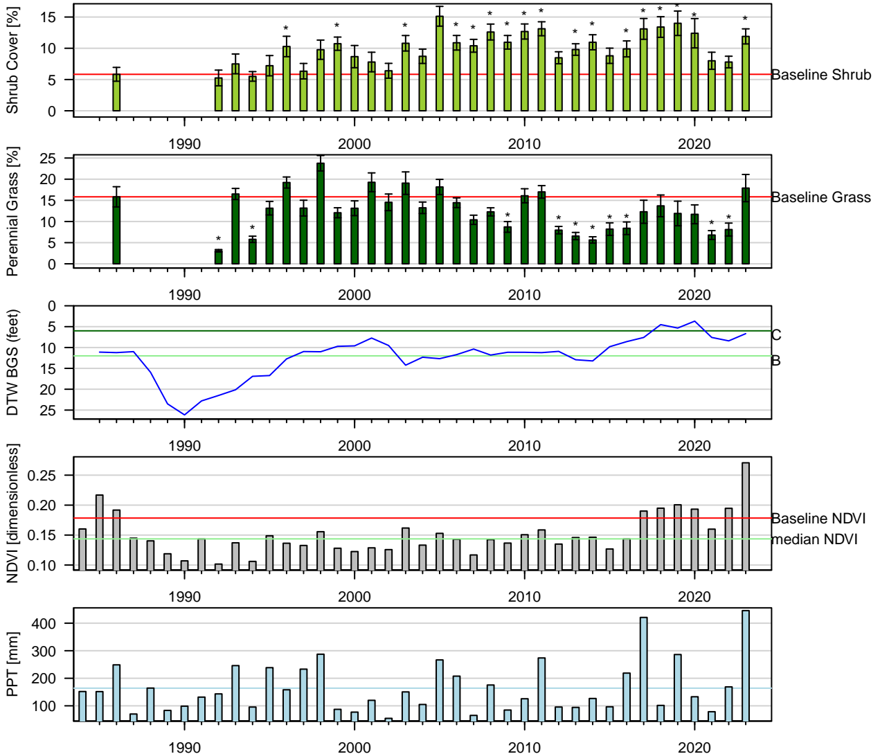
Figure 18: Two-Sample t-Test: Baseline (1pt) vs. reinventory (* p < 0.05 ). Baseline sample size ( n = 6 ). Current year sample size ( n = 10 ). Error bars = 95% CI.
