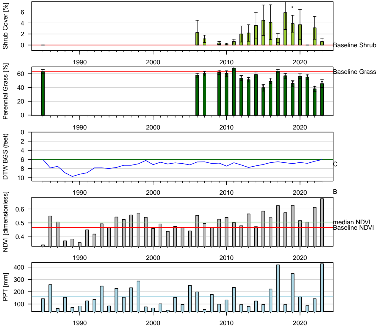
Figure 124: One-Sample t-Test: Baseline (1pt) vs. reinventory (* p < 0.05 ). Baseline sample size ( n = 2 ). Current year sample size ( n = 16 ). Error bars = 95% CI.
