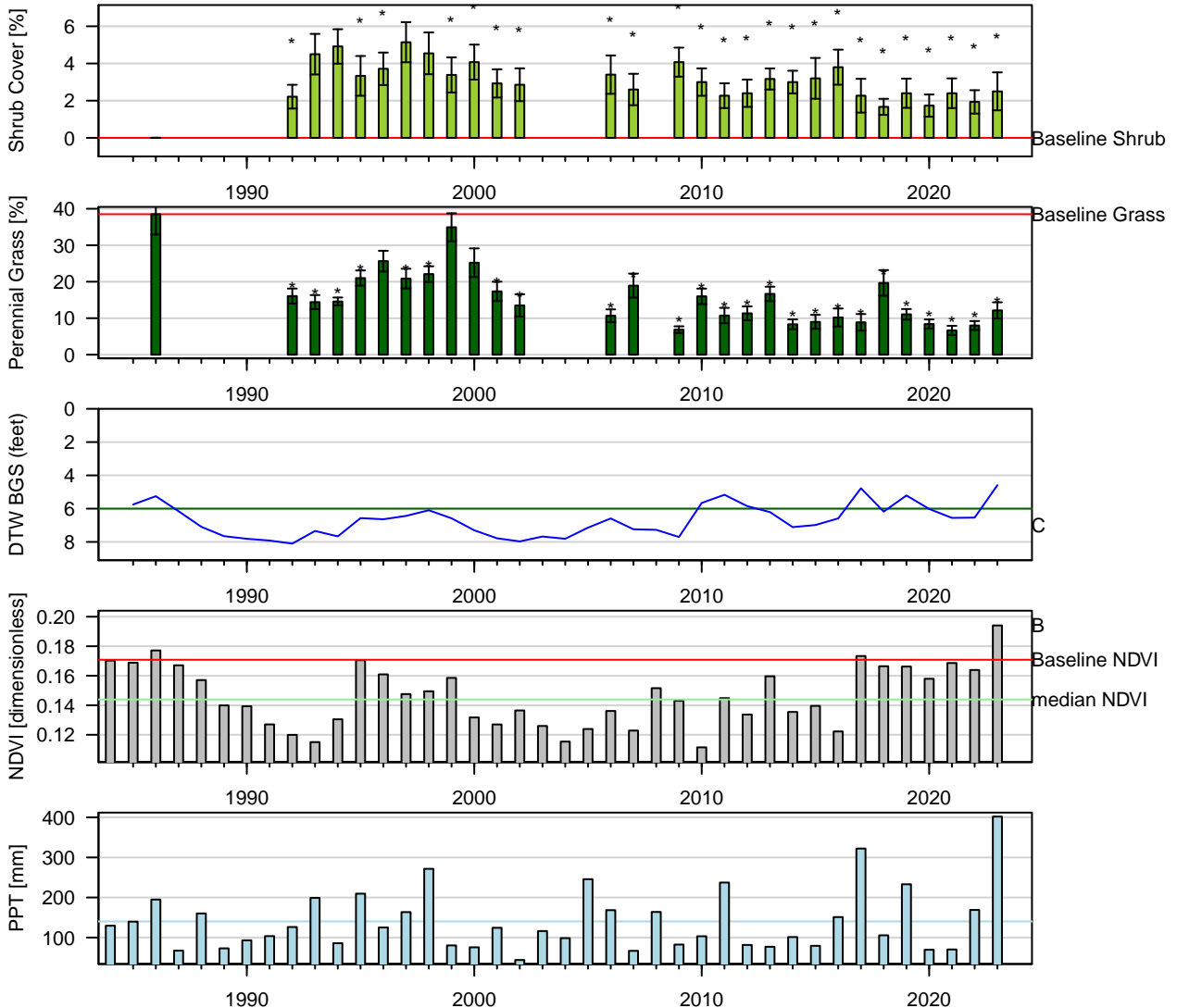
Figure 2: Two-Sample t-Test: Baseline (lpt) vs. reinventory (* p < 0.05 ). Baseline sample size ( n = 6 ). Current year sample size ( n = 14 ). Error bars = 95% CI.
