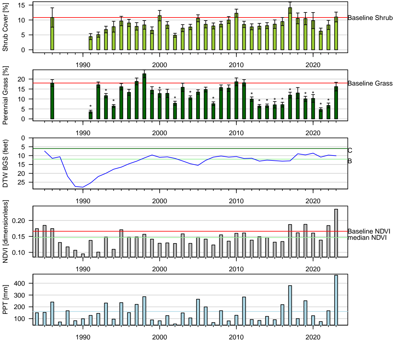
Figure 12: Two-Sample t-Test: Baseline (lpt) vs. reinventory (* p < 0.05 ). Baseline sample size ( n = 6 ). Current year sample size ( n = 15 ). Error bars = 95% CI.
