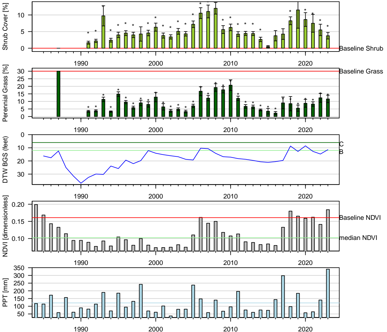
Figure 87: One-Sample t-Test: Baseline (wvcom) vs. reinventory (* p < 0.05 ). Baseline sample size ( n = 1 ). Current year sample size ( n = 8 ). Error bars = 95% CI.
