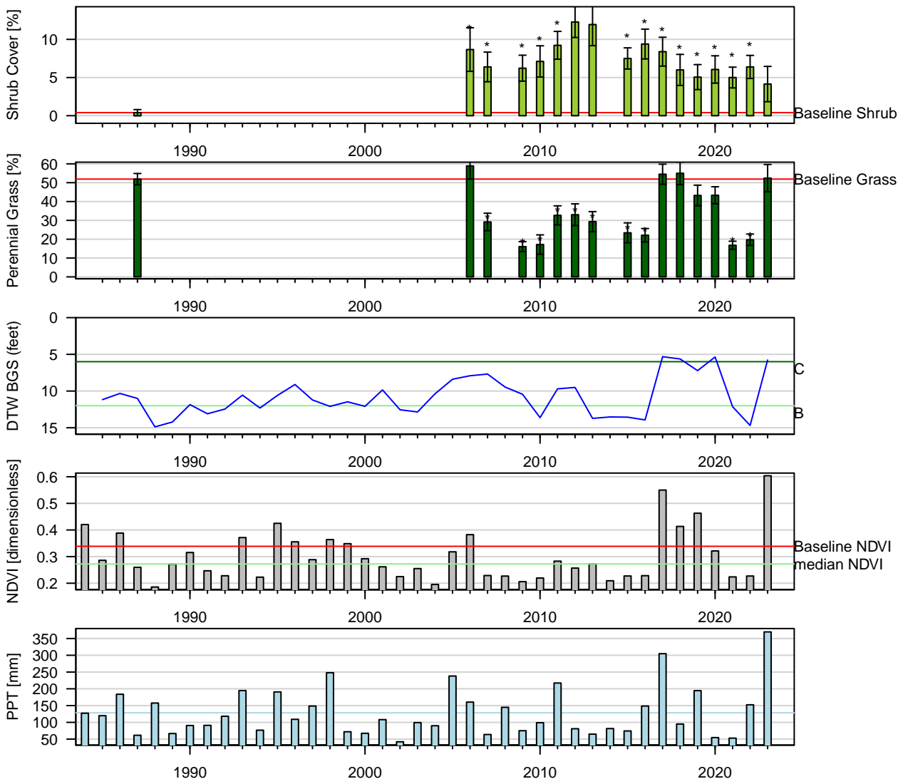
Figure 39: Two-Sample t-Test: Baseline (1pt) vs. reinventory (* p < 0.05 ).
