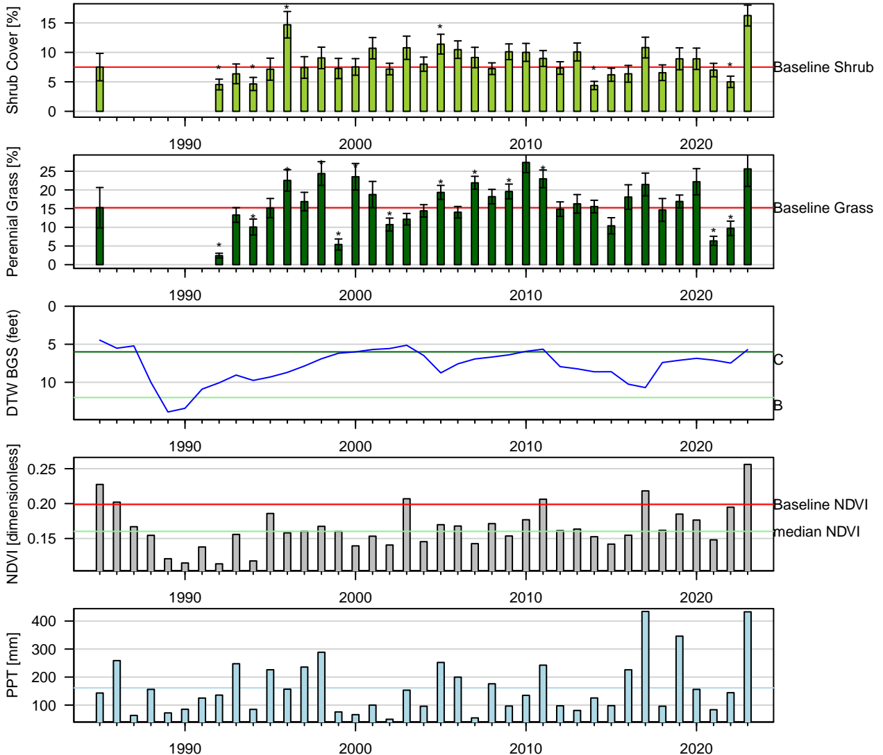
Figure 99: One-Sample t-Test: Baseline (1pt) vs. reinventory (* p < 0.05 ). Baseline sample size ( n = 4 ). Current year sample size ( n = 8 ). Error bars = 95% CI.
