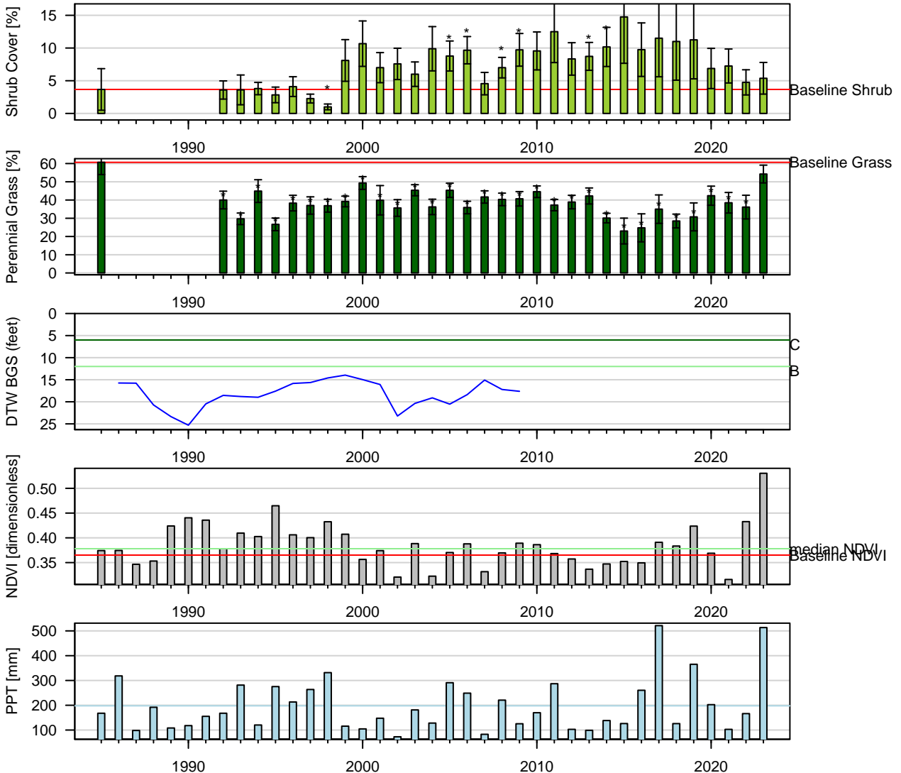
Figure 105: One-Sample t-Test: Baseline (1pt) vs. reinventory (* p < 0.05 ). Baseline sample size ( n = 3 ). Current year sample size ( n = 8 ). Error bars = 95% CI.
