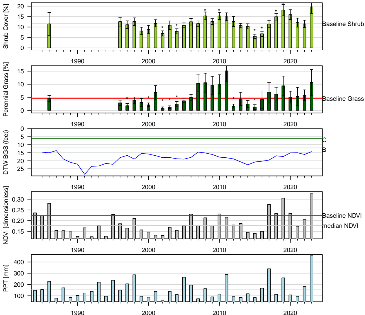
Figure 51: One-Sample t-Test: Baseline (lpt) vs. reinventory (* p < 0.05 ).
