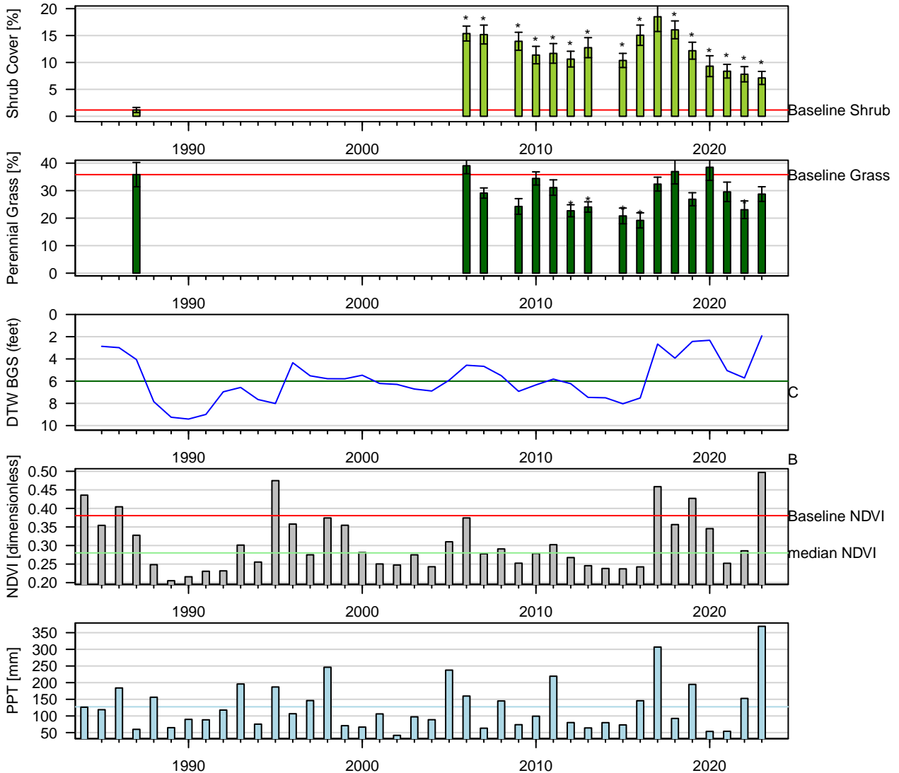
Figure 35: Two-Sample t-Test: Baseline (1pt) vs. reinventory (* p < 0.05 ).
