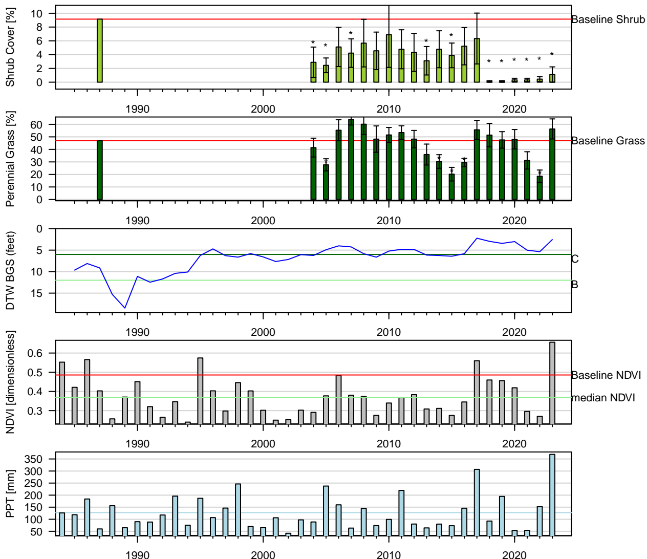
Figure 41: One-Sample t-Test: Baseline (wvcom) vs. reinventory (* p < 0.05 ). Baseline sample size ( n = 1 ). Current year sample size ( n = 9 ). Error bars = 95% CI.
