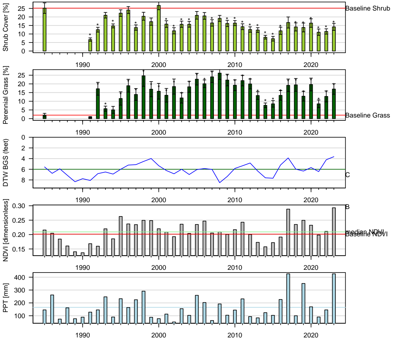
Figure 125: Two-Sample t-Test: Baseline (1pt) vs. reinventory (* p < 0.05 ). Baseline sample size ( n = 6 ). Current year sample size ( n = 23 ). Error bars = 95% CI.
