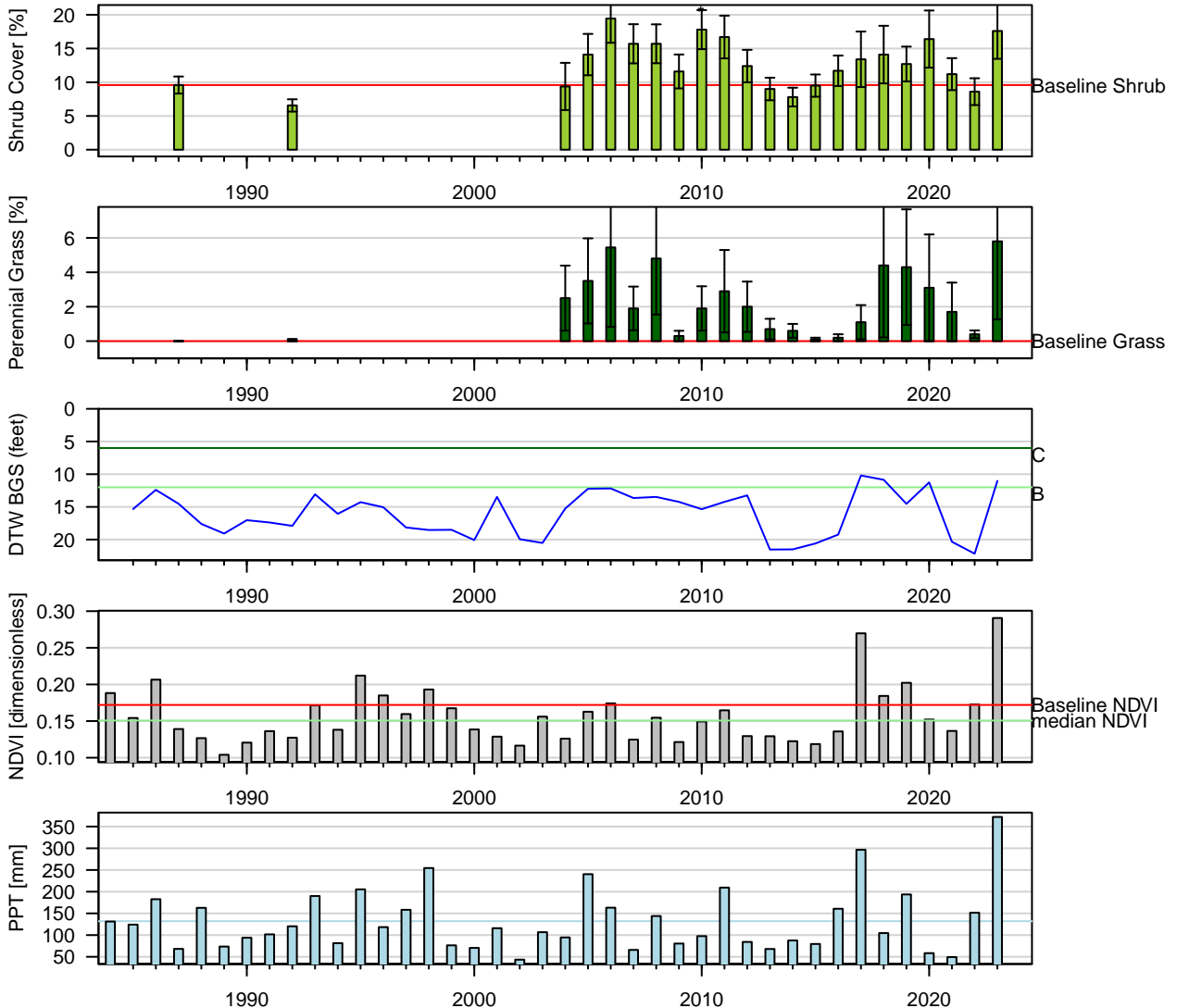
Figure 38: Two-Sample t-Test: Baseline (lpt) vs. reinventory (* p < 0.05 ). Baseline sample size ( n = 12 ). Current year sample size ( n = 10 ). Error bars = 95% CI.
