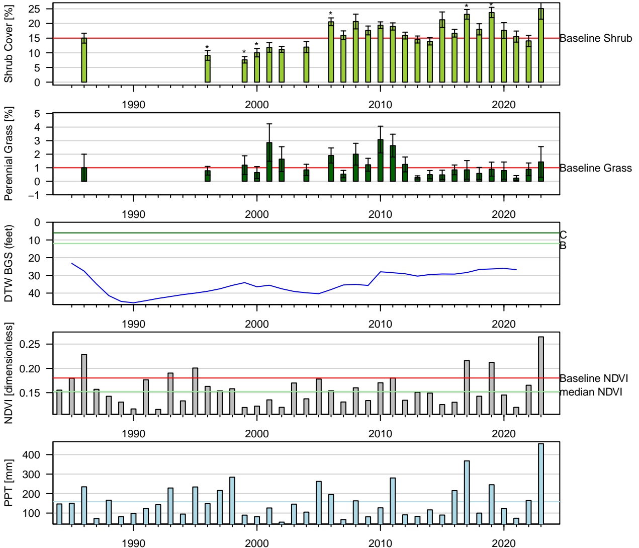
Figure 11: Two-Sample t-Test: Baseline (1pt) vs. reinventory (* p < 0.05 ). Baseline sample size ( n = 6 ). Current year sample size ( n = 14 ). Error bars = 95% CI.
