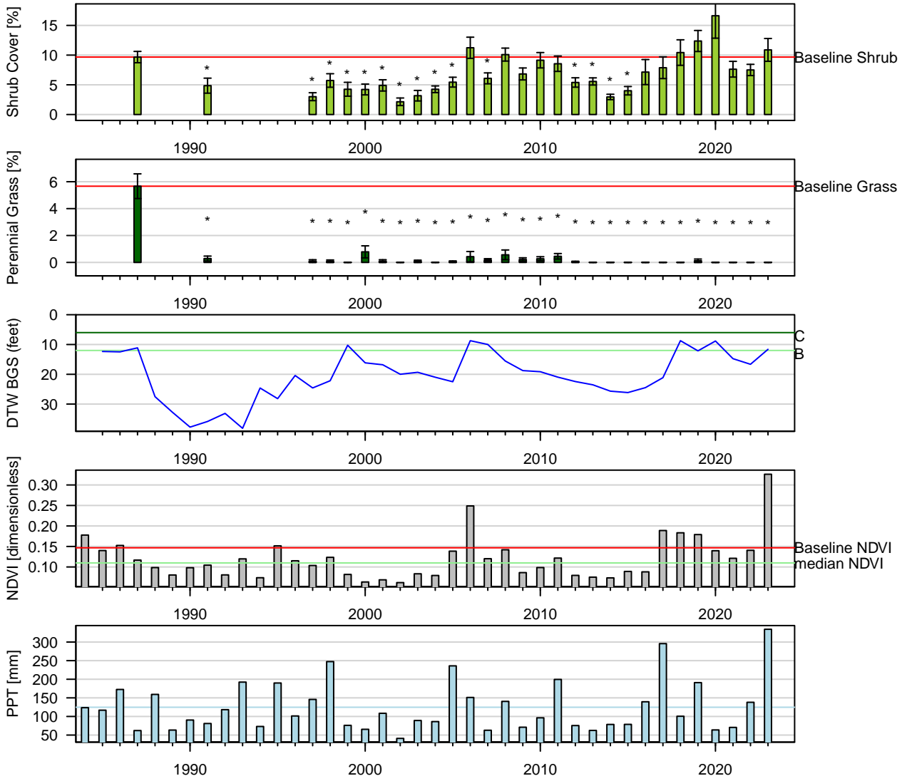
Figure 86: Two-Sample t-Test: Baseline (1pt) vs. reinventory (* p < 0.05 ). Baseline sample size ( n = 6 ). Current year sample size ( n = 8 ). Error bars = 95% CI.
