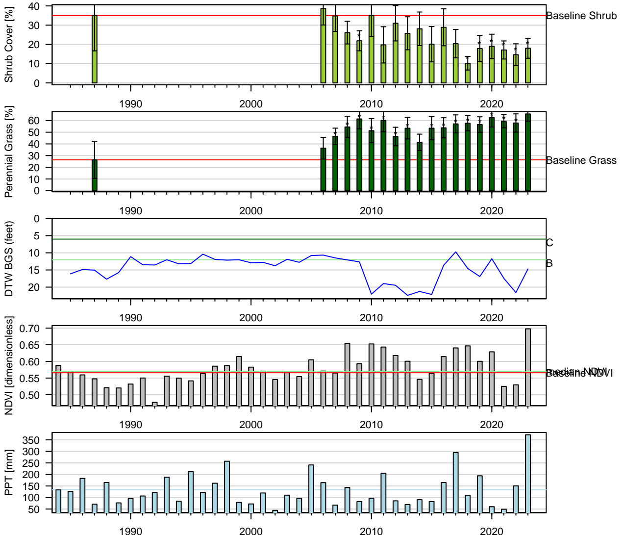
Figure 49: One-Sample t-Test: Baseline (1pt) vs. reinventory (* p < 0.05 ). Baseline sample size ( n = 3 ). Current year sample size ( n = 9 ). Error bars = 95% CI.
