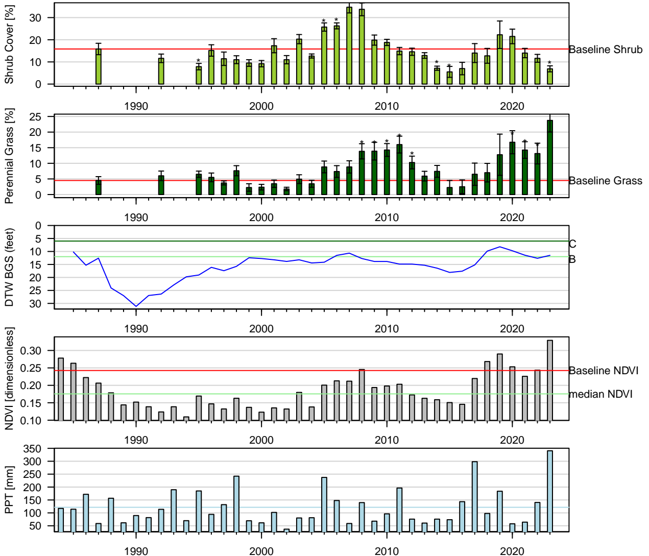
Figure 91: Two-Sample t-Test: Baseline (lpt) vs. reinventory (* p < 0.05 ). Baseline sample size ( n = 6 ). Current year sample size ( n = 8 ). Error bars = 95% CI.
