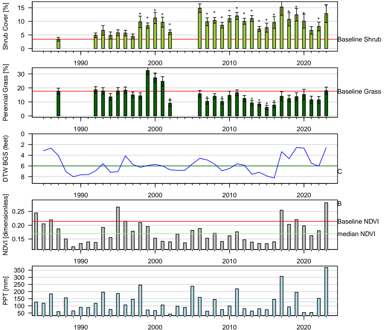
Figure 36: Two-Sample t-Test: Baseline (lpt) vs. reinventory (* p < 0.05 ). Baseline sample size ( n = 12 ). Current year sample size ( n = 12 ). Error bars = 95% CI.
