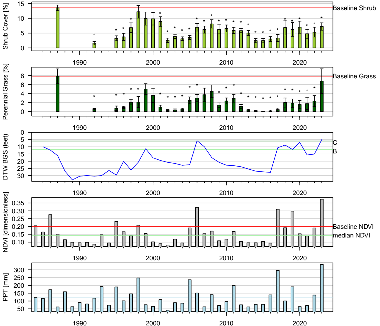
Figure 80: Two-Sample t-Test: Baseline (1pt) vs. reinventory (* p < 0.05 ). Baseline sample size ( n = 9 ). Current year sample size ( n = 9 ). Error bars = 95% CI.
