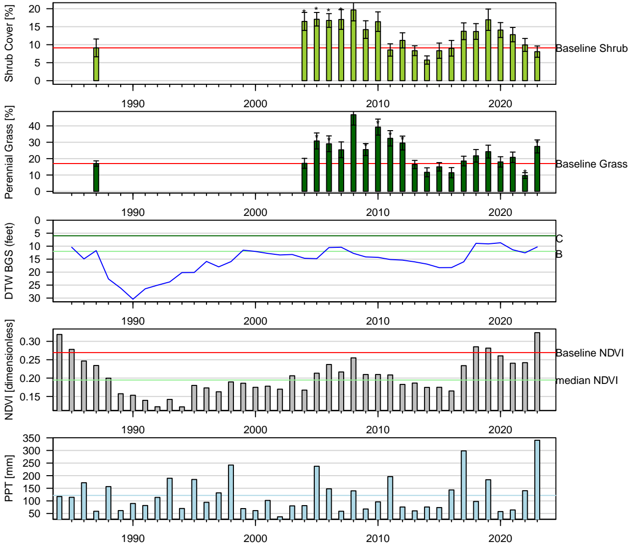
Figure 88: Two-Sample t-Test: Baseline (lpt) vs. reinventory (* p < 0.05 ).
