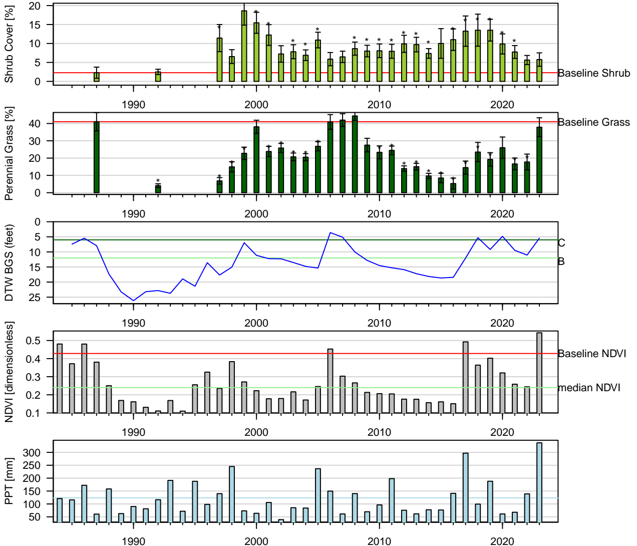
Figure 85: Two-Sample t-Test: Baseline (1pt) vs. reinventory (* p < 0.05 ). Baseline sample size ( n = 7 ). Current year sample size ( n = 8 ). Error bars = 95% CI.
