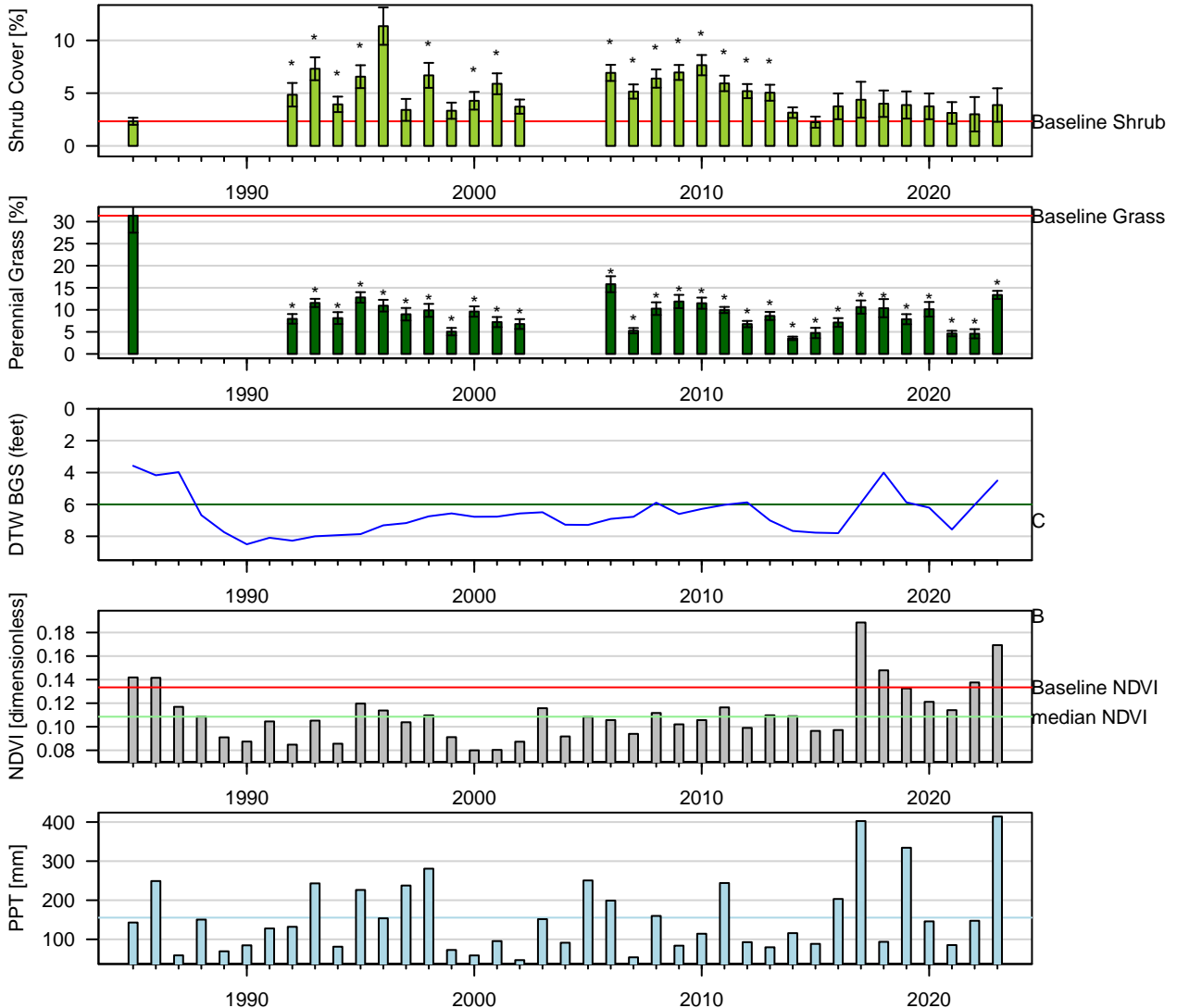
Figure 68: One-Sample t-Test: Baseline (1pt) vs. reinventory (* p < 0.05 ). Baseline sample size ( n = 3 ). Current year sample size ( n = 8 ). Error bars = 95% CI.
