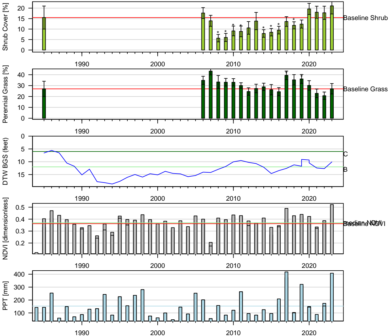
Figure 58: One-Sample t-Test: Baseline (1pt) vs. reinventory (* p < 0.05 ). Baseline sample size (n = 2). Current year sample size (n = 12). Error bars = 95% CI.
