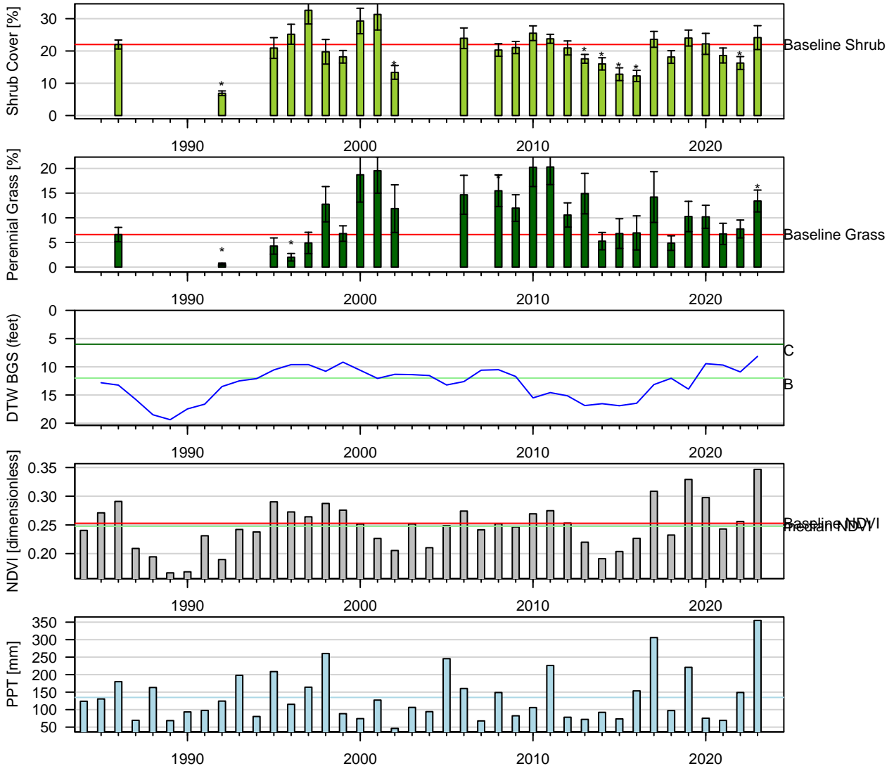
Figure 6: Two-Sample t-Test: Baseline (1pt) vs. reinventory (* p < 0.05 ). Baseline sample size ( n = 10 ). Current year sample size ( n = 15 ). Error bars = 95% CI.
