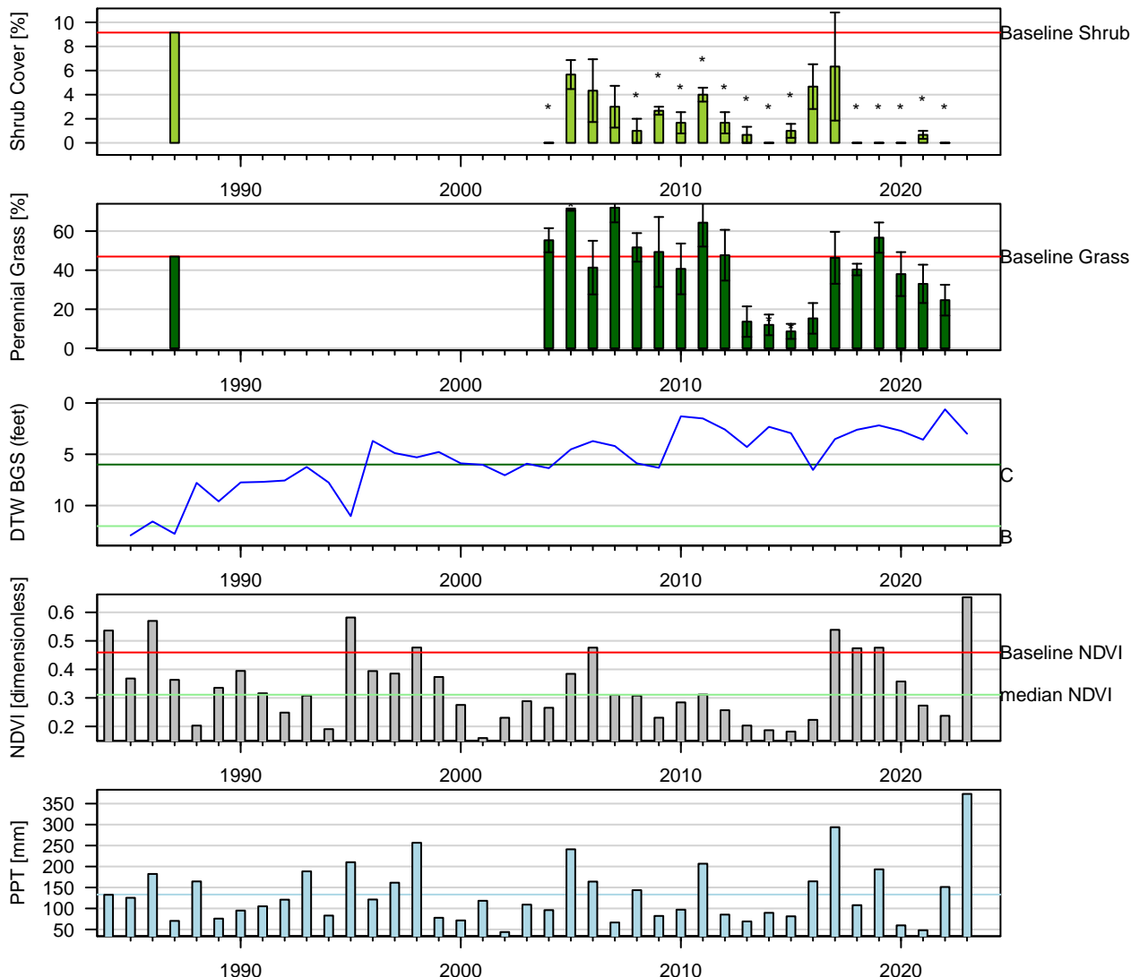
Figure 43: One-Sample t-Test: Baseline (wvcom) vs. reinventory (* p < 0.05 ). Baseline sample size ( n = 1 ). Current year sample size ( n = ). Error bars = 95% CI.
