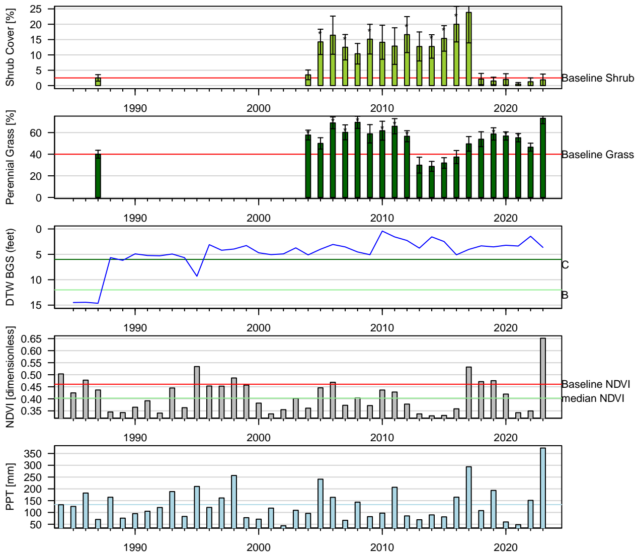
Figure 44: Two-Sample t-Test: Baseline (lpt) vs. reinventory (* p < 0.05 ). Baseline sample size ( n = 6 ). Current year sample size ( n = 8 ). Error bars = 95% CI.
