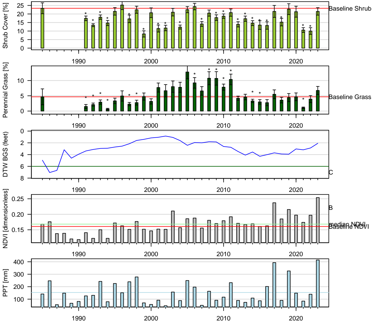
Figure 65: One-Sample t-Test: Baseline (1pt) vs. reinventory (* p < 0.05 ). Baseline sample size ( n = 3 ). Current year sample size ( n = 12 ). Error bars = 95% CI.
