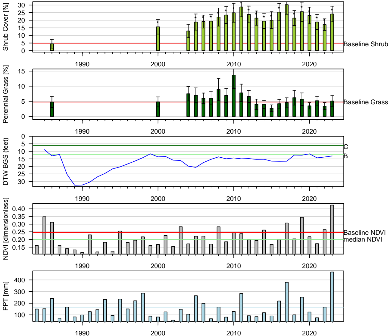
Figure 13: One-Sample t-Test: Baseline (1pt) vs. reinventory (* p < 0.05 ). Baseline sample size (n = 4). Current year sample size (n = 10). Error bars = 95% CI.
