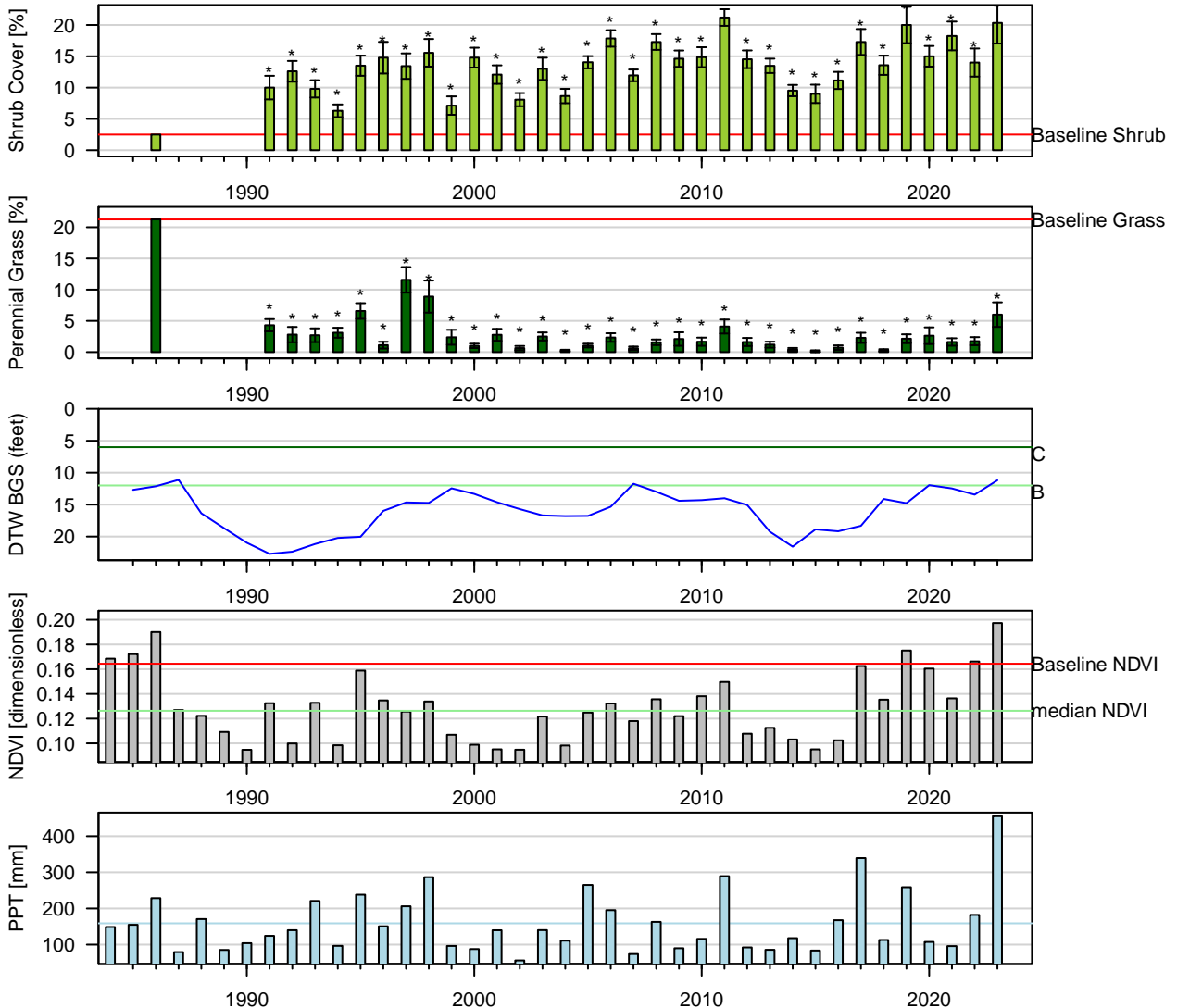
Figure 52: One-Sample t-Test: Baseline (wvcom) vs. reinventory (* p < 0.05 ). Baseline sample size ( n = 1 ). Current year sample size ( n = 6 ). Error bars = 95% CI.
