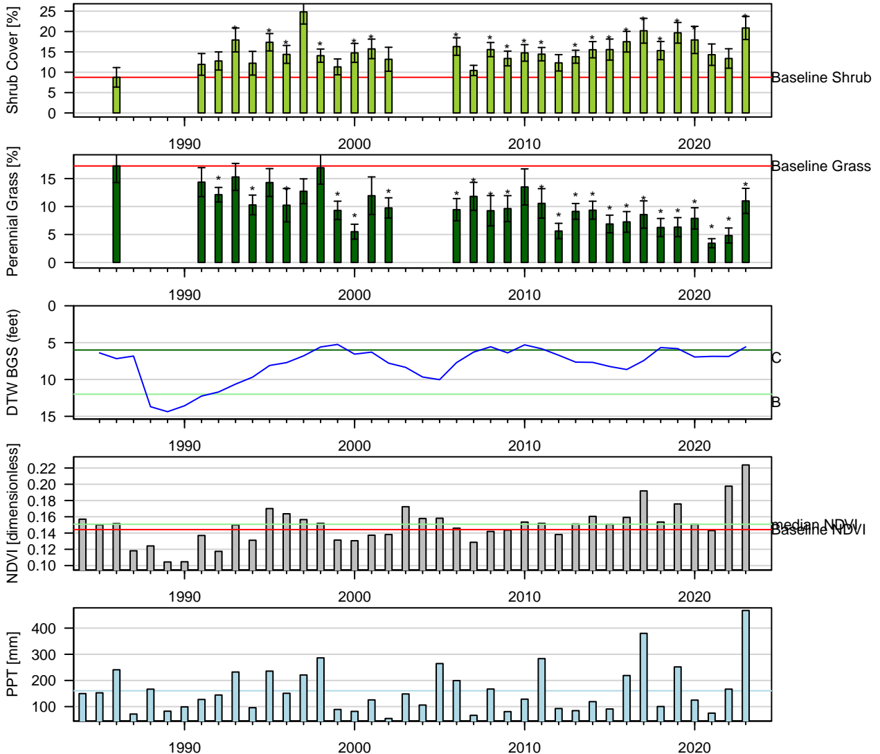
Figure 29: One-Sample t-Test: Baseline (1pt) vs. reinventory (* p < 0.05 ). Baseline sample size (n = 4). Current year sample size (n = 16). Error bars = 95% CI.
