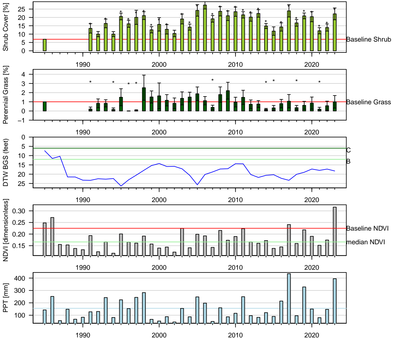
Figure 66: One-Sample t-Test: Baseline (wvcom) vs. reinventory (* p < 0.05 ). Baseline sample size ( n = 1 ). Current year sample size ( n = 15 ). Error bars = 95% CI.
