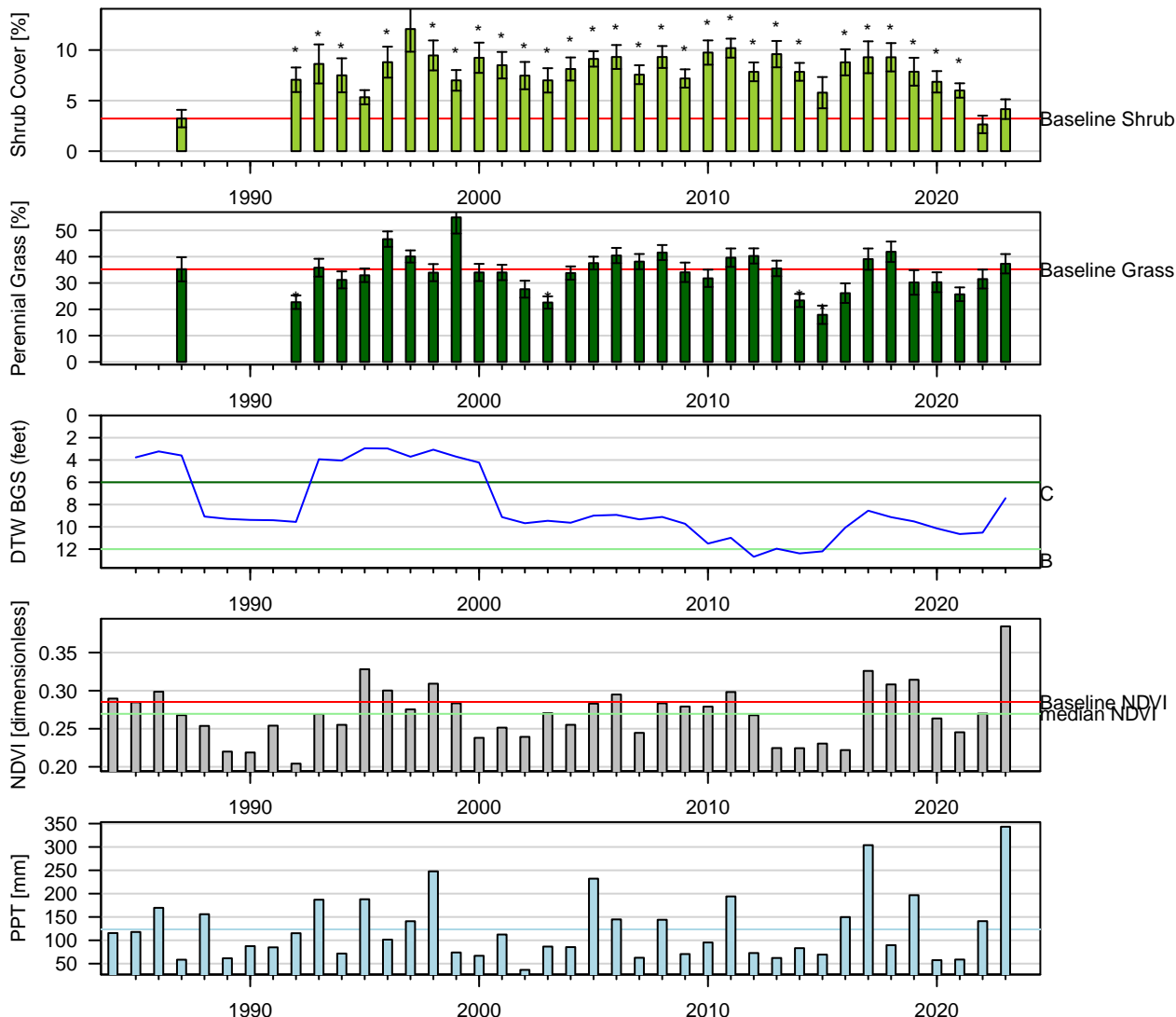
Figure 113: Two-Sample t-Test: Baseline (1pt) vs. reinventory (* p < 0.05 ). Baseline sample size (n = 9). Current year sample size (n = 13). Error bars = 95% CI.
