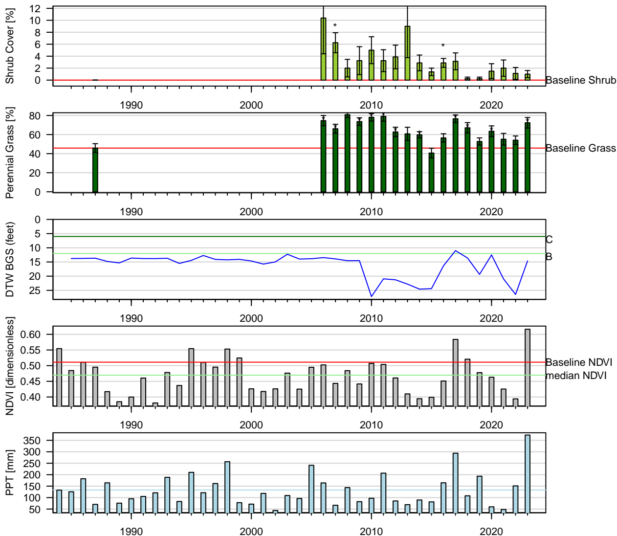
Figure 48: Two-Sample t-Test: Baseline (1pt) vs. reinventory (* p < 0.05 ). Baseline sample size ( n = 6 ). Current year sample size ( n = 8 ). Error bars = 95% CI.
