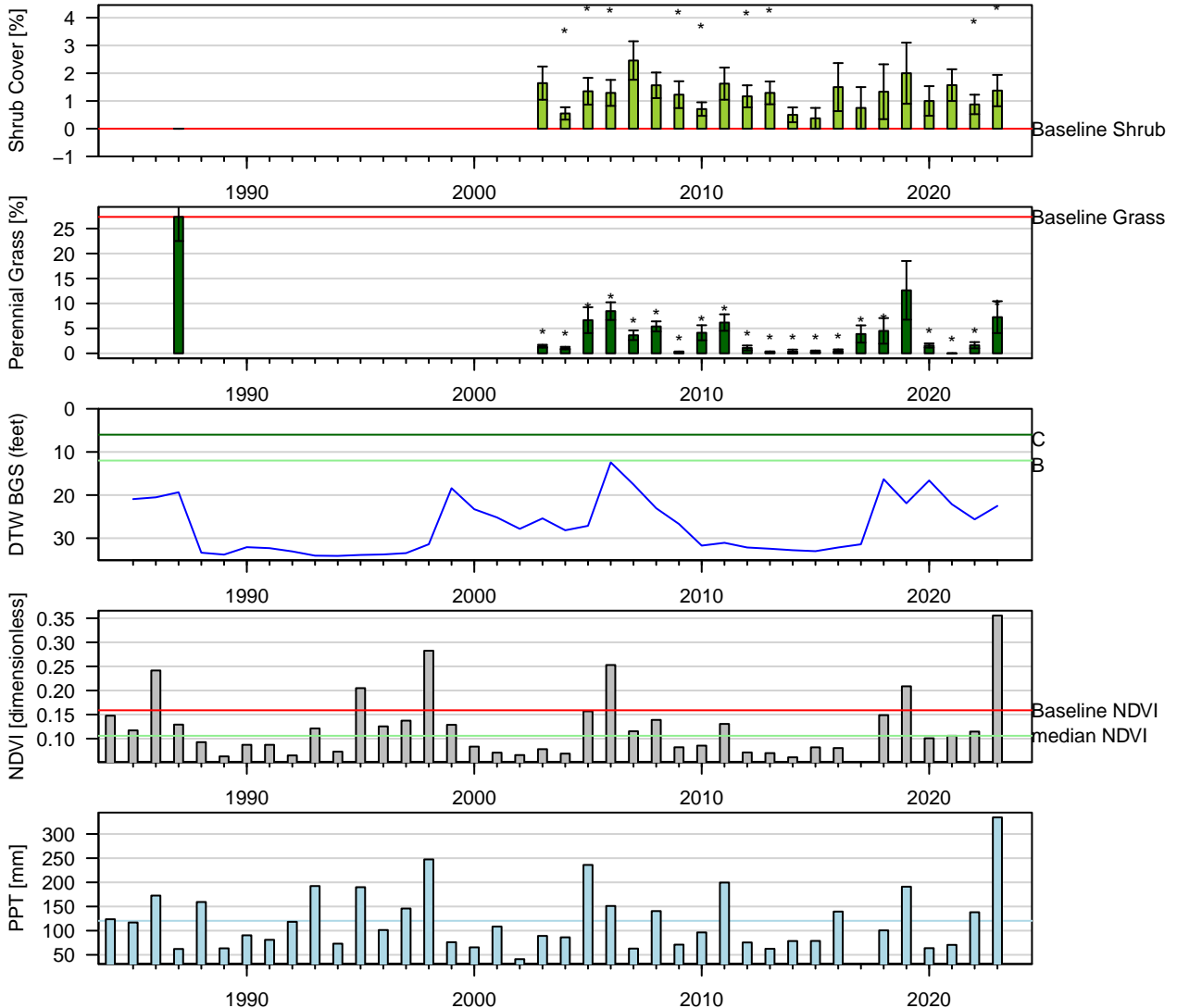
Figure 77: Two-Sample t-Test: Baseline (1pt) vs. reinventory (* p < 0.05 ). Baseline sample size ( n = 6 ). Current year sample size ( n = 8 ). Error bars = 95% CI.
