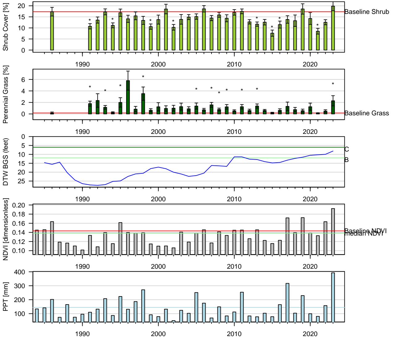
Figure 117: Two-Sample t-Test: Baseline (1pt) vs. reinventory (* p < 0.05 ). Baseline sample size ( n = 6 ). Current year sample size ( n = 14 ). Error bars = 95% CI.
