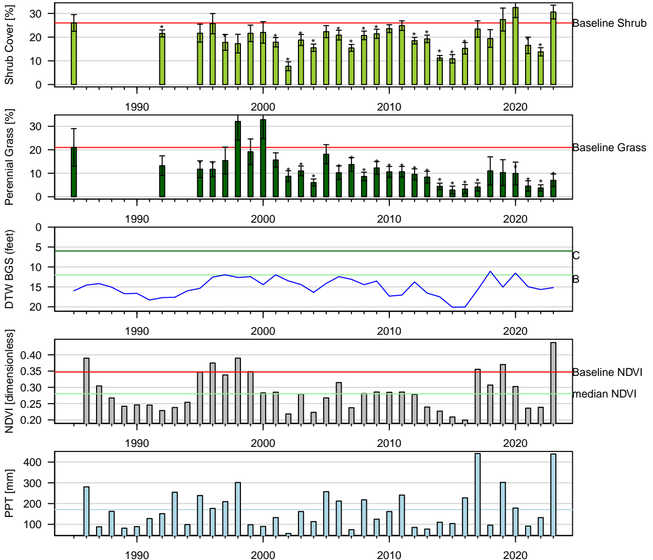
Figure 96: One-Sample t-Test: Baseline (lpt) vs. reinventory (* p < 0.05 ). Baseline sample size ( n = 3 ). Current year sample size ( n = 10 ). Error bars = 95% CI.
