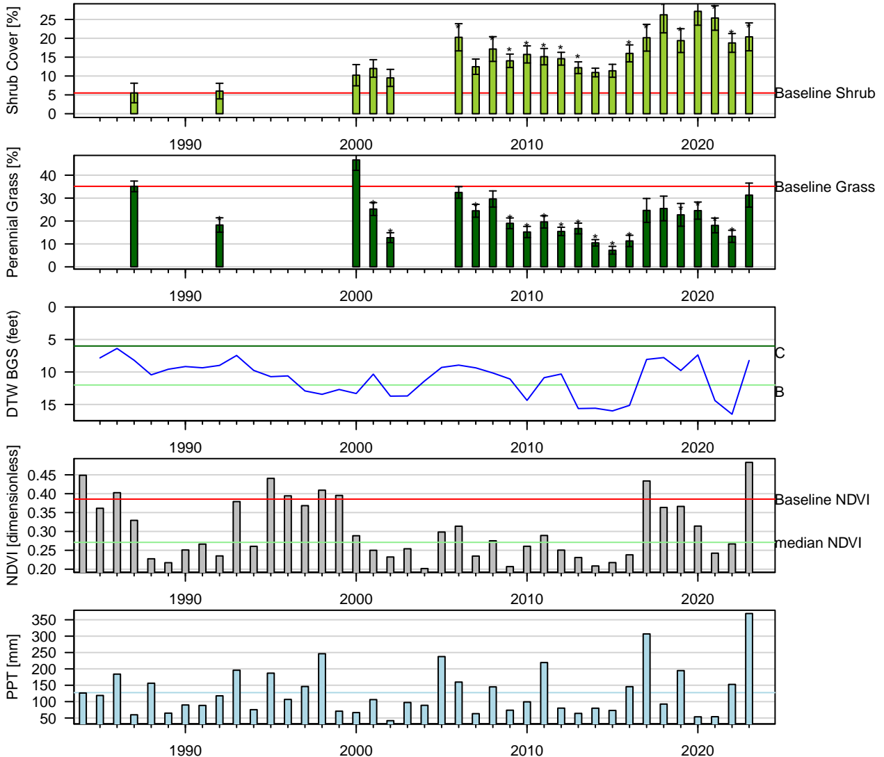
Figure 37: Two-Sample t-Test: Baseline (lpt) vs. reinventory (* p < 0.05 ).
