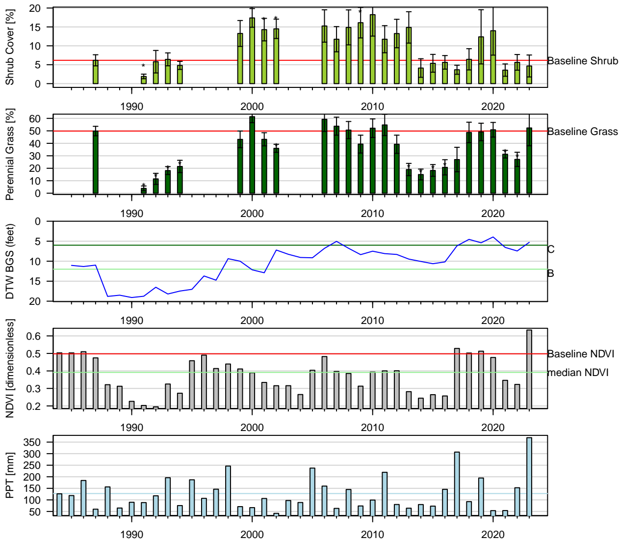
Figure 32: Two-Sample t-Test: Baseline (lpt) vs. reinventory (* p < 0.05 ). Baseline sample size ( n = 6 ). Current year sample size ( n = 3 ). Error bars = 95% CI.
