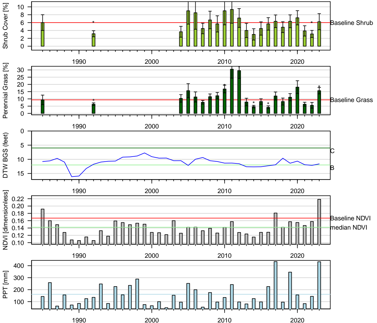
Figure 102: One-Sample t-Test: Baseline (1pt) vs. reinventory (* p < 0.05 ). Baseline sample size ( n = 3 ). Current year sample size ( n = 9 ). Error bars = 95% CI.
