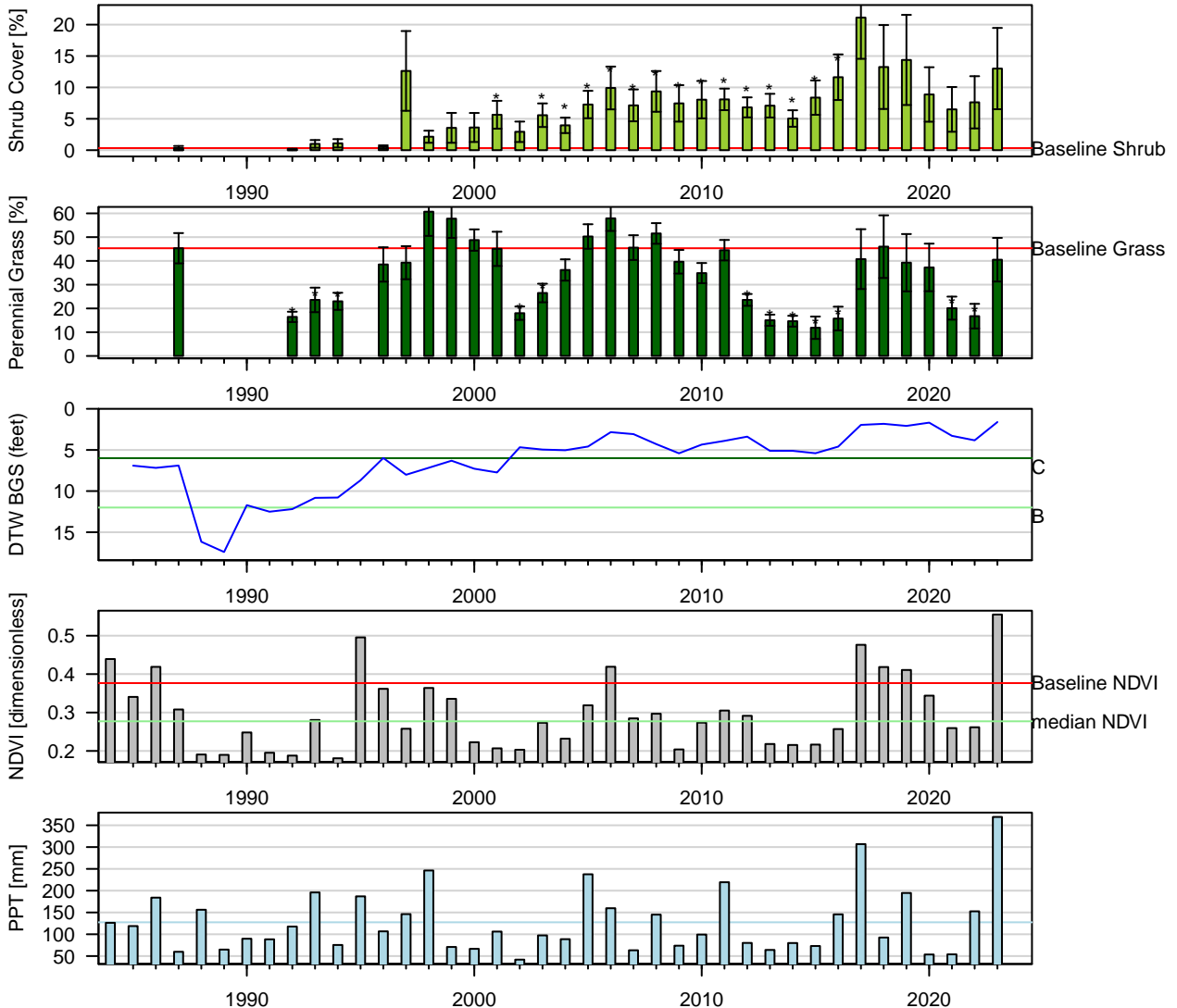
Figure 40: Two-Sample t-Test: Baseline (lpt) vs. reinventory (* p < 0.05 ). Baseline sample size ( n = 6 ). Current year sample size ( n = 8 ). Error bars = 95% CI.
