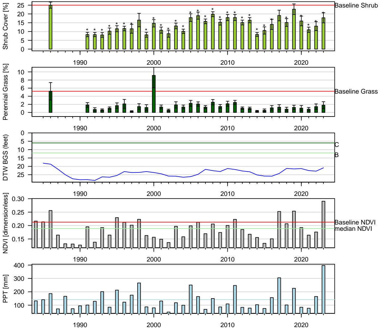
Figure 7: Two-Sample t-Test: Baseline (1pt) vs. reinventory (* p < 0.05 ). Baseline sample size ( n = 9 ). Current year sample size ( n = 15 ). Error bars = 95% CI.
