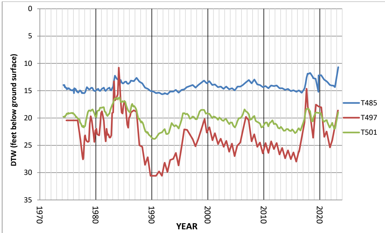
Figure 11.c. Hydrographs of selected monitoring wells in the eastern Bishop wellfield.
