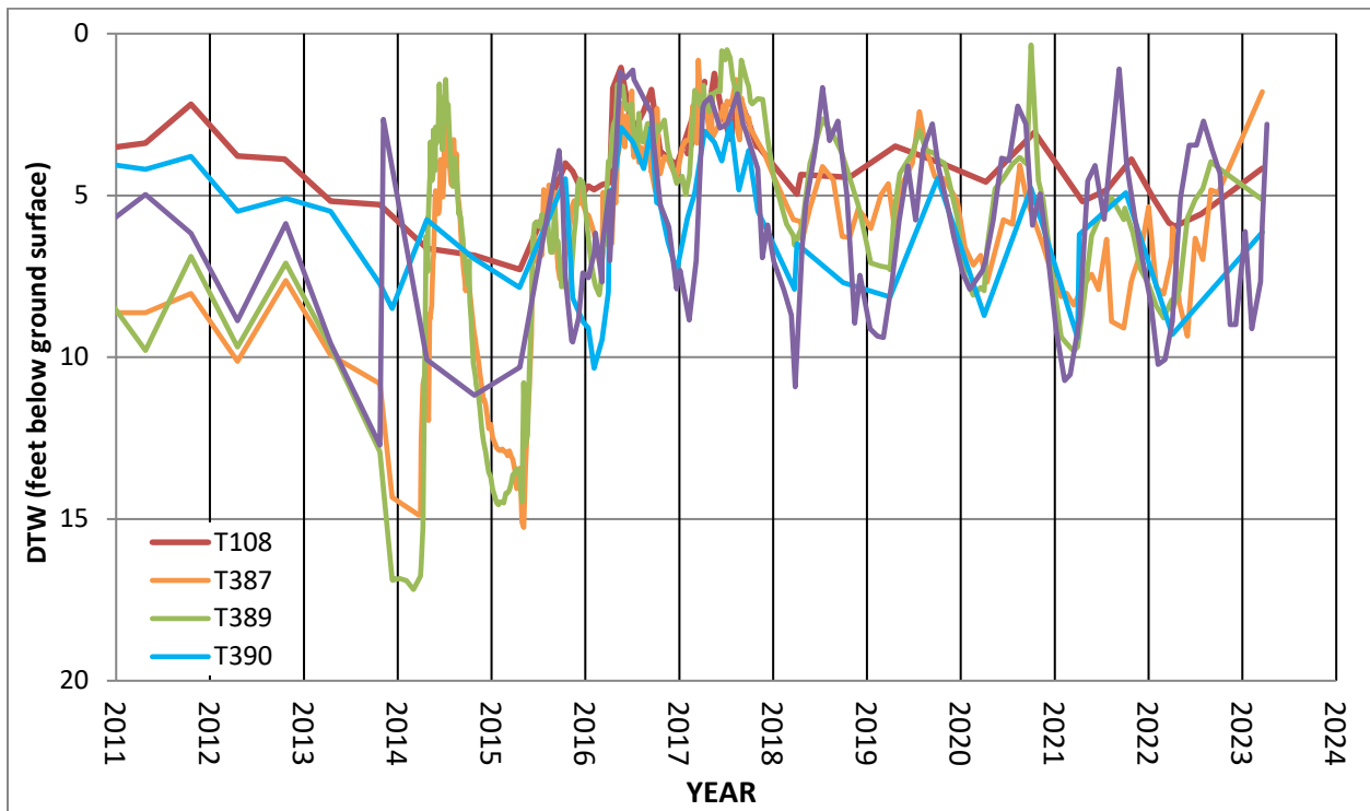
Figure 12. Recent hydrographs of selected monitoring wells in western Bishop wellfield.
