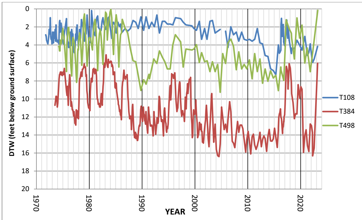
Figure 11.b. Hydrographs of selected monitoring wells in the northern Bishop wellfield.
