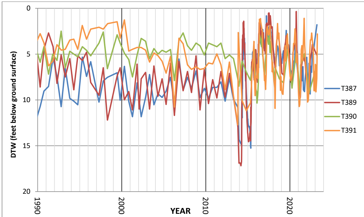
Figure 11.a. Hydrographs of selected monitoring wells in the western Bishop wellfield.
