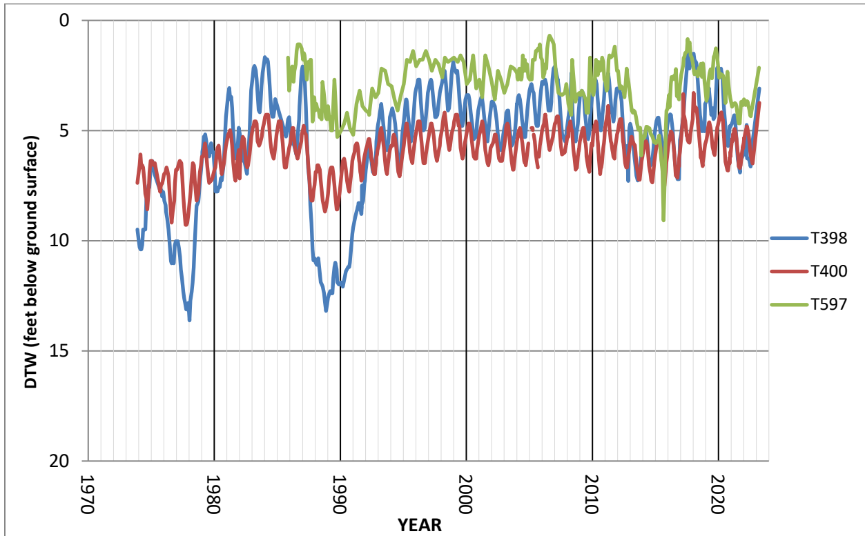
Figure 32. Hydrographs of Indicator wells and 597T in the Bairs-Georges wellfield.
