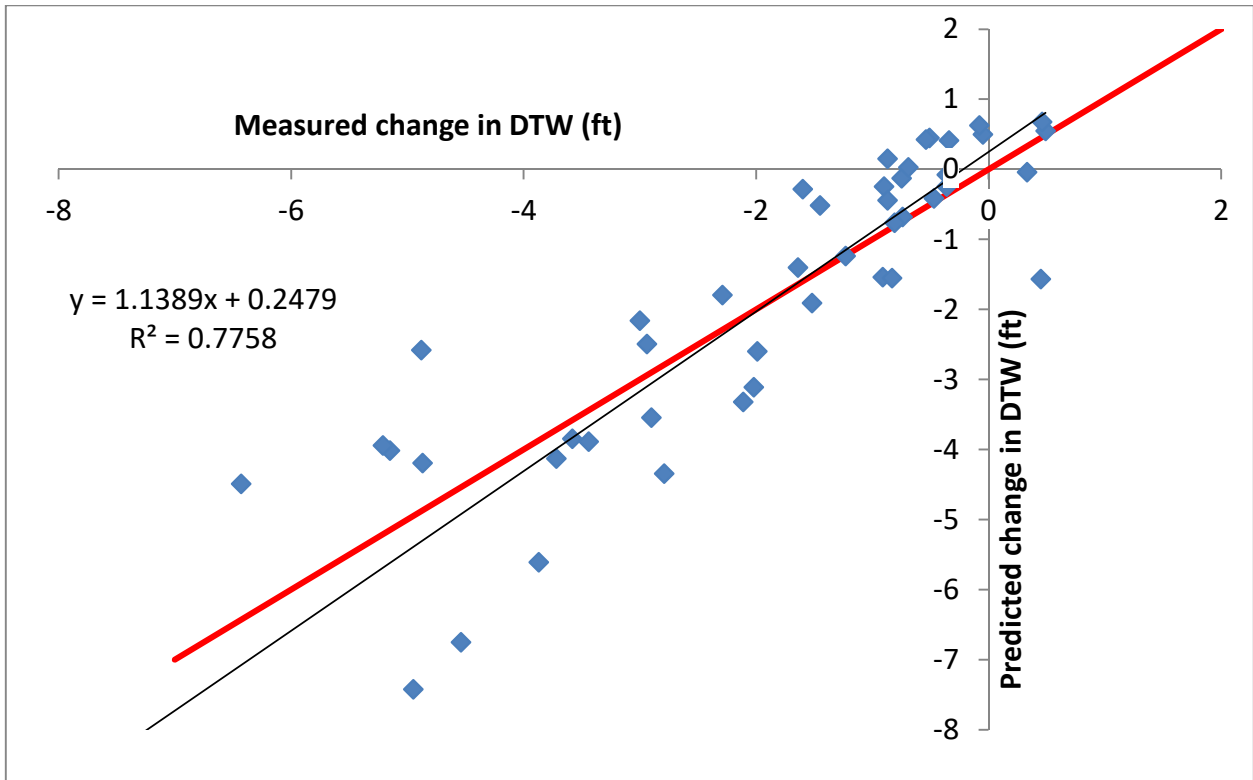
Figure 3.37. Corrected measured and predicted change in DTW from April 2020 to April 2021 for 46 indicator well using actual pumping and runoff values. The solid red line is the 1:1 line. Negative values denote decline in water level. Data points right of the redline indicate actual groundwater level changes were more positive (shallower) than predicted.
