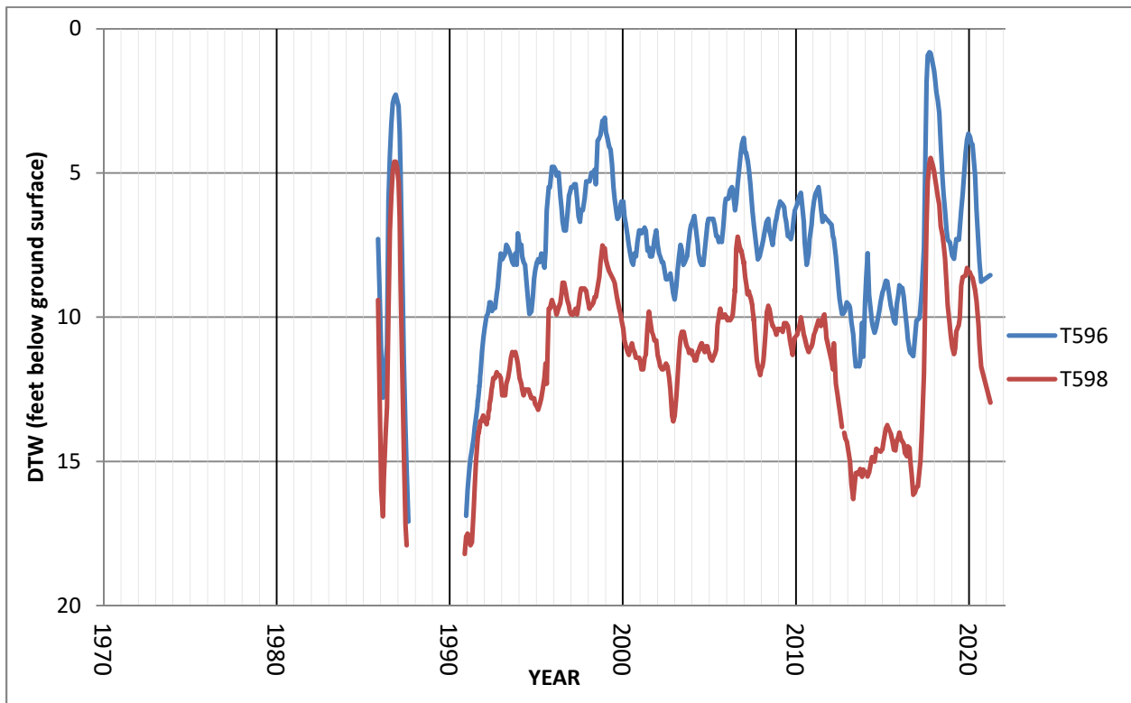
Figure 3.33. Hydrographs of selected wells in the Bairs-Georges wellfield.
