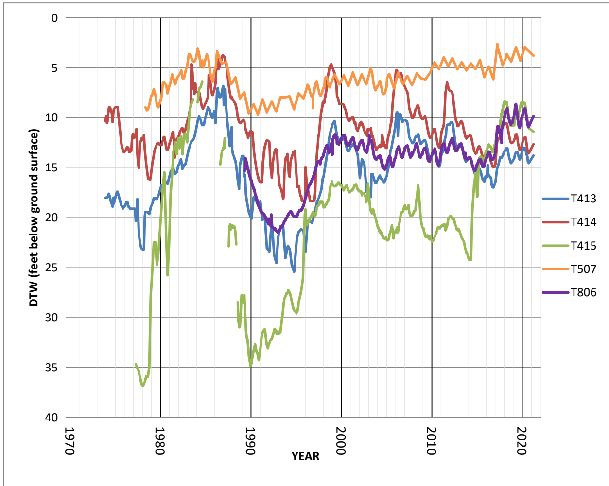
Figure 3.22. Hydrographs of selected test wells in the Thibaut-Sawmill wellfield.
