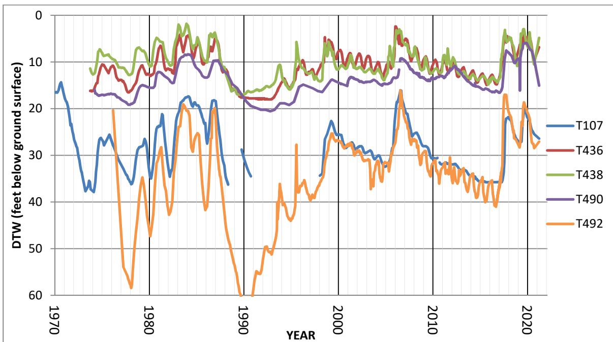
Figure 3.9. Hydrographs of indicator wells in the Laws wellfield. Well T492 is dry if DTW is below 60 ft, and well T107 is dry if DTW is below 37 feet.
