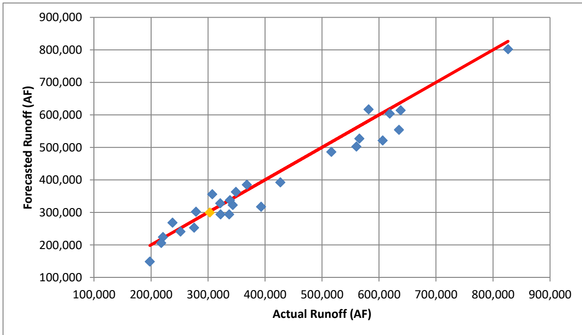
Figure 3.1. Comparison of actual and forecasted runoff 1994-2020 runoff years with 100% accuracy between forecast and actual runoff in red. The most recent year is the orange diamond (2020 actual runoff was 303,013 ac-ft; forecasted runoff was 299,600 ac-ft).
