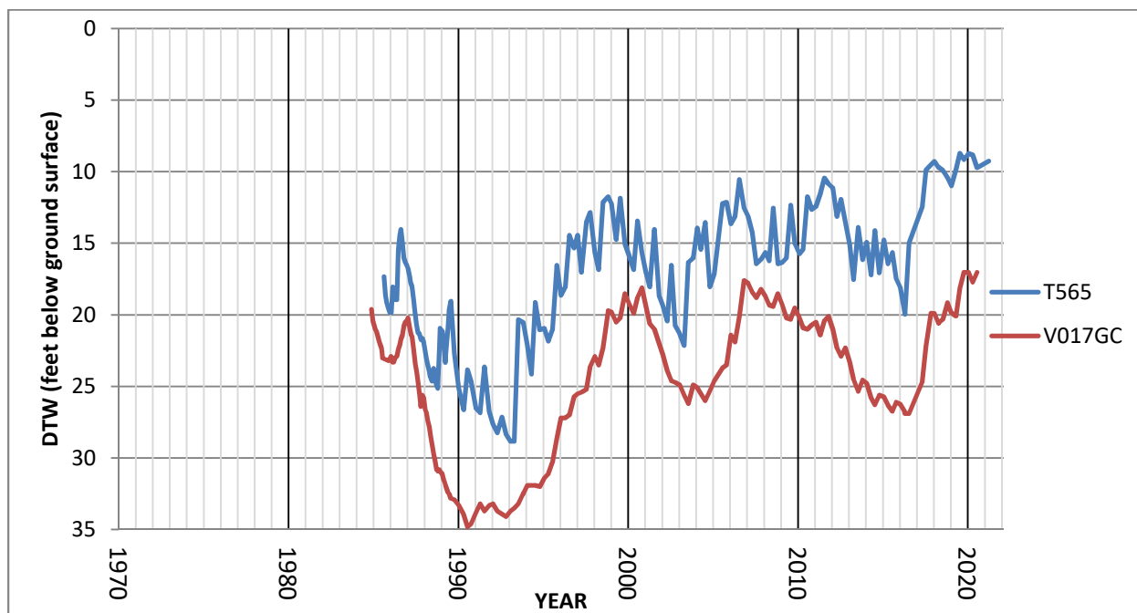
Figure 3.16. Hydrographs of monitoring wells in the southern Big Pine wellfield near pumping wells W218 and W219.
