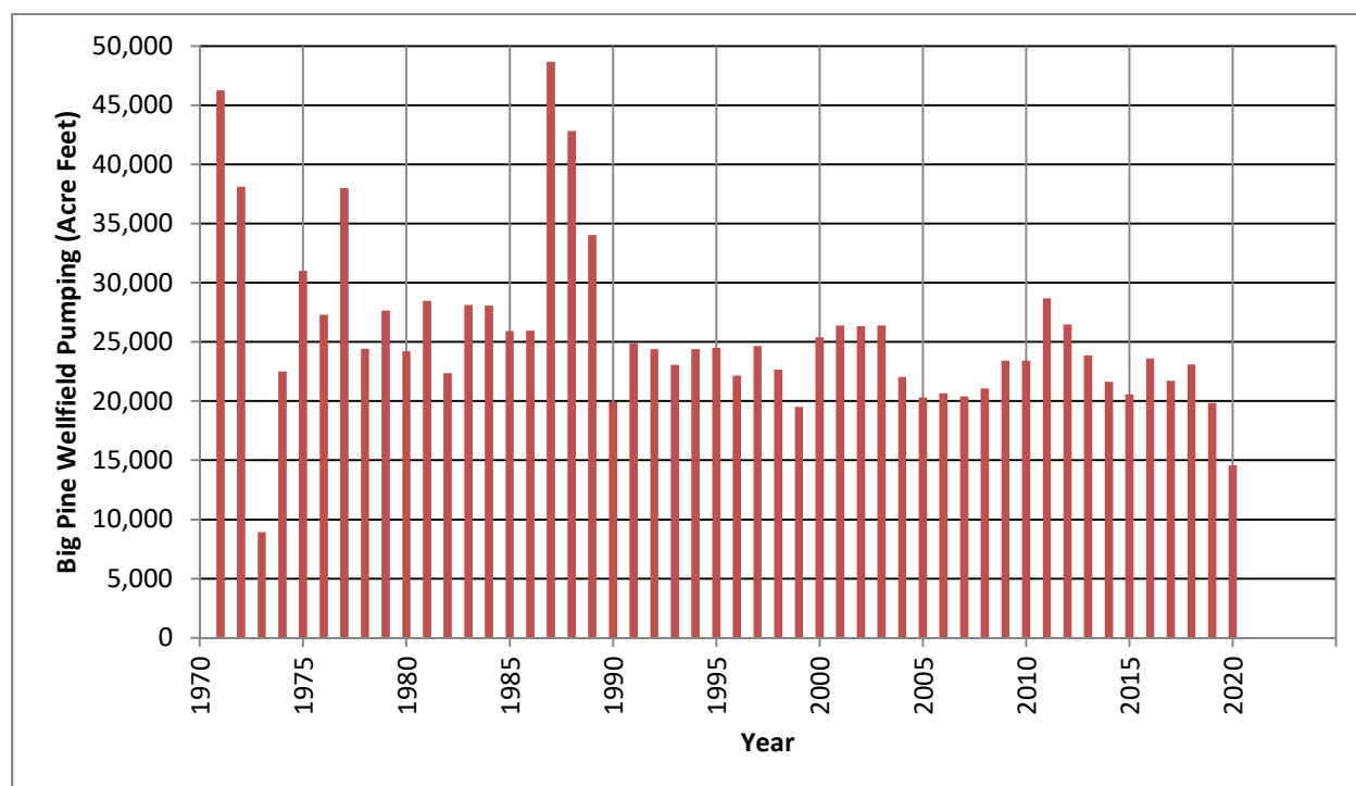
Figure 3.14. Pumping totals for the Big Pine wellfield
