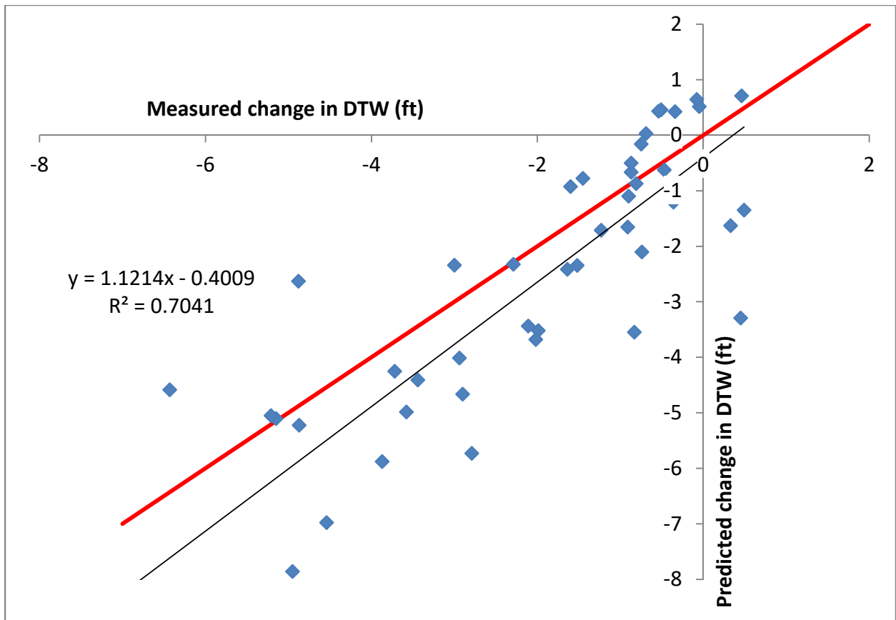
Figure 3.36. Measured and predicted change in DTW from April 2020 to April 2021 for 46 indicator wells. The solid red line is the 1:1 line. Negative values denote decline in water level. Data points right of the redline indicate actual groundwater level changes were more positive (shallower) than predicted.
