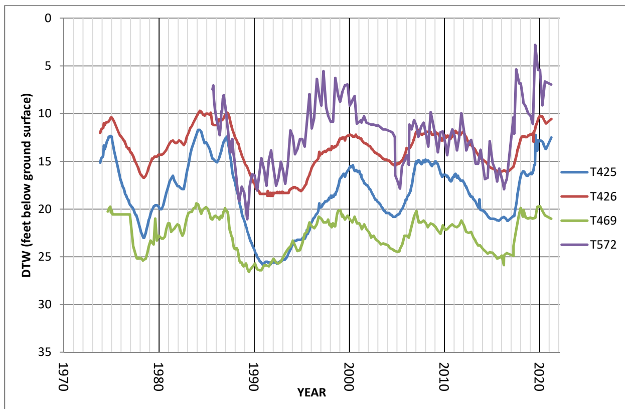
Figure 3.15. Hydrographs of indicator wells in the Big Pine wellfield. Periods of missing data for T572 occurred when the well was plugged and in need of repair.
