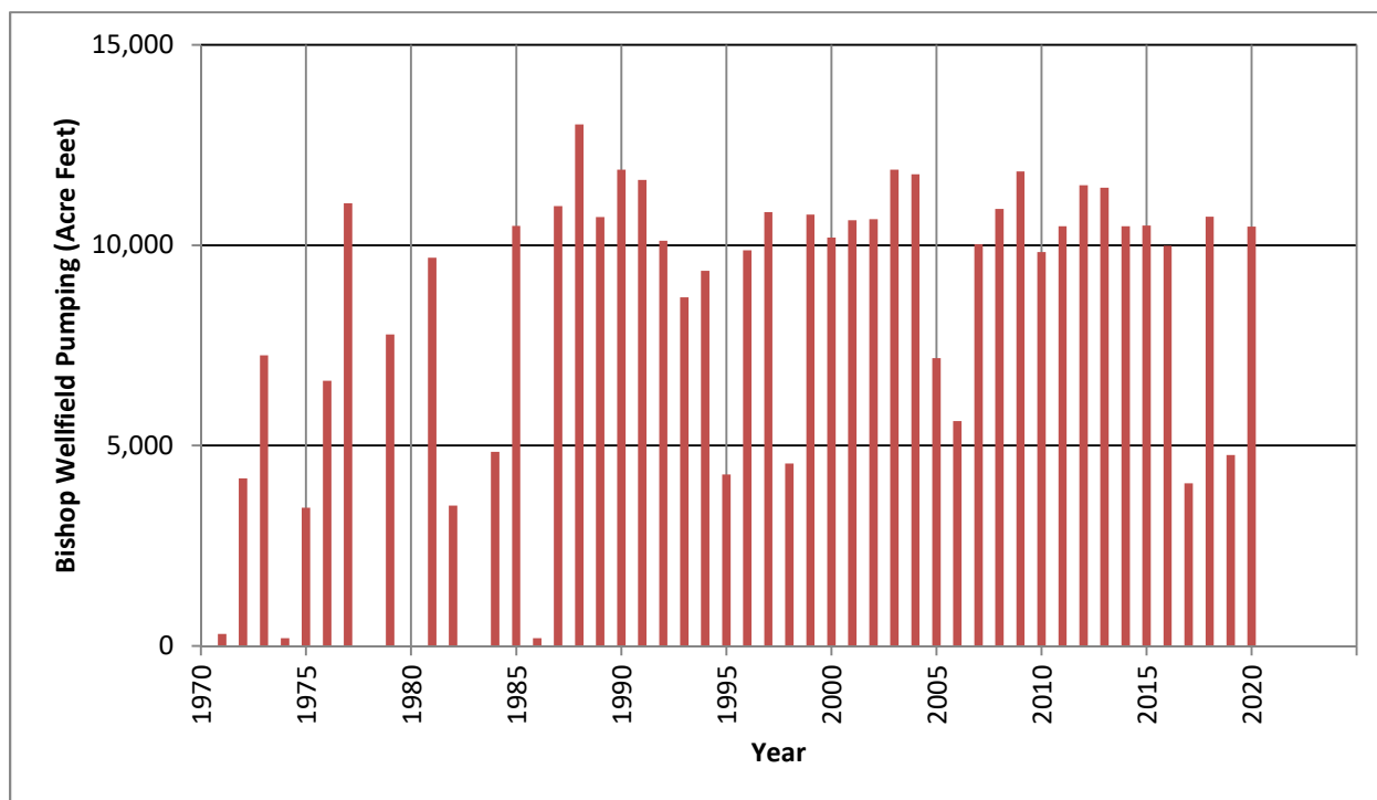
Figure 3.10. Pumping totals for the Bishop wellfield.
