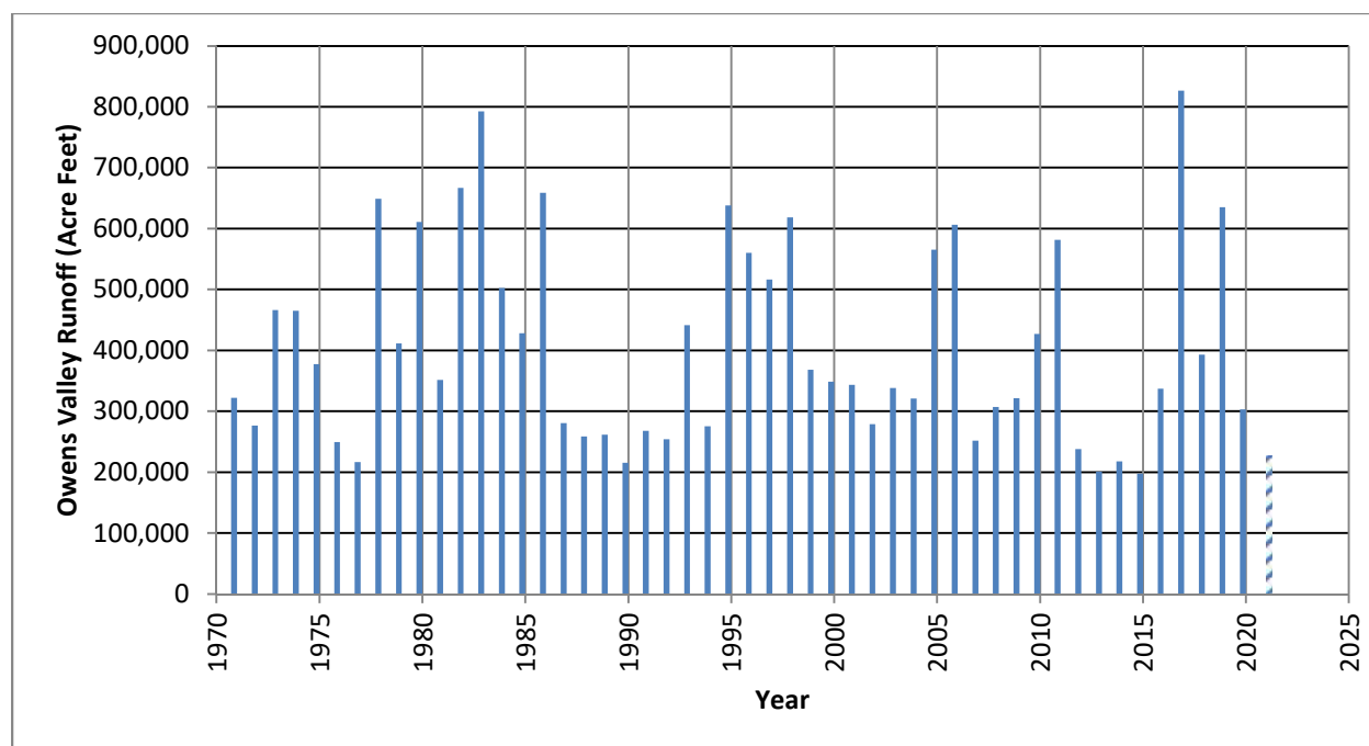
Figure 3.3. Measured Owens Valley runoff since 1970. Values are for the runoff year (e.g. runoff year 2020 includes April 1, 2020 through March 31, 2021). Dash line is current runoff year estimate.
