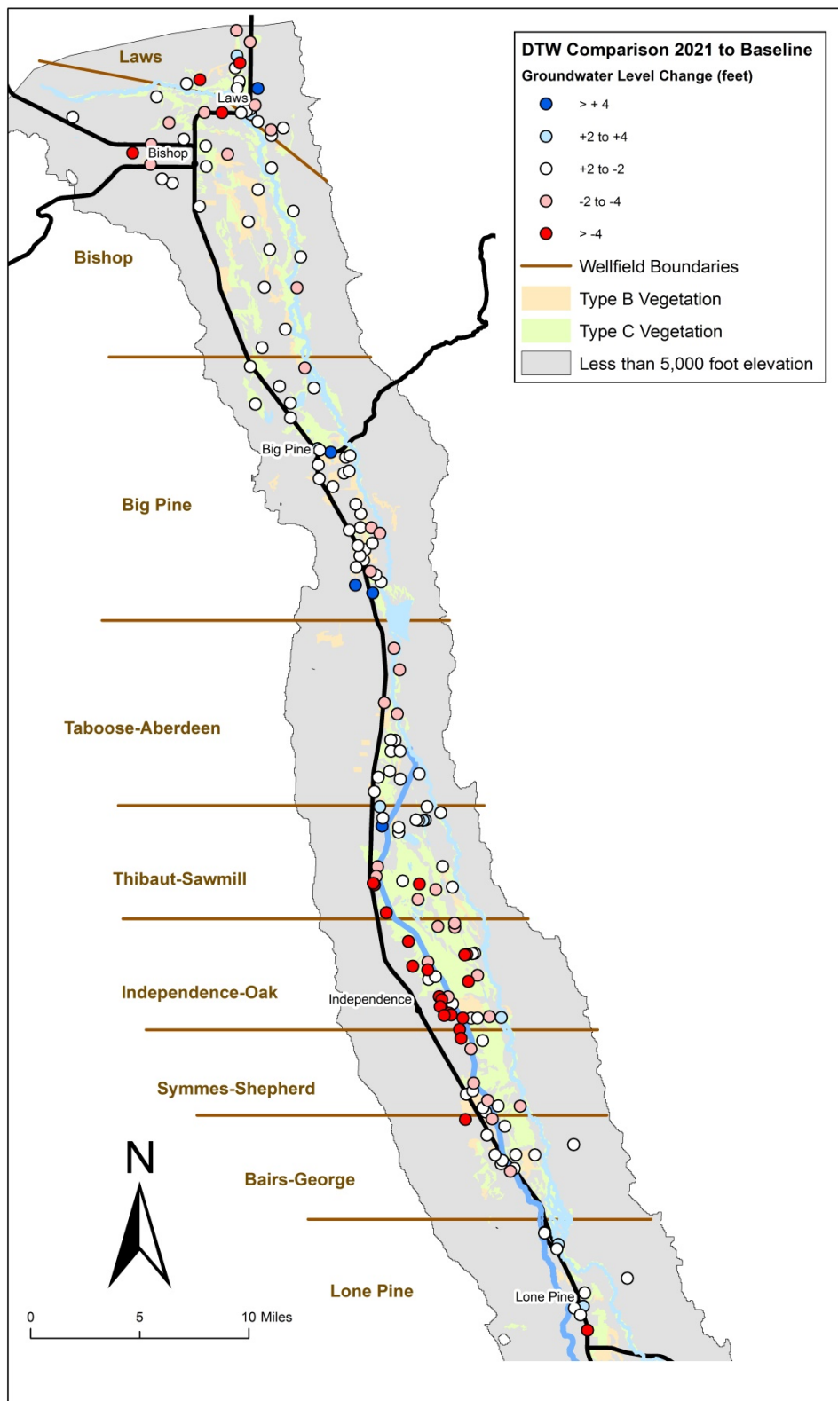
Figure 3.6. Spring 2021 groundwater levels wells compared with average water level in spring 1985-87.
