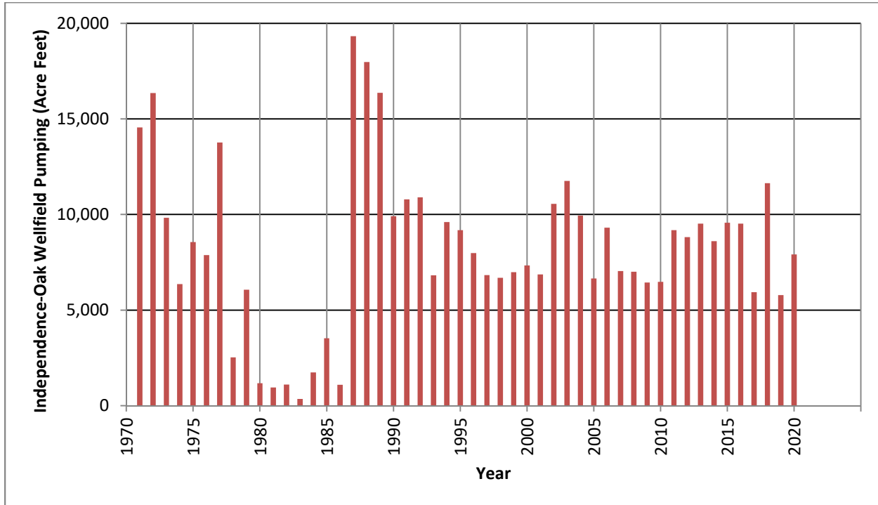
Figure 3.24. Pumping totals for the Independence-Oak wellfield.
