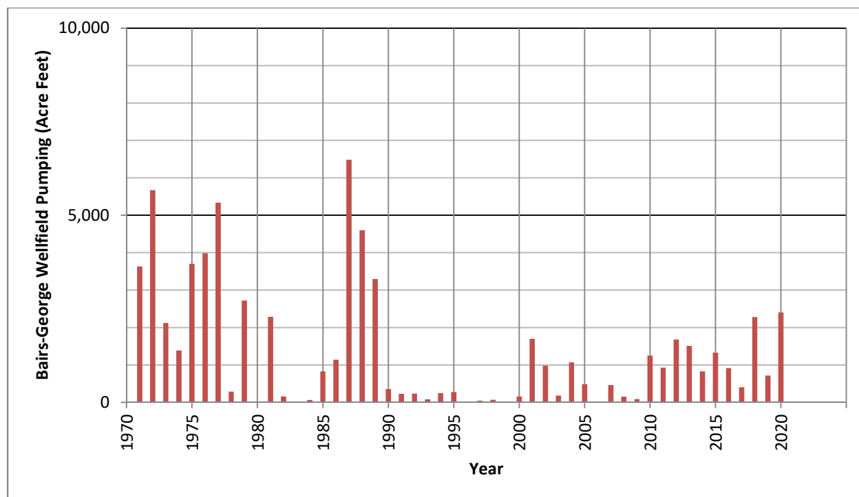
Figure 3.31. Pumping totals for the Bairs-Georges wellfield.
