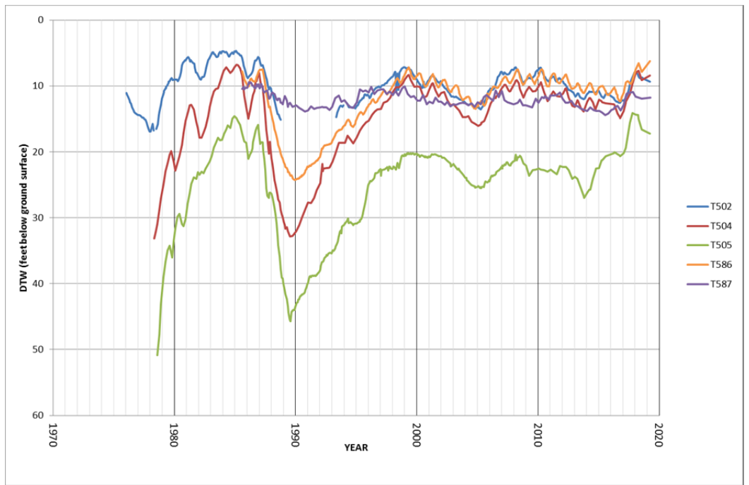
Figure 3.20. Hydrographs of indicator wells in the Taboose-Aberdeen wellfield. Periods of missing data denote when the test well was dry.
