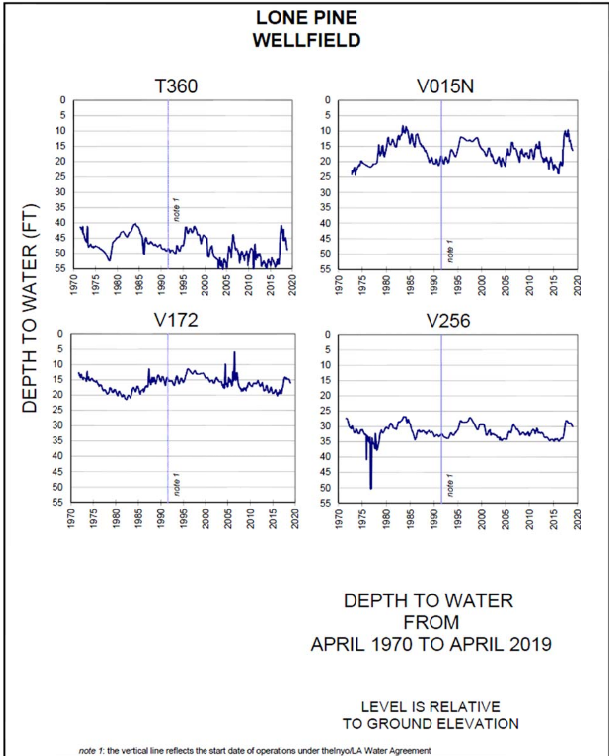
Figure 2.10. Depth to Water Hydrographs for Lone Pine Wellfield
