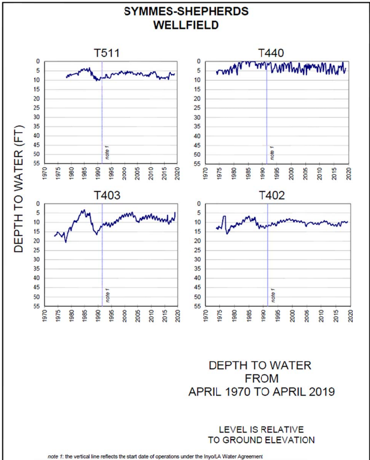
Figure 2.8. Depth to Water Hydrographs for Symmes-Shepard Wellfield
