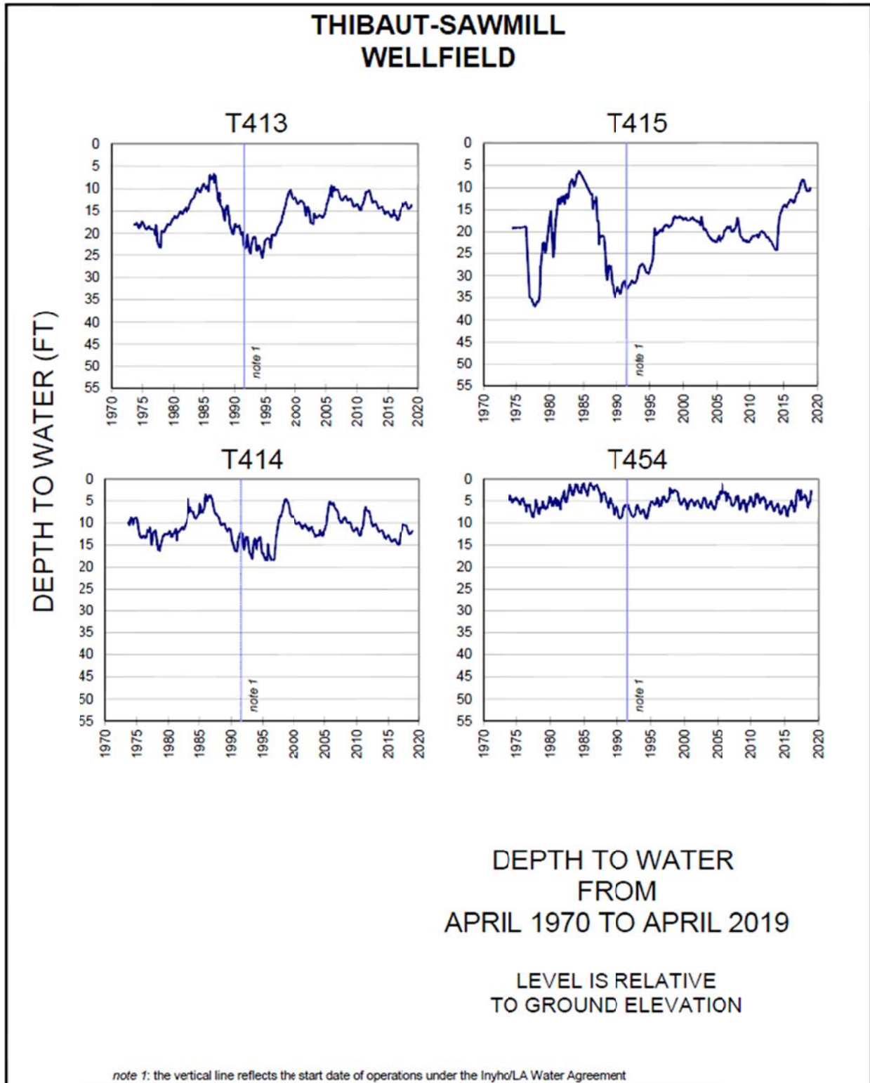
Figure 2.6. Depth to Water Hydrographs for Thibaut-Sawmill Wellfield
