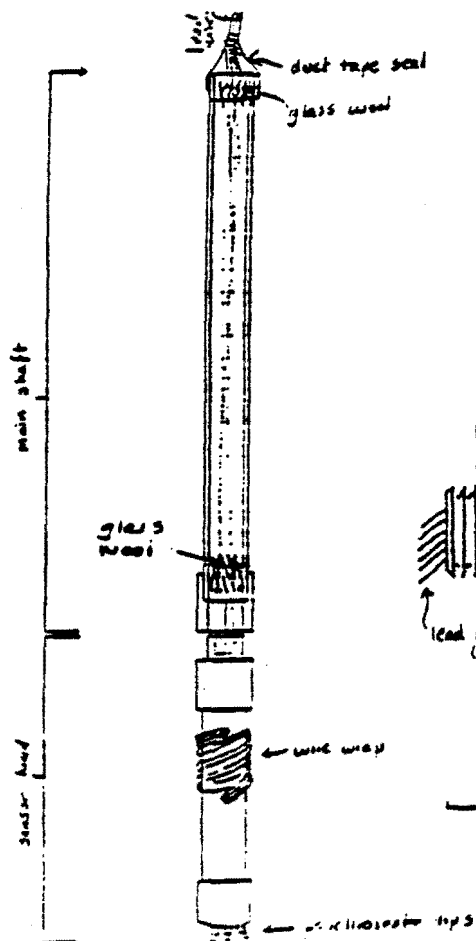
Figure 1. Psychrometer Cassette
