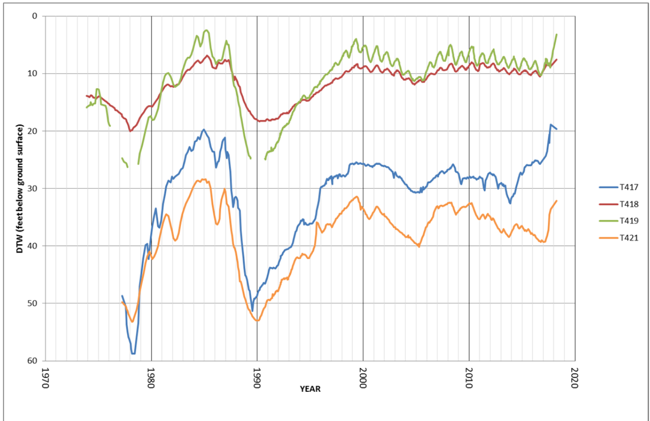
Figure 3.19. Hydrographs of indicator wells in the Taboose-Aberdeen wellfield.
