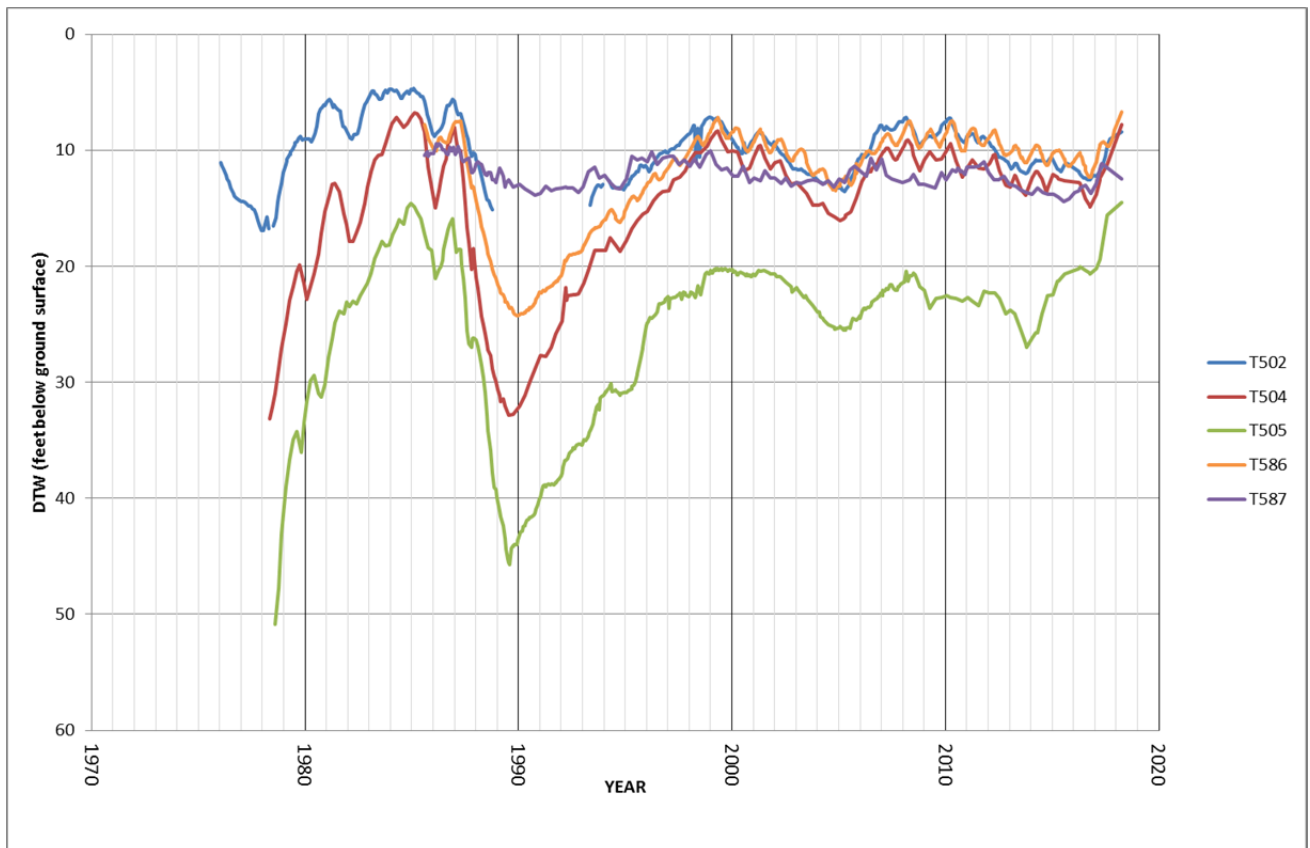
Figure 3.20. Hydrographs of indicator wells in the Taboose-Aberdeen wellfield.
