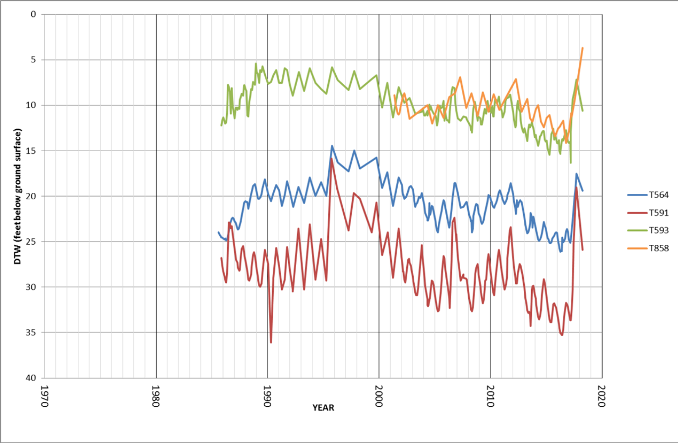
Figure 3.35. Hydrographs of selected test wells in the Lone Pine wellfield.
