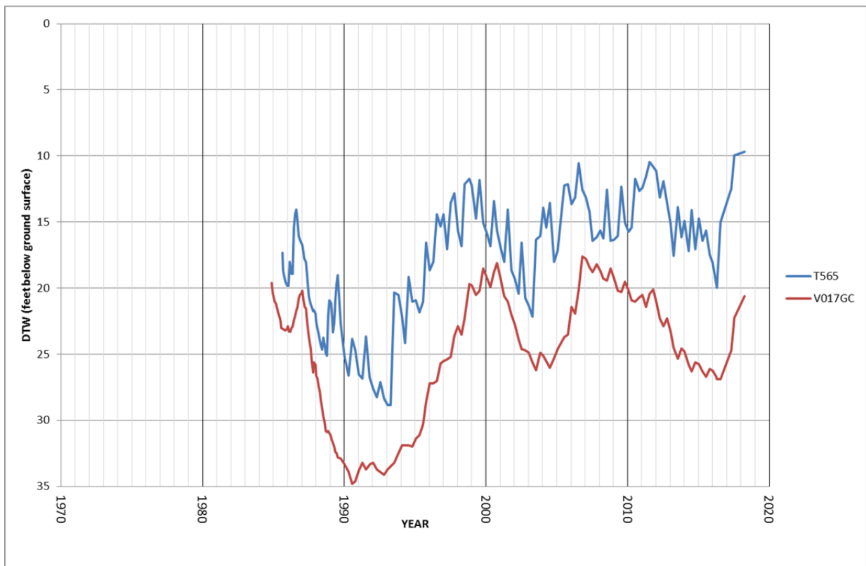
Figure 3.16. Hydrographs of monitoring wells in the southern Big Pine wellfield.
