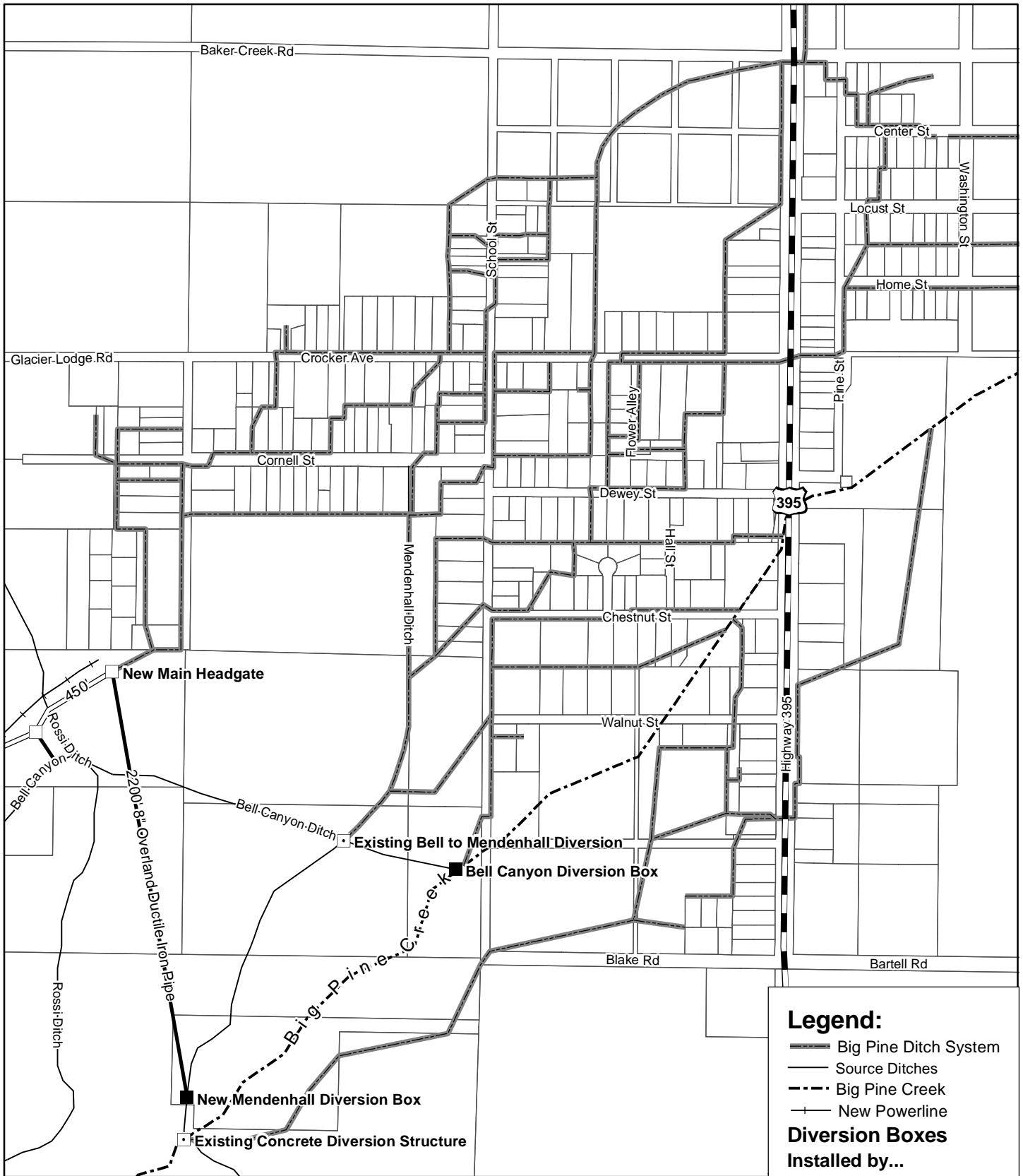
Figure 2. Big Pine Ditch System Delivery Structures
