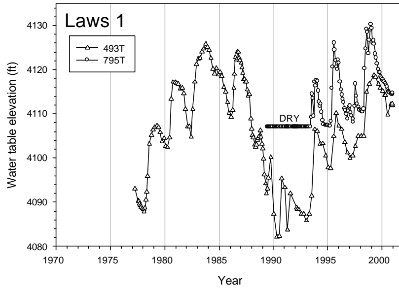
Figure 2. Water table elevation in LW 1 test well (795T) and indicator well 493T.
