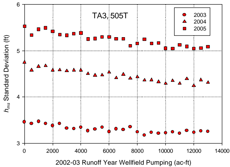
Figure 27. Standard deviation of the predicted h_{ms} at TA3, 505T, for each year as a function of pumping in runoff year 2002-2003.
